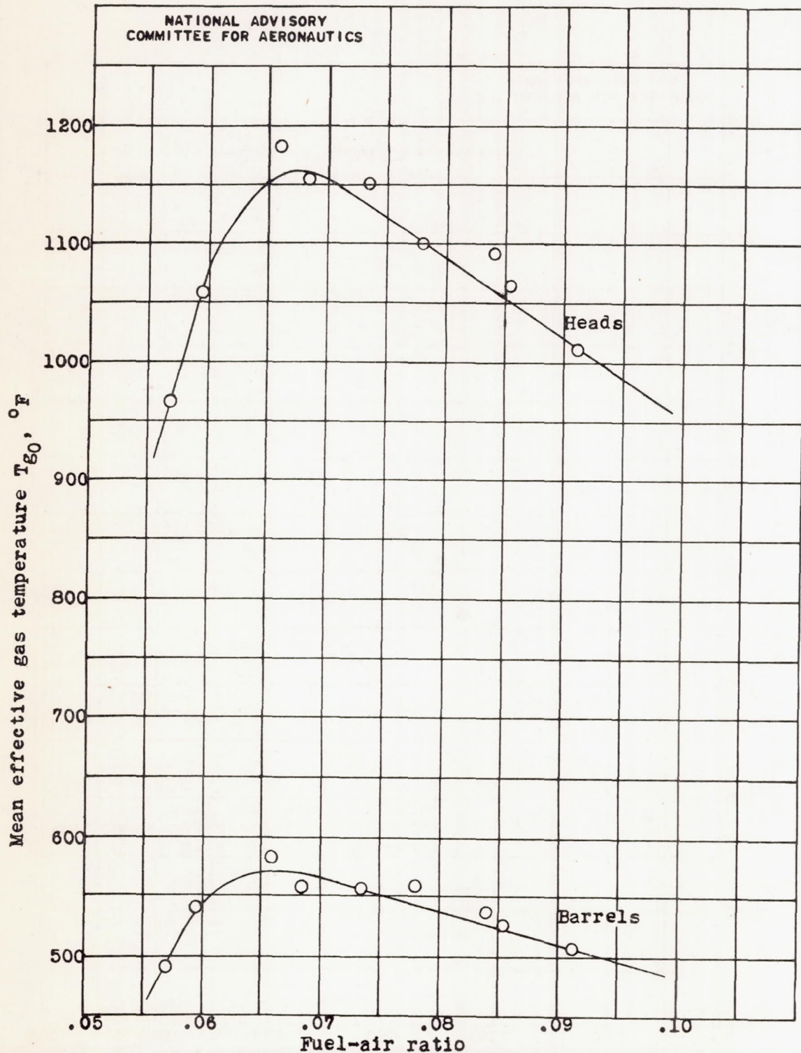
Figure 7. - Variation of mean effective gas temperature T_{g0} with fuel-air ratio. \Delta p , 12 to 14 inches of water; charge-air flow, 5210 to 5360 pounds per hour; low blower ratio; engine speed, 2230 rpm; spark advance, 25° B.T.C.
