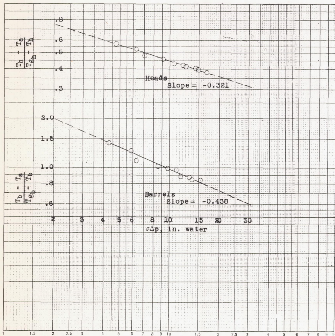
Figure 5. - Variation of \frac{T_h - T_a}{T_{a_h} - T_h} and \frac{T_b - T_a}{T_{a_b} - T_b} with \sigma \Delta p at a pressure
