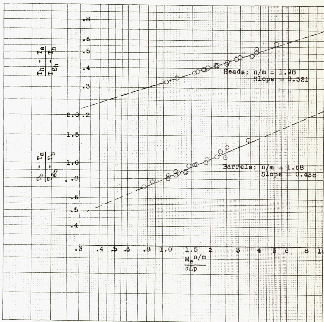
Figure 6. - Cooling-correlation curve at a pressure altitude of 7000 feet. Low blower ratio; engine speed, 2230 rpm; spark advance, 25° B.T.C.
