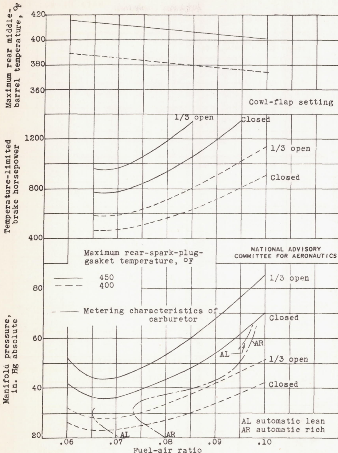
Figure 11. - Predicted temperature-limited manifold pressure, brake horsepower and corresponding maximum rear middle-barrel temperatures for normal flight of four-engine airplane with maximum rear-spark-plug-gasket temperatures of 400° and 450° F. Army summer-air; altitude, 7000 feet; low blower ratio; engine speed, 2230 rpm; spark advance, 25° B.T.C.
