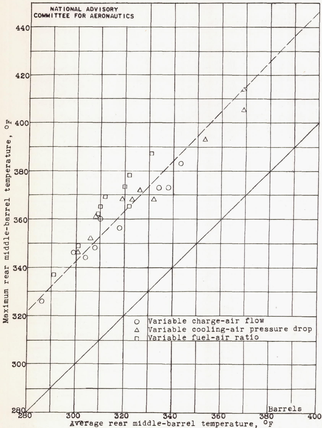
Figure 9. - Deviation of maximum from average rear middle-barrel temperature.
