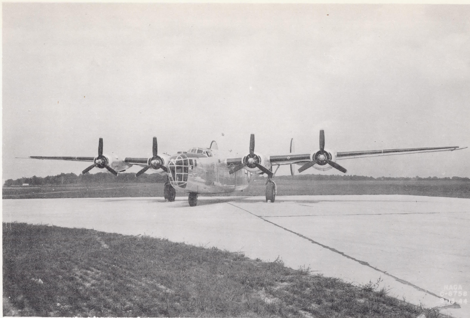
Figure 1. - View of four-engine airplane used for flight knock and cooling investigation.
