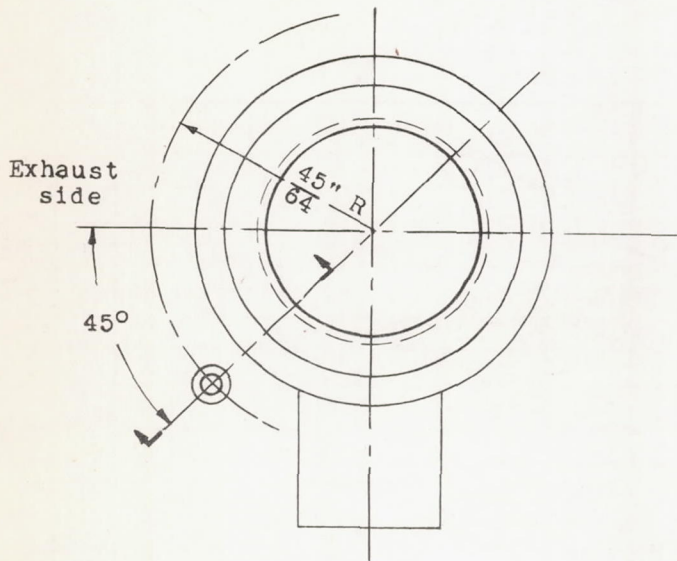
(a) Method of locating thermocouple.
