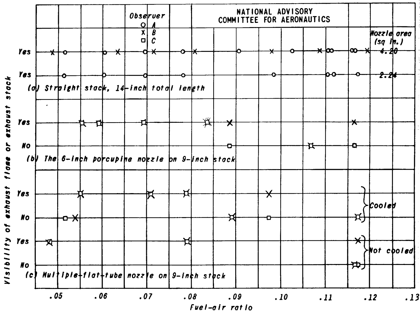
Figure 18. - Visibility of exhaust flame or exhaust stack with miscellaneous nozzles.
