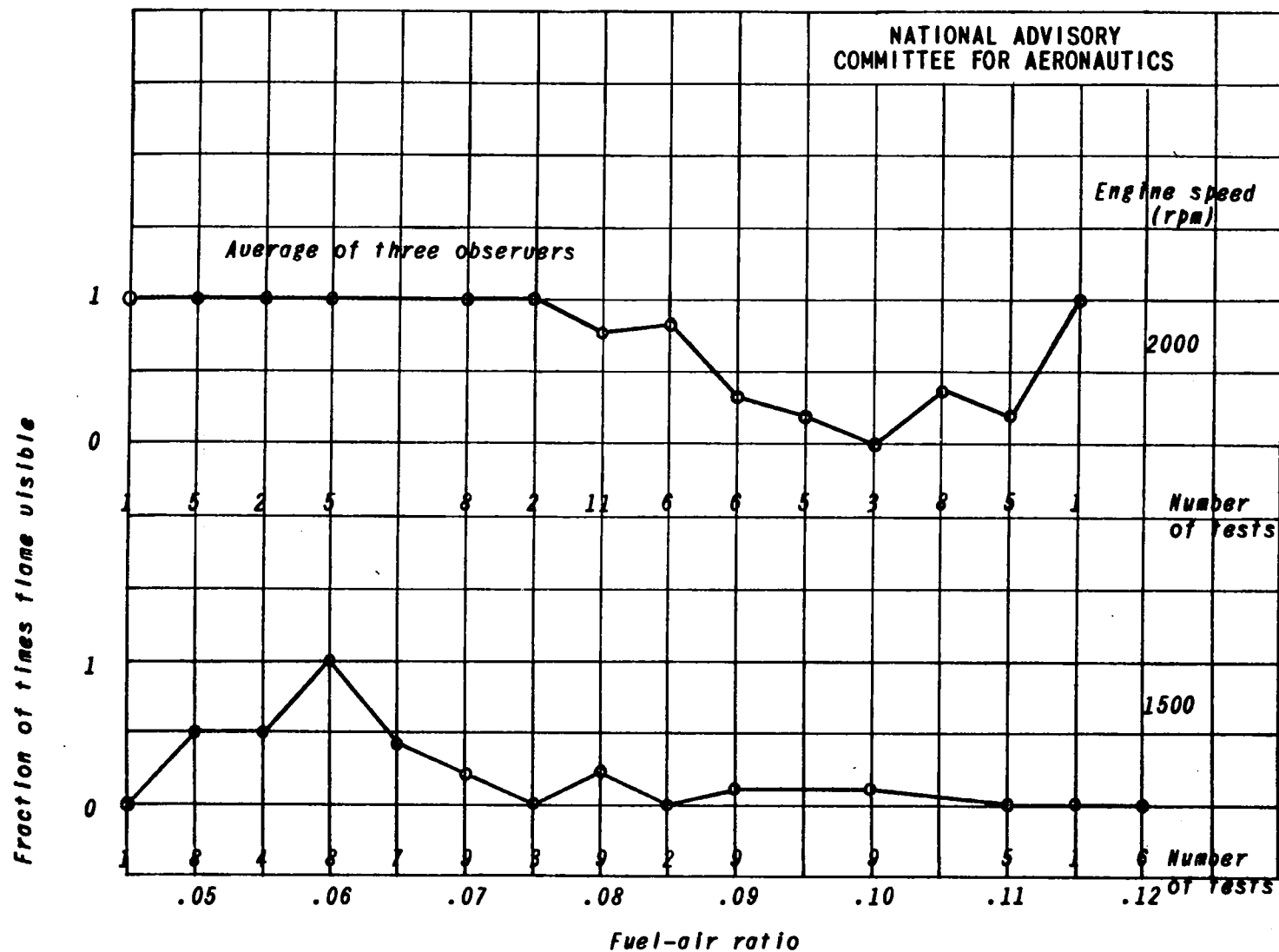
Figure 20. - Visibility of exhaust flame from the four-tube stack, sample A.
