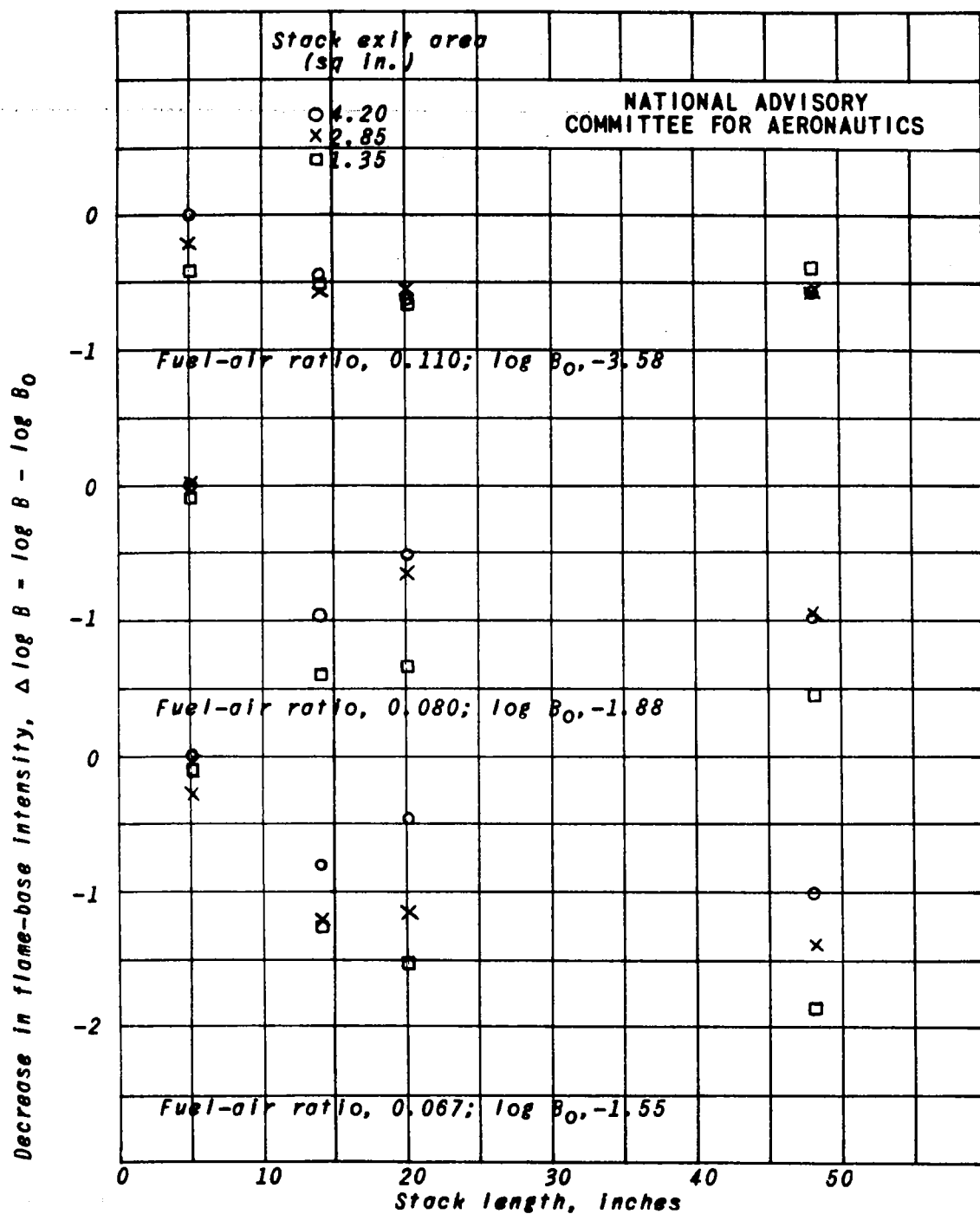
Figure 10. - Effect of stack length on external flame-base intensity. B_0 is the intensity of undamped flame base in millilamberts.
