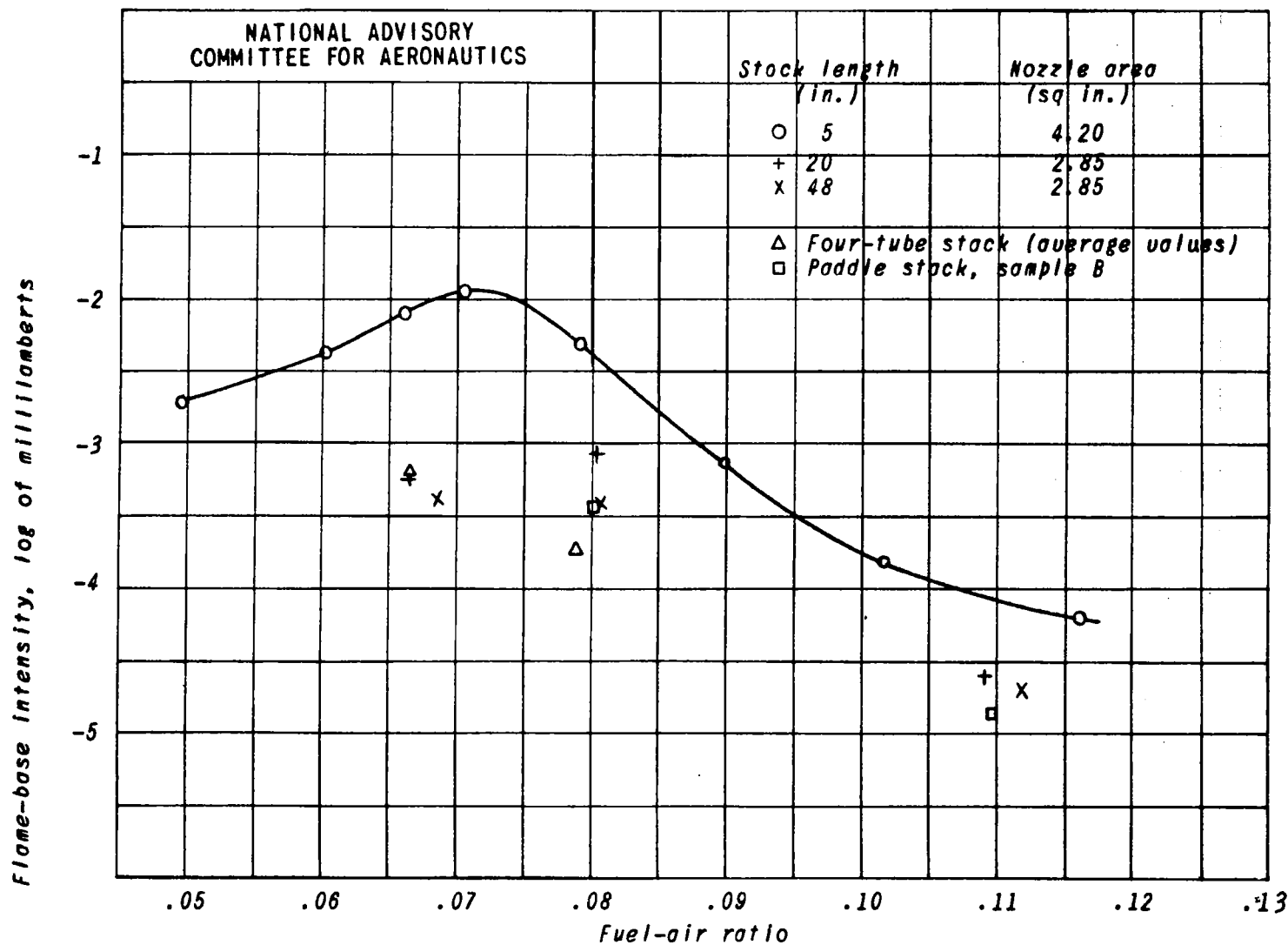
Figure 9. - Intensity of flame base for 5-inch unrestricted stack and other stacks and nozzles. Intake-manifold pressure, 30 inches Hg absolute; engine speed, 1500 rpm.
