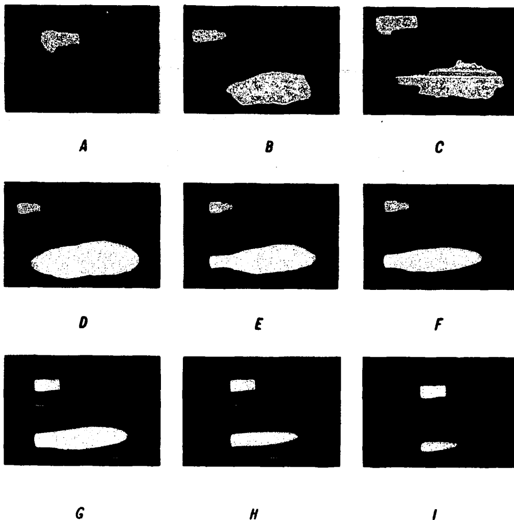
Figure 6. - Undamped flame of the 1820-G engine. Fuel, leaded; fuel-air ratio, variable; hydrogen-carbon ratio, 0.189.
