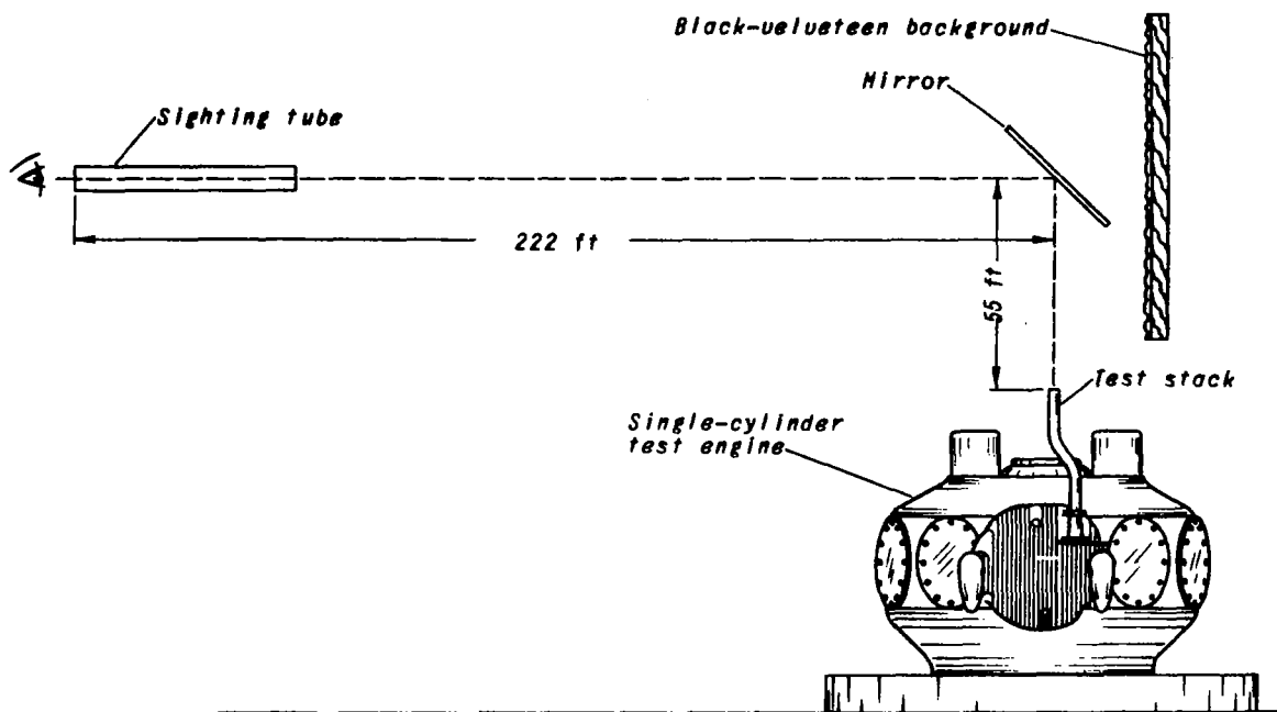
Figure 3. - Visibility-test setup.
