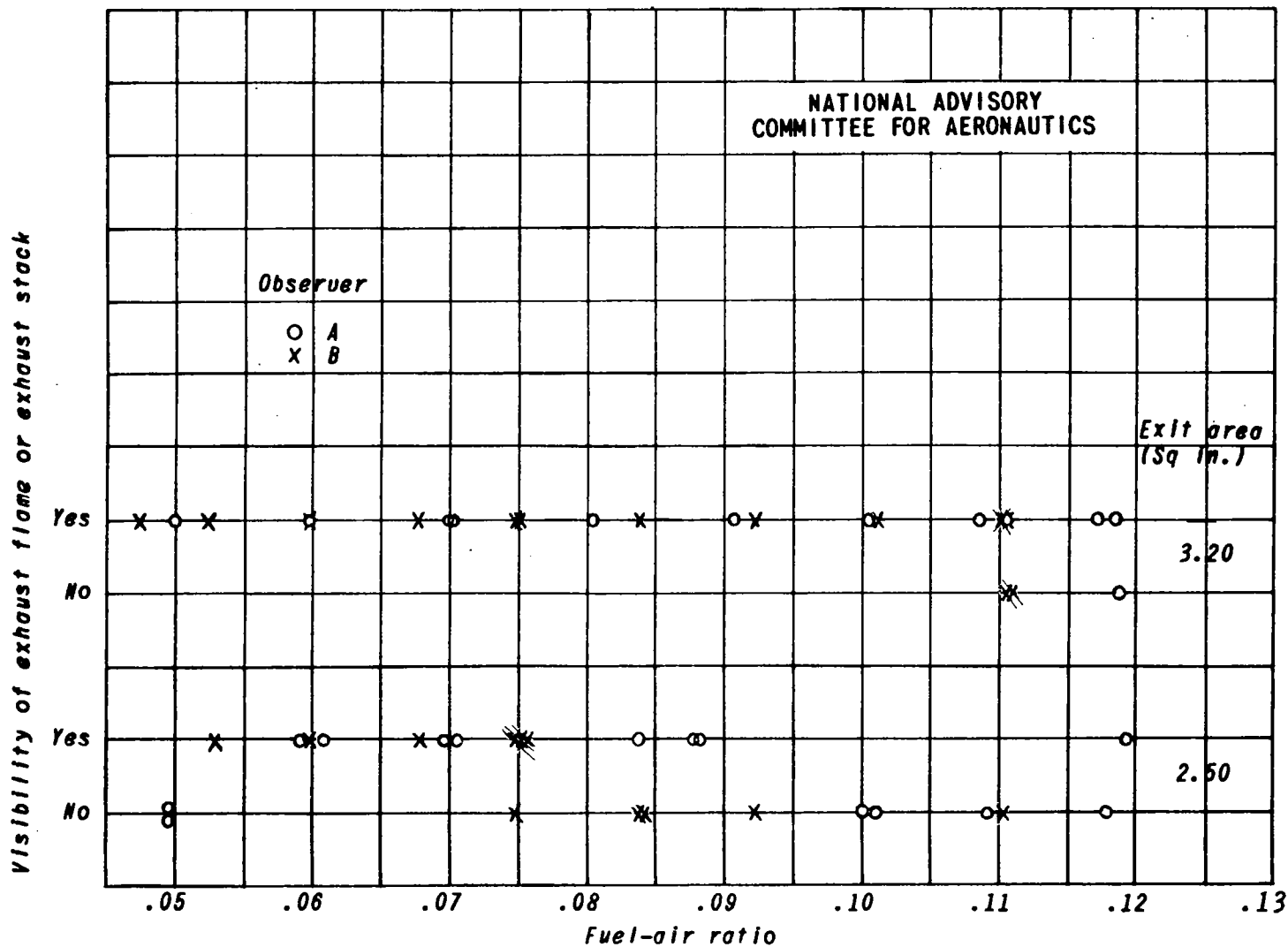
Figure 19. - Visibility of exhaust flames from paddle-type stacks, samples B and C.
