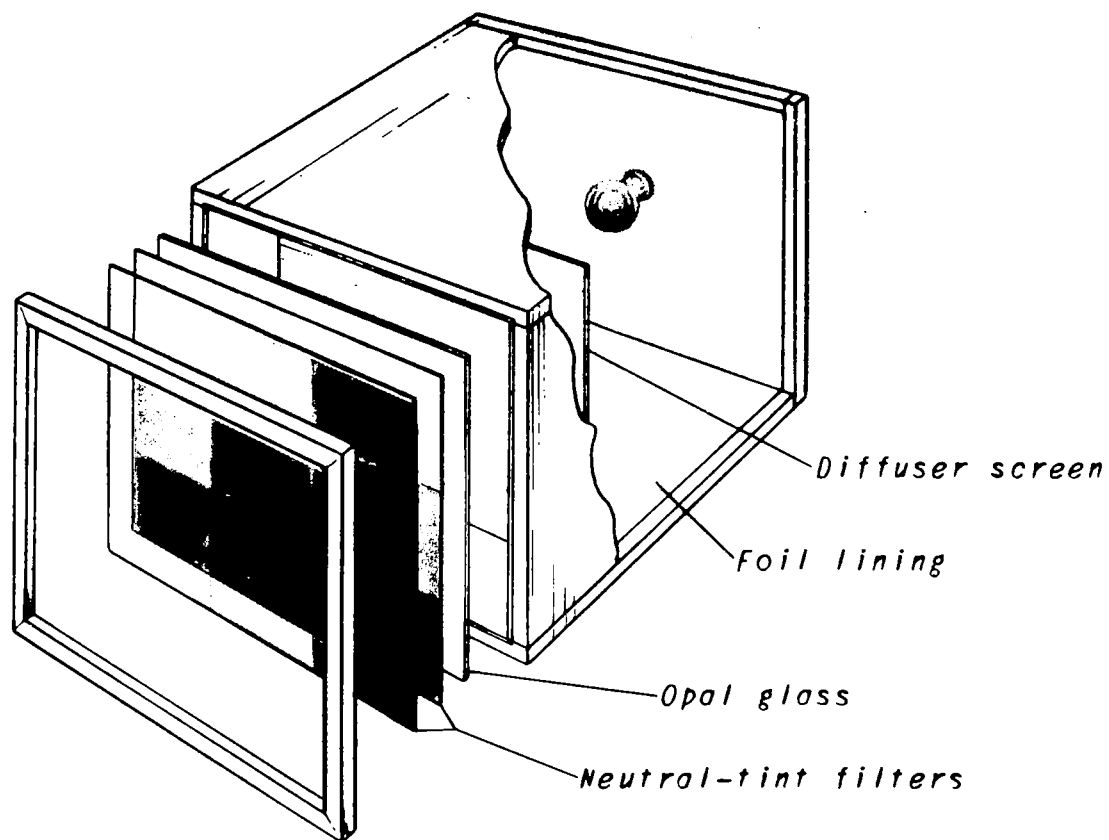
Figure 1. - Construction of comparison light source.
