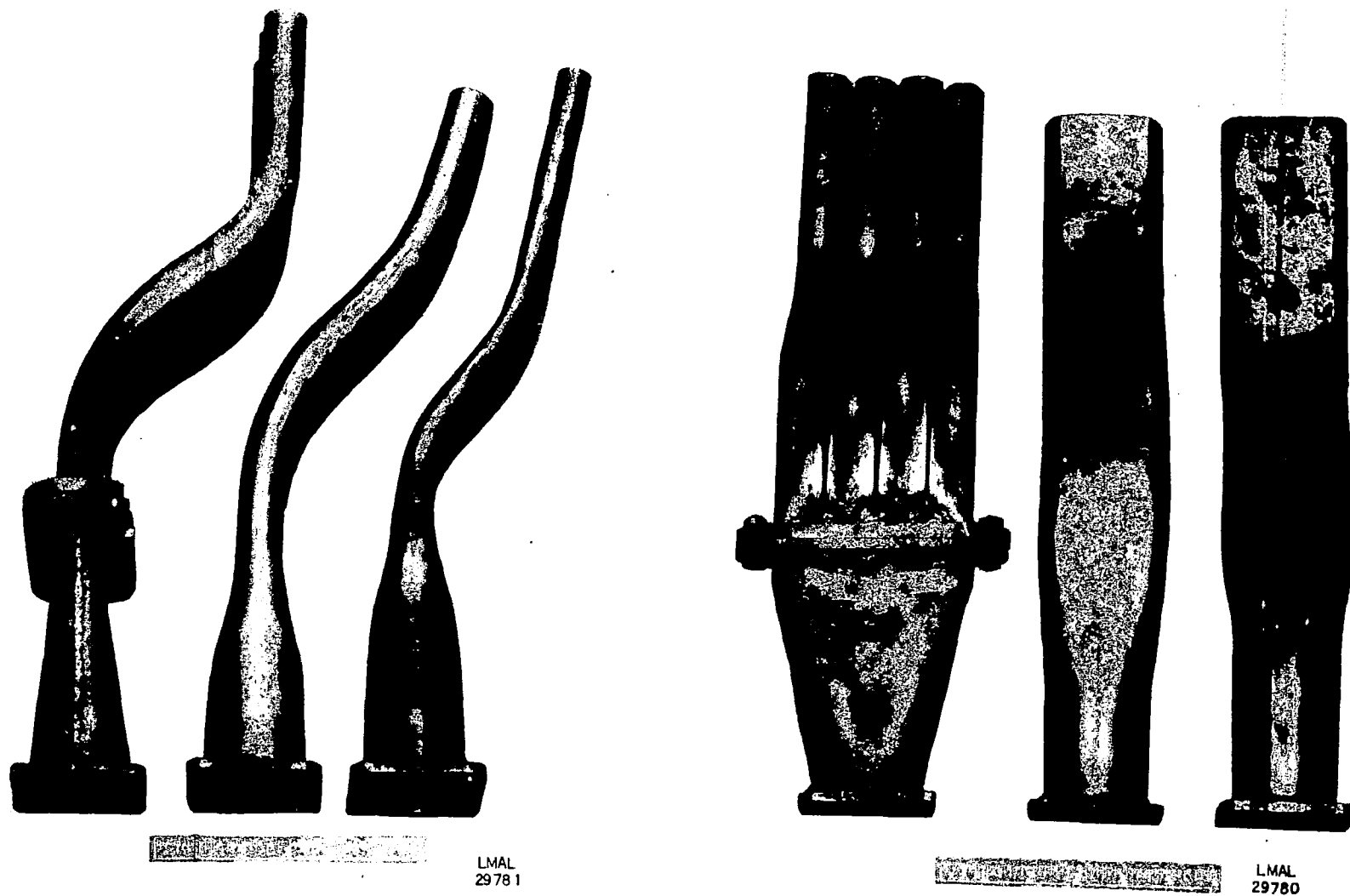
Figure 16. - Sample flame-damping stacks A, B, and C.
