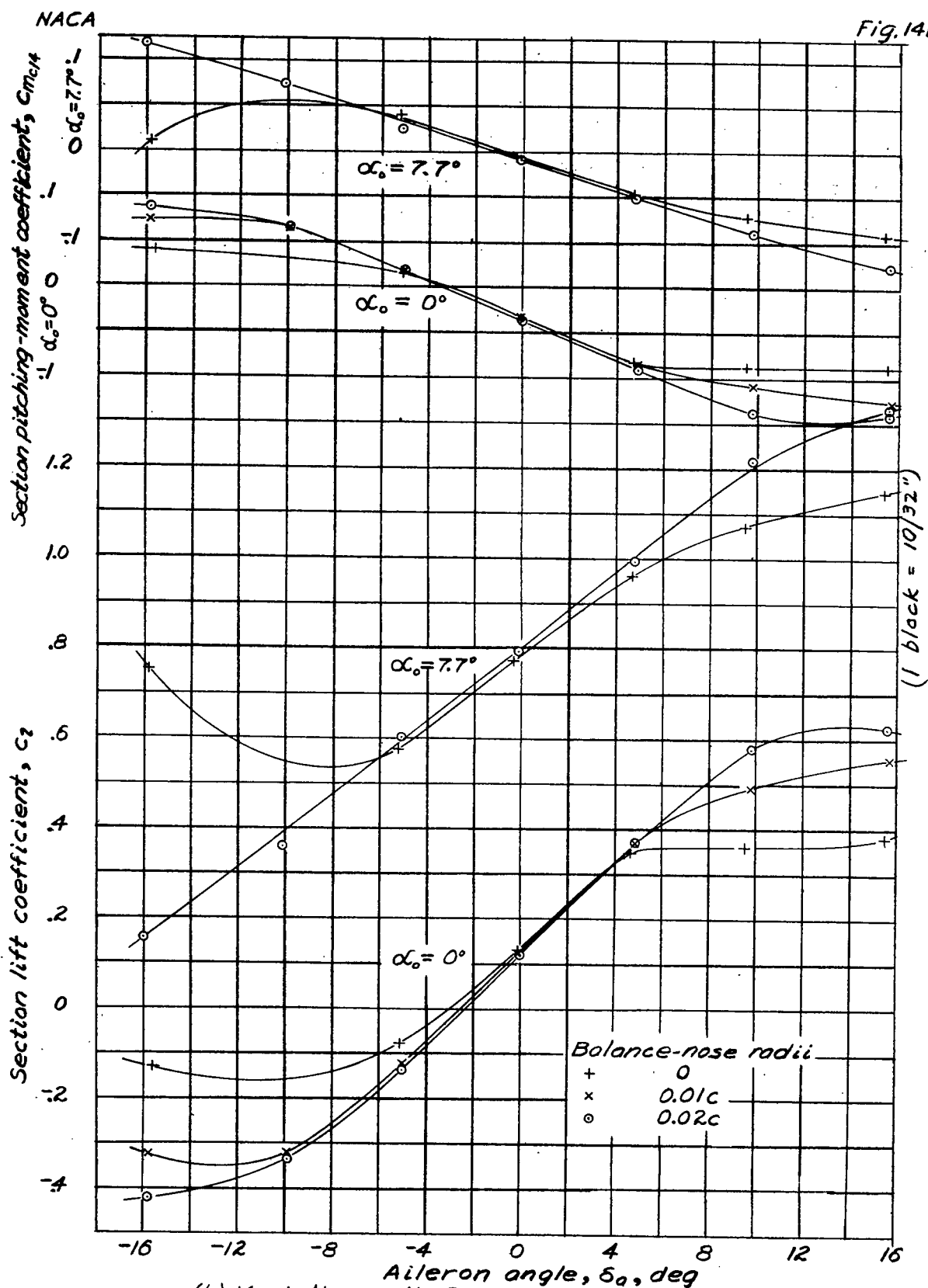
(b) Variation with \delta_a . Figure 14. — Section lift coefficients and section pitching-moment coefficients obtained by pressure-distribution. M=0.358 ; gap = 0.0055c. (Concluded).
