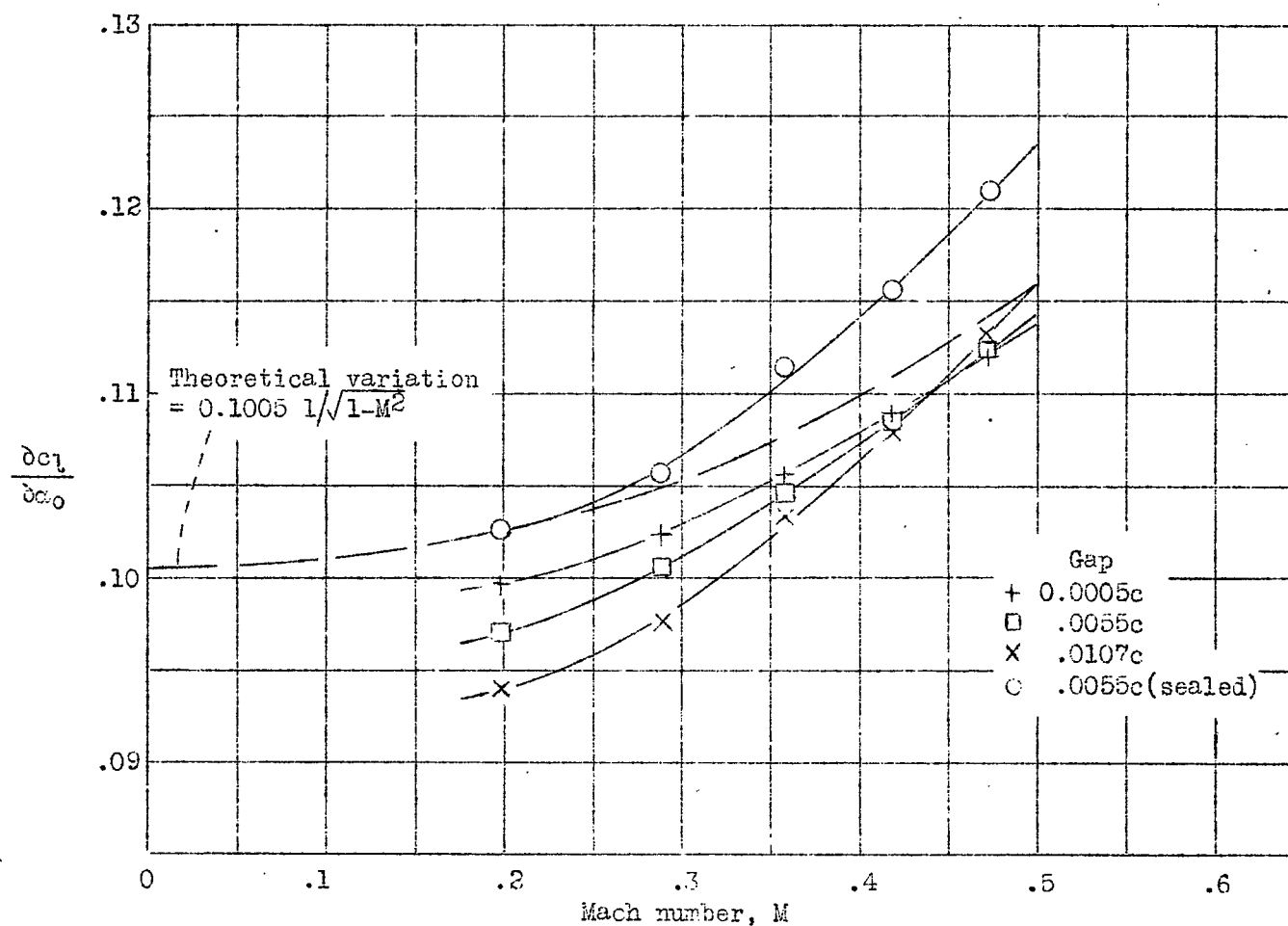
Figure 12.- Variation of lift curve slope \delta c_l / \delta \alpha with Mach number for various gap widths. \delta_a = 0 .
