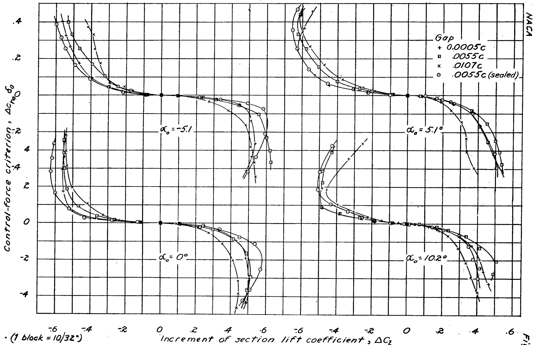
Figure 19. -- Variation of control-force criterion with increment of section lift coefficient, showing effect of gap. Balance-nose radii = 0.020c; M = 0.417 .
