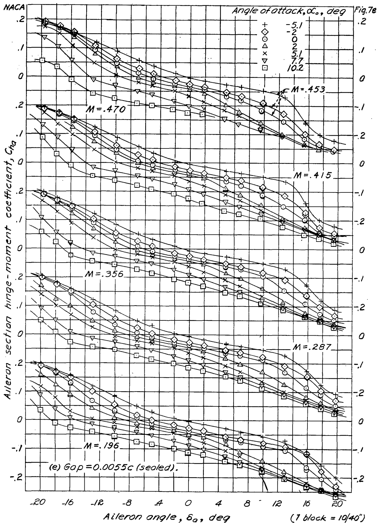
Figure 7.—Variation of aileron section hinge-moment coefficient with aileron angle. Balance-nose radii = 0.02c. (Concluded)
