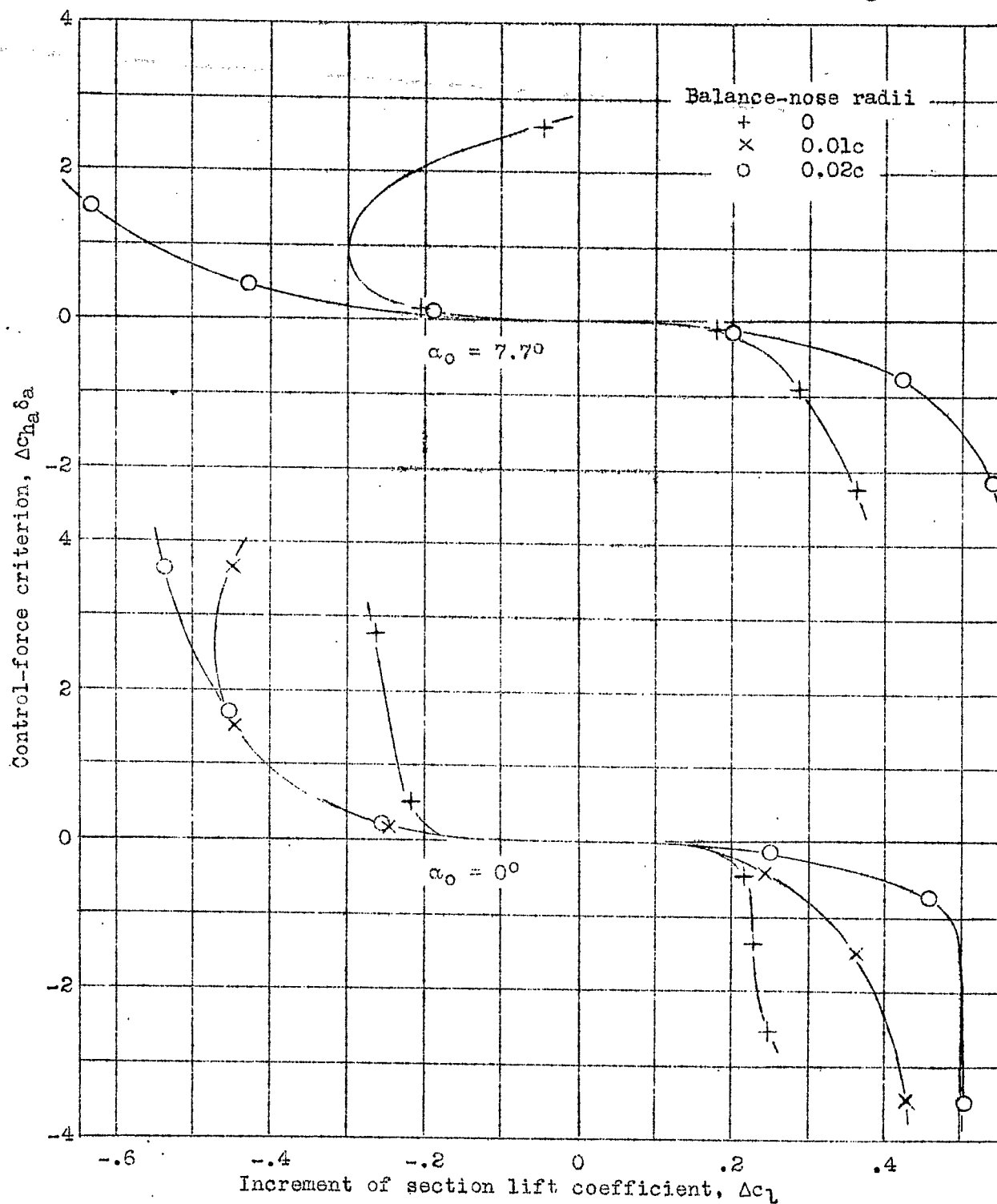
Figure 18.- Variation of \Delta c_{ha} \delta a with \Delta c_l (by pressure distribution) showing effect of balance-nose radii. M = 0.358 ; gap = .00055c.
