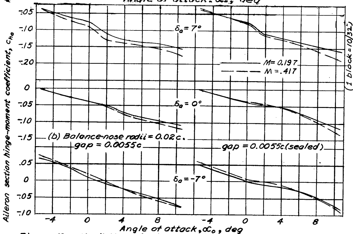
Figure 10. — Variation of aileron section hinge-moment coefficient with angle of attack.
