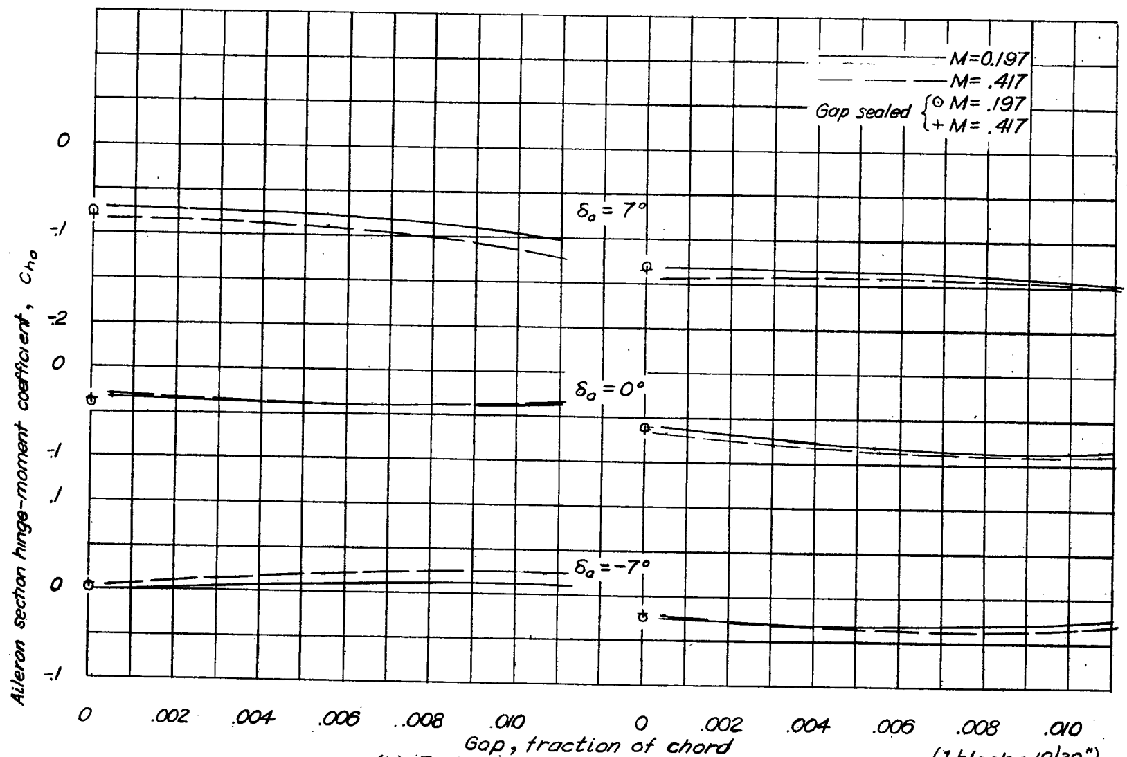
(b) Balance-nose radii = 0.02c. \alpha_o = 0^\circ \alpha_o = 5.1^\circ Figure 9.— Variation of aileron section hinge-moment coefficient with gap: (Continued)
