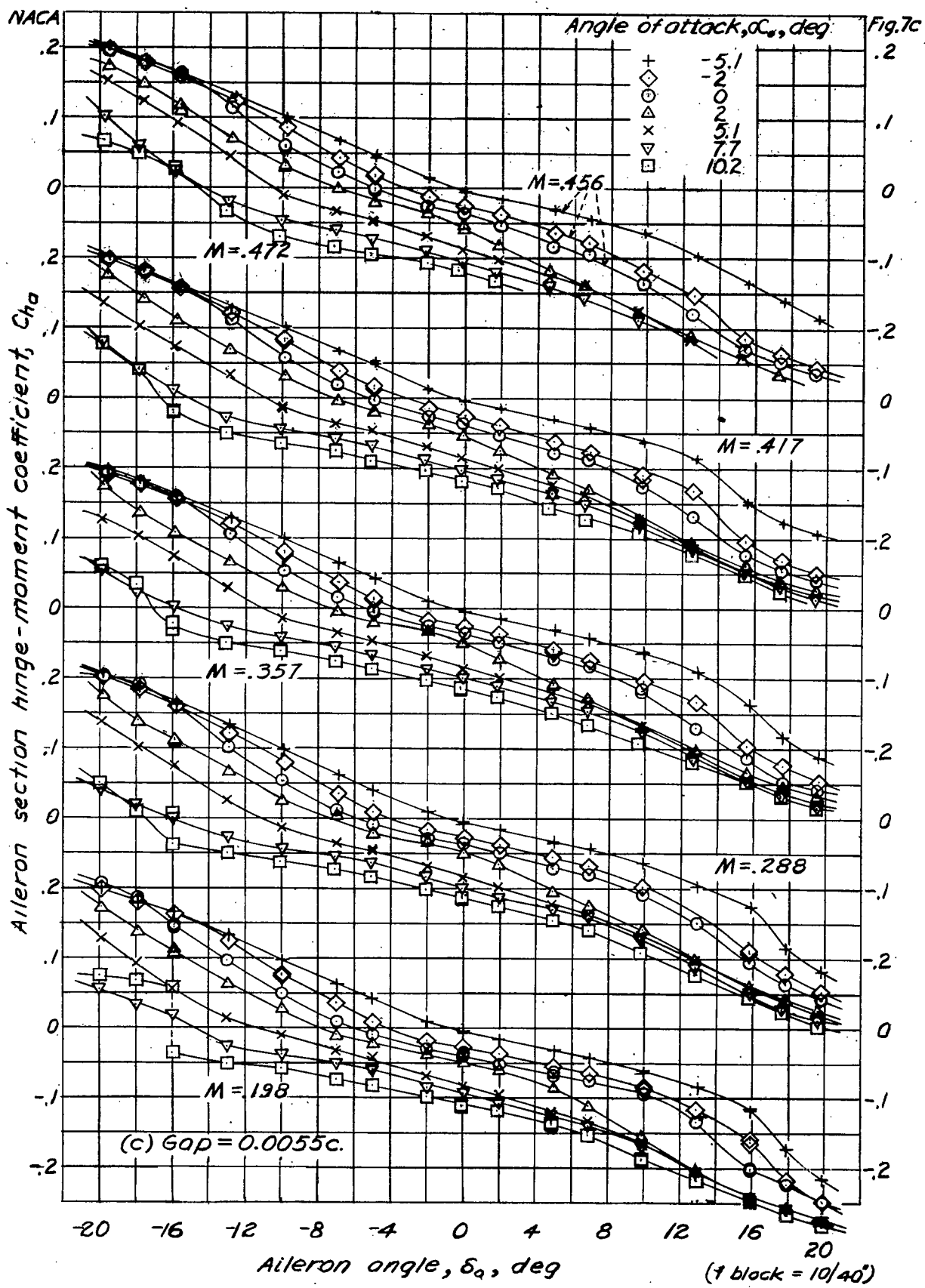
Figure 7. — Variation of aileron section hinge-moment coefficient with aileron angle. Balance-nose radii = 0.02c. (Continued)
