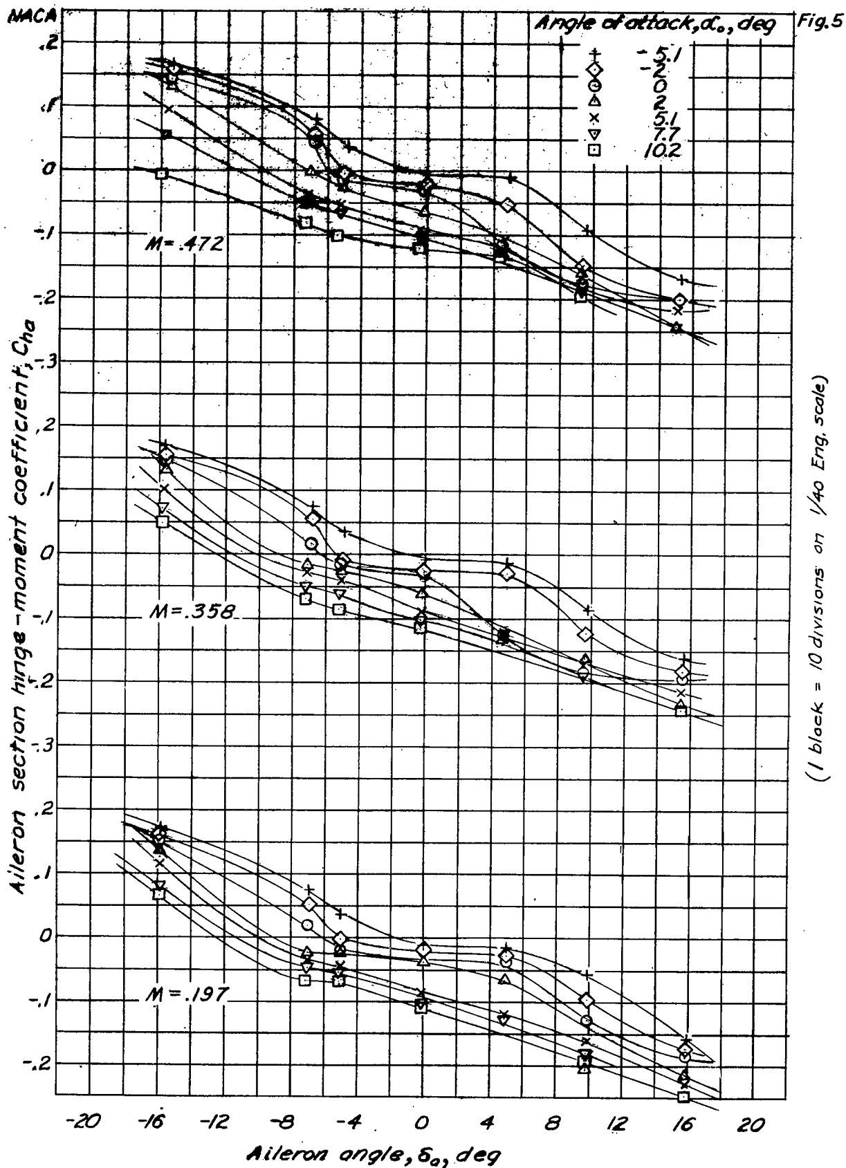
Figure 5.—Variation of aileron section hinge-moment coefficient with aileron angle (by pressure distribution). Balance-rose radii = 0; gap = 0.0055 c.
