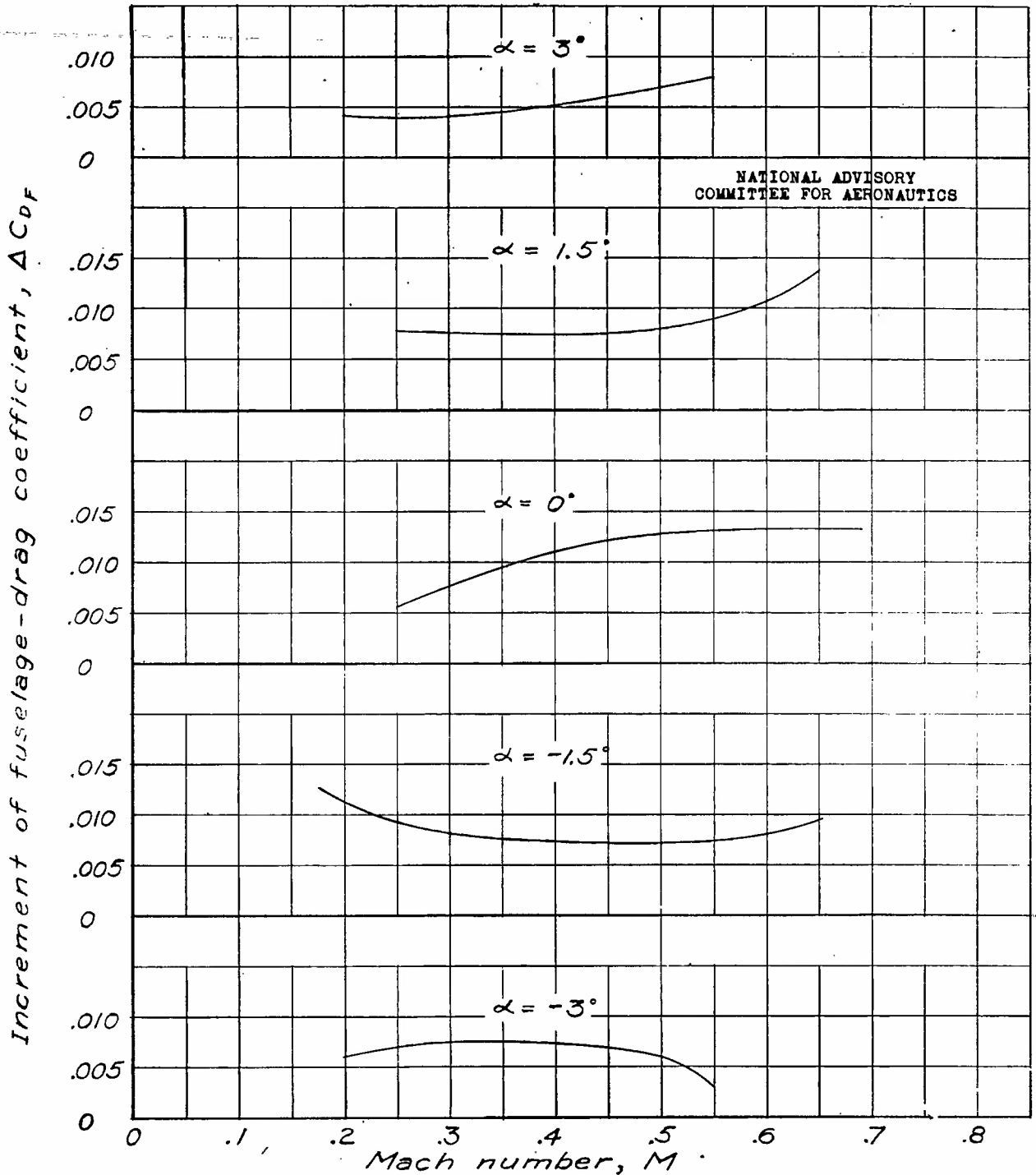
Figure 7.-Increment of fuselage-drag coefficient, \Delta C_{df} , based on maximum fuselage cross-sectional area due to eight gun openings in the nose of the fuselage of a 1/4-scale model airplane. Fixed transition 15 inches from nose.
