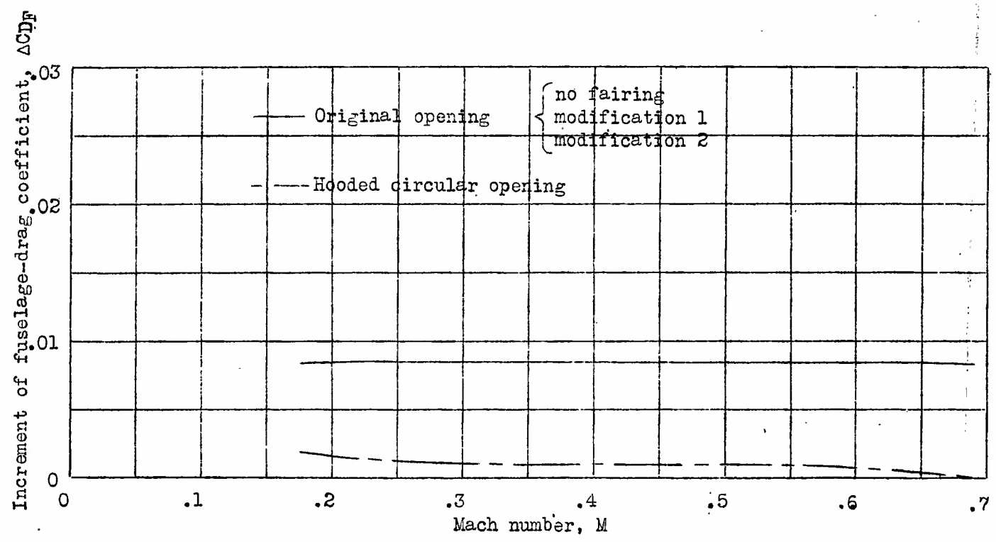
Figure 4.- Increment of fuselage-drag coefficient, \Delta C_{Df} , based on maximum fuselage cross-sectional area due to an outboard .50-caliber machine-gun opening in the nose of the fuselage of a 1/4-scale model airplane. Natural transition; \alpha = 0^\circ .
