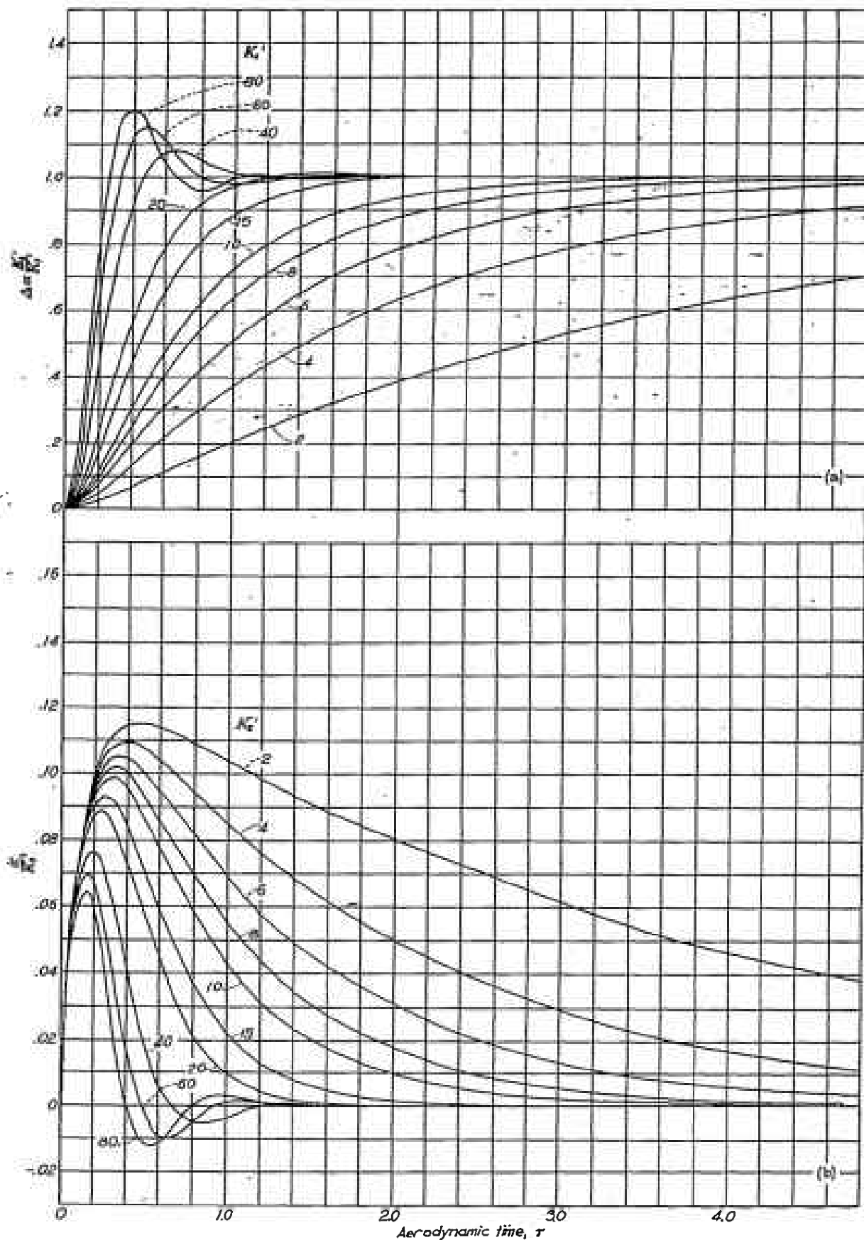
FIGURE 5.—Variation of \Delta\alpha \frac{K'}{K} and \frac{d}{K'} with aerodynamic time for an instantaneous elevator deflection. K' = 8.0 .
