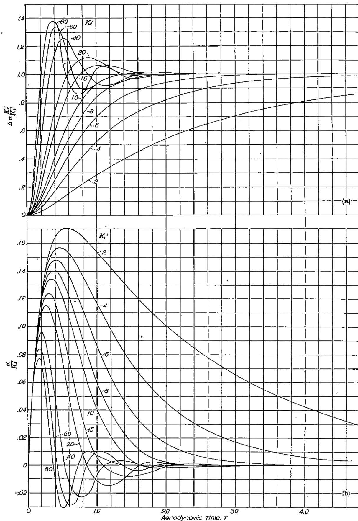
FIGURE 2—Variation of \Delta \alpha \frac{K'_t}{K'_f} and \frac{d}{K'_f} with aerodynamic time for an instantaneous elevator deflection. K'_f = 5.0 .
