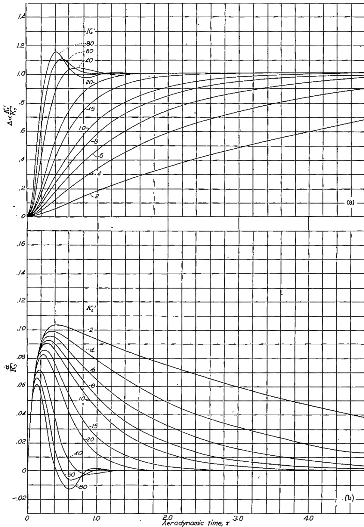
FIGURE 6.—Variation of \Delta\alpha \frac{K'_H}{K'_Y} and \delta \frac{K'_Y}{K'_Y} with aerodynamic time for an instantaneous elevator deflection. K'_Y = 0.0 .
