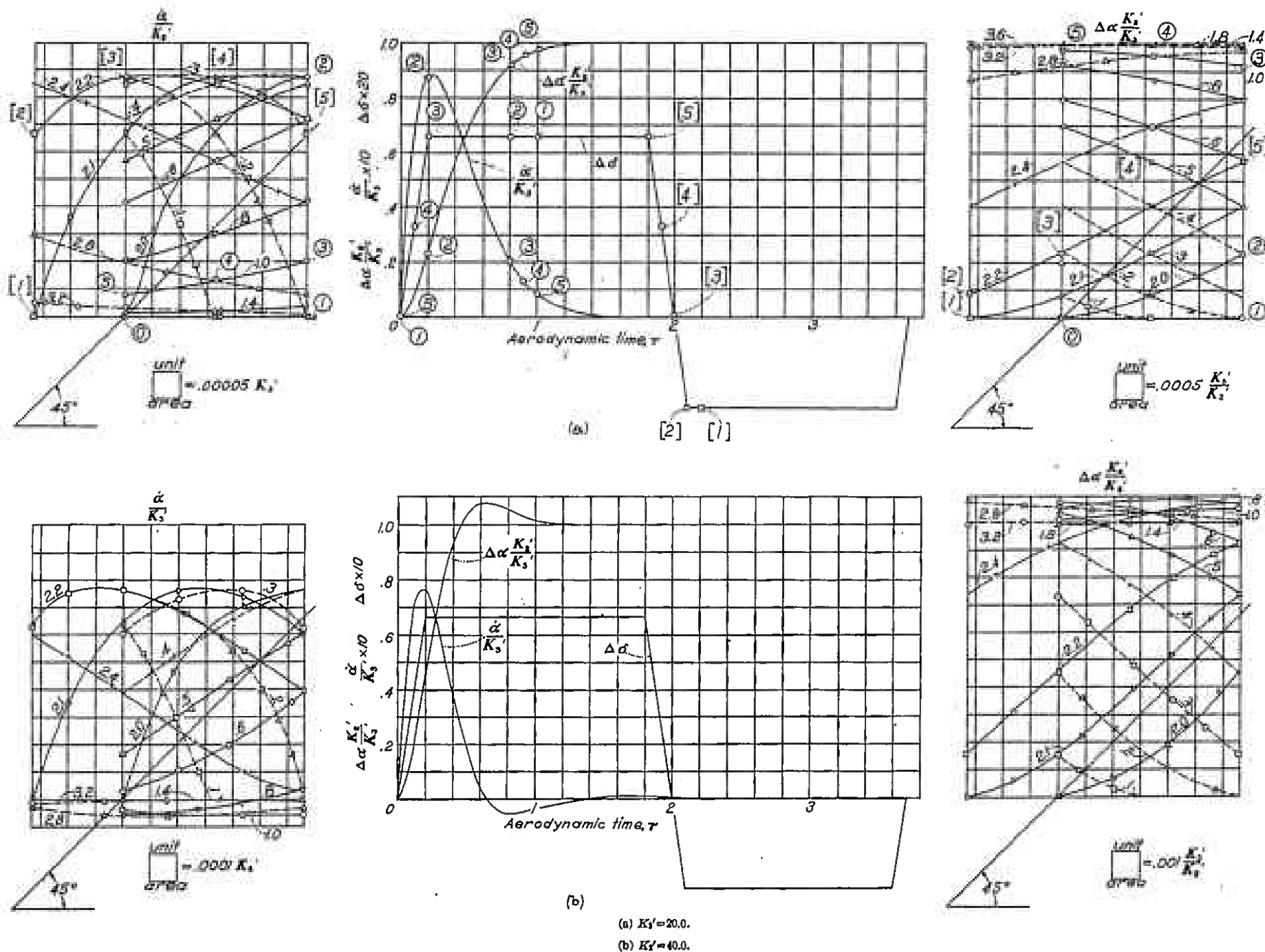
FIGURE 7.—Determination of \Delta\alpha and \dot{\alpha} for the elevator motion suggested in reference 1. K_1' = 3.0 ; K_2' = -100.0 .
