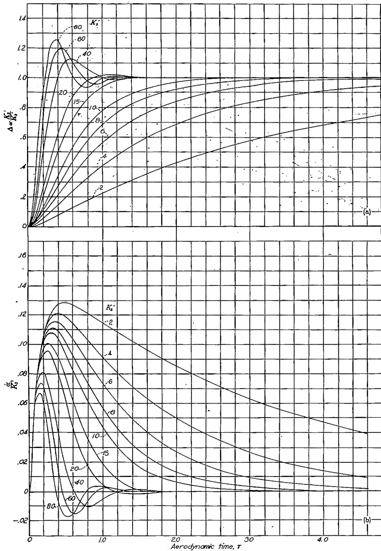
FIGURE 4.—Variation of \Delta \alpha \frac{K_1'}{K_2'} and \ddot{\alpha} \frac{K_1'}{K_2'} with aerodynamic time for an instantaneous elevator deflection. K_1' = 7.0 .
