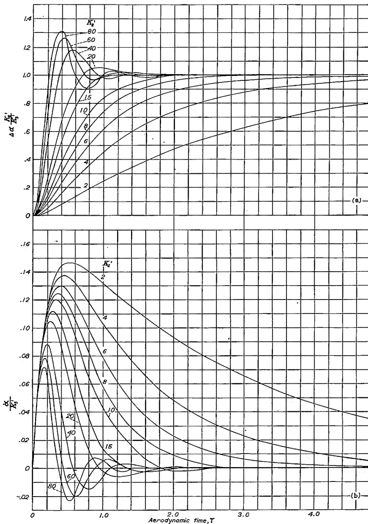
FIGURE 3.—Variation of \Delta \alpha \frac{K_3'}{K_3} and \frac{\alpha}{K_3} with aerodynamic time for an instantaneous elevator deflection. K_1' = 6.0 .
