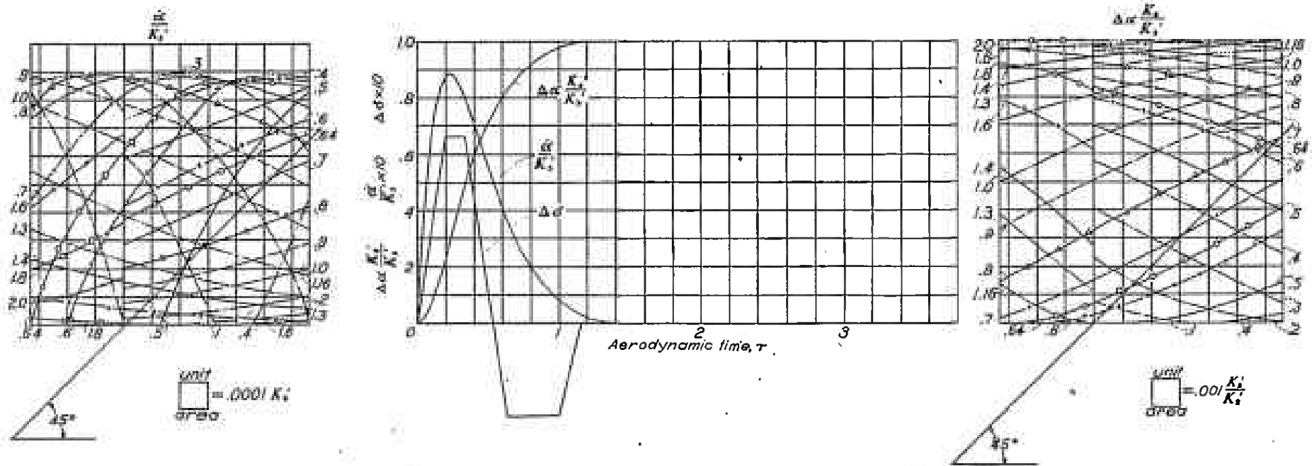
FIGURE 9.—Determination of \Delta\alpha and \Delta\delta for rapid reversal of elevator. K_1=8.0 ; K_2=20.0 ; K_3=-100.0 .
