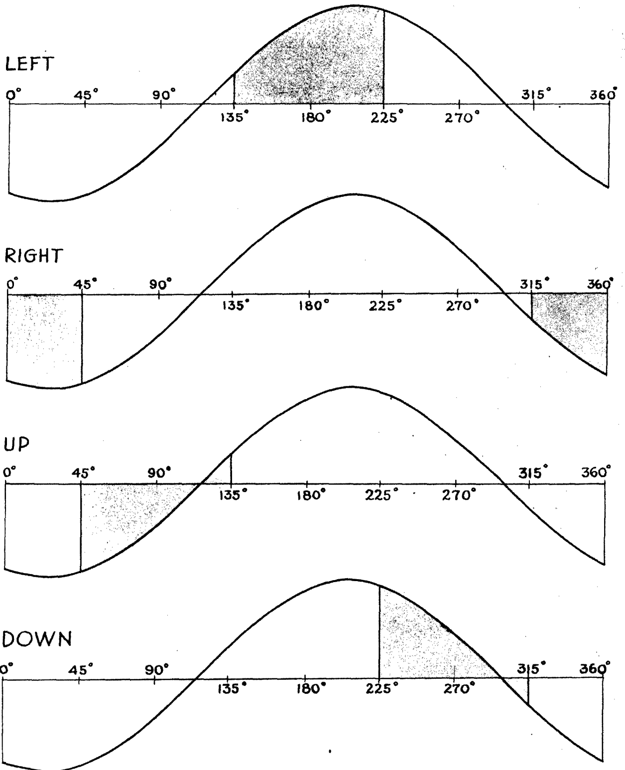
Figure 7 — Commutation of Scanned Signals
