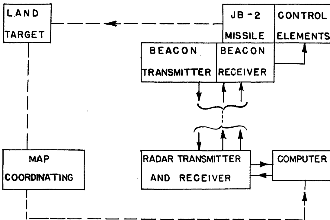
Figure 2 — The Guided Buzz-Bomb (JB-2)
