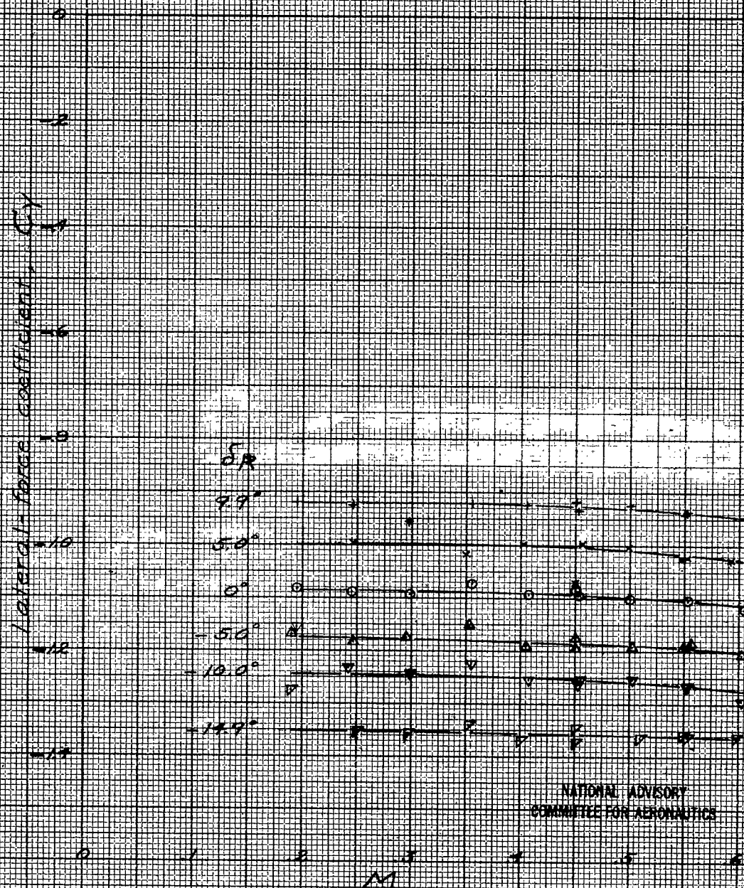
Figure 13. Variation of lateral force coefficient with Mach number for several rudder angles \gamma = -15.5^\circ
