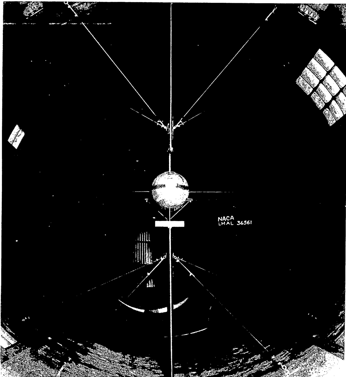
Figure 4.- Setup employed for determining support-strut tares.
