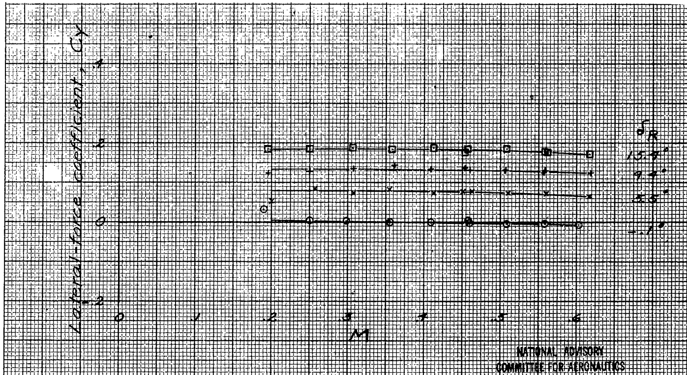
Figure 15-Variation of lateral-force coefficient with Mach number for several rudder angles \psi = -1.5^\circ ; antenna struts removed
