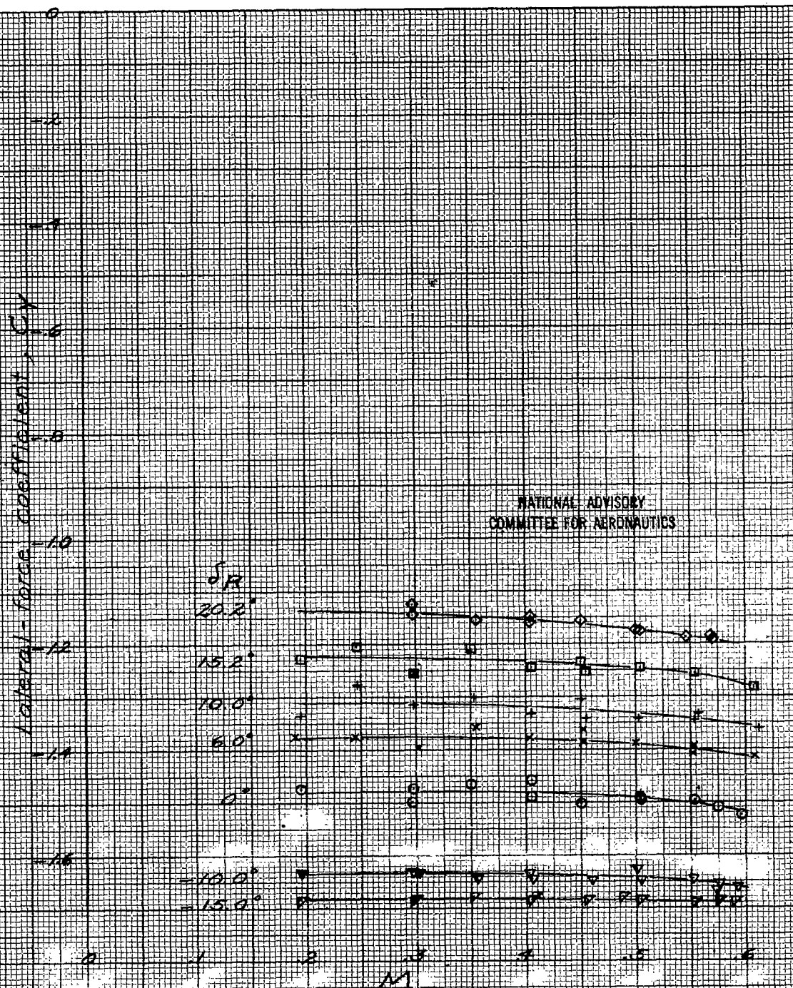
Figure 14- Variation of lateral-force coefficient with Mach number for several rudder angles \eta = -20.5^\circ
