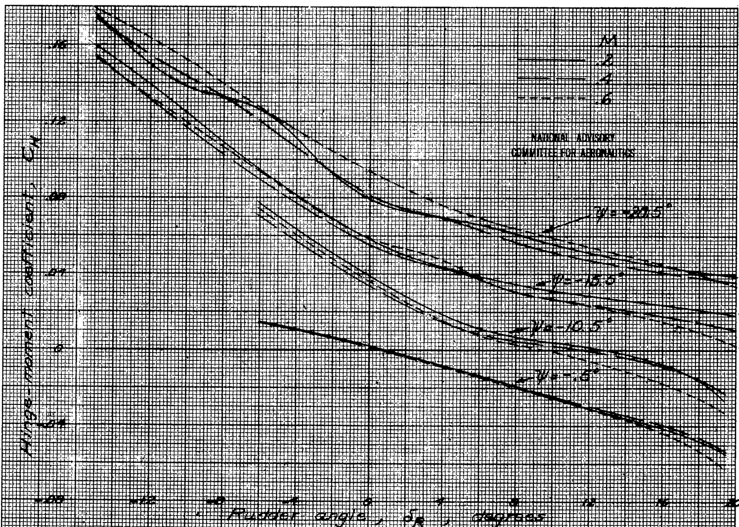
Figure 26.- Variation of rudder hinge-moment coefficient with rudder angle for several angles of sideslip and Mach numbers
