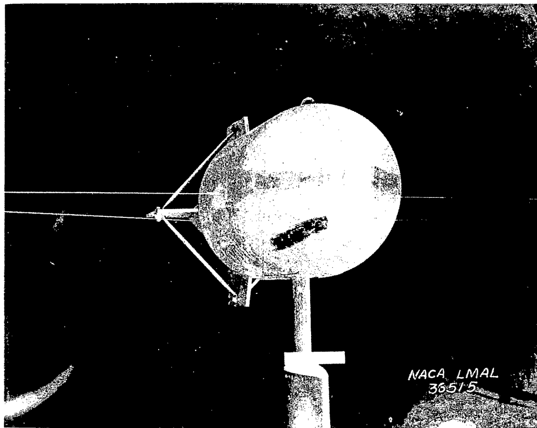
Figure 3.- AN-M-65-AZON 1000-pound bomb installed in the 16-foot high-speed tunnel.
