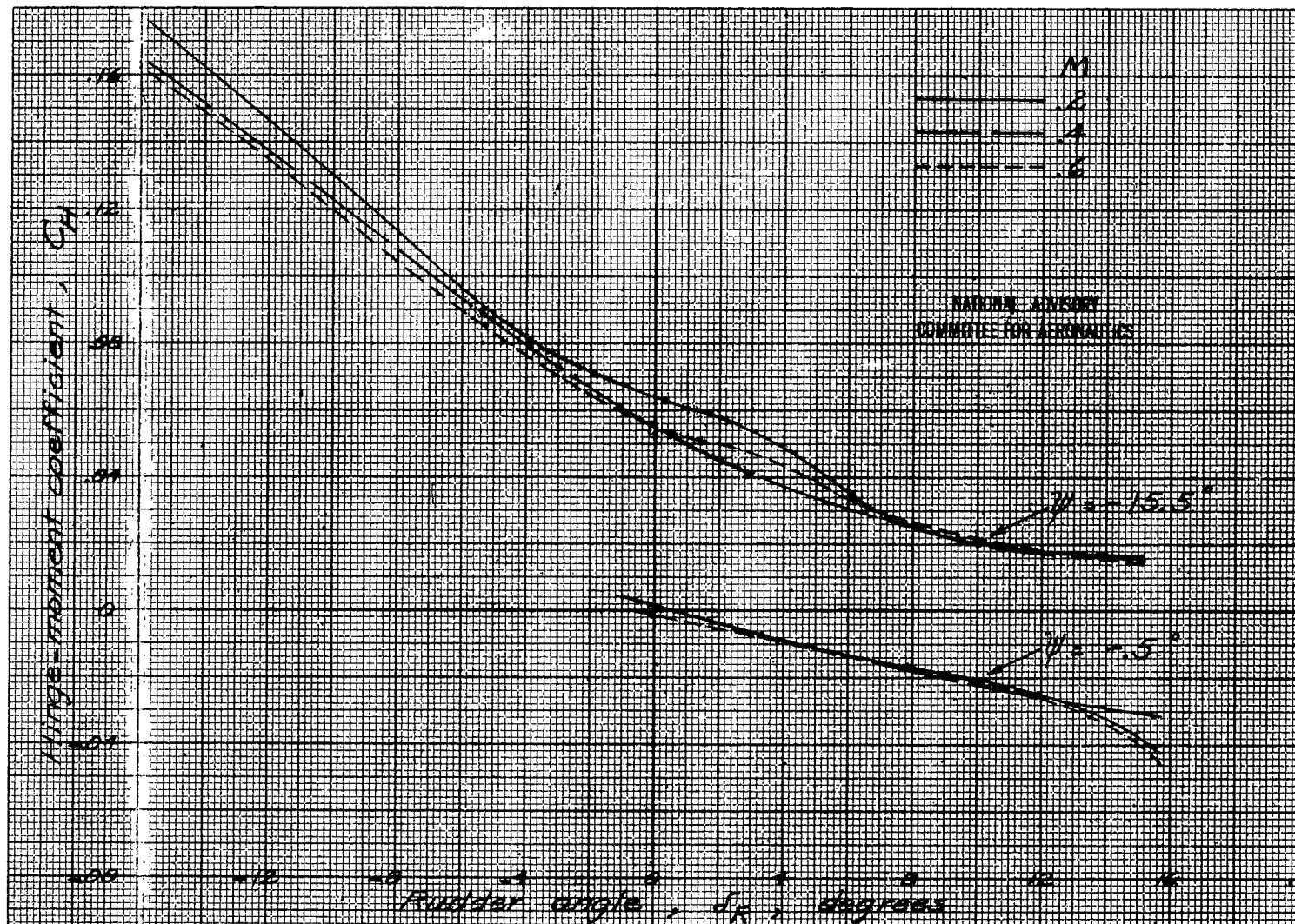
Figure 31.- Variation of rudder hinge-moment coefficient with rudder angle; antenna struts removed
