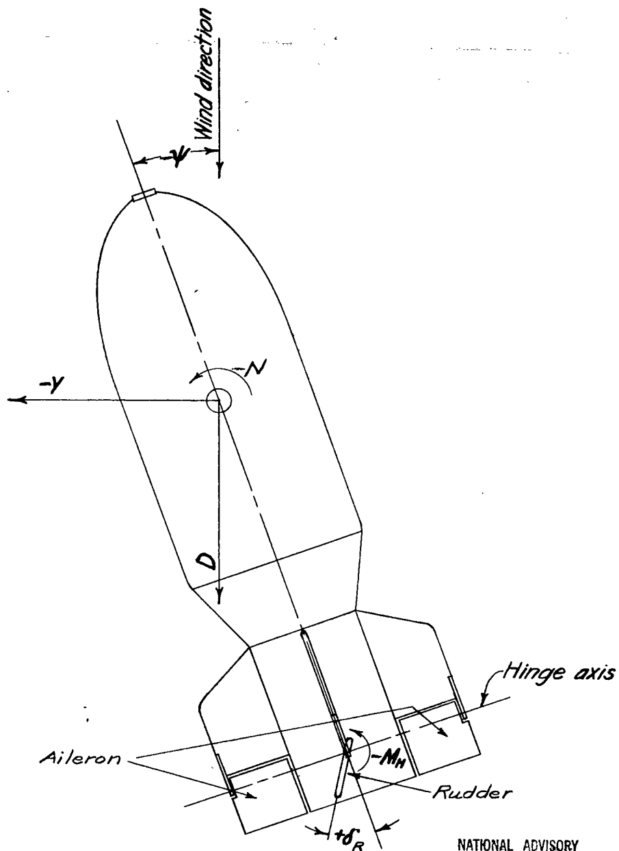
Figure 1.—Sketch showing sign conventions for angles, forces, and moments.
