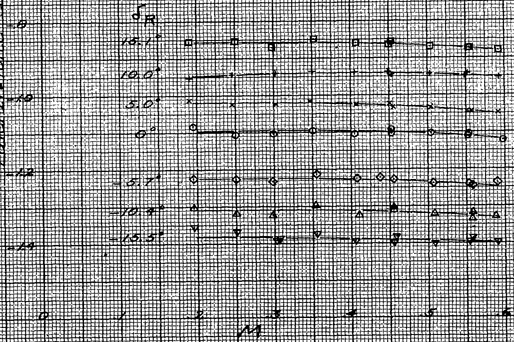
Figure 16. Variation of lateral-force coefficient with Mach number for several rudder angles \delta_R = -15.5^\circ ; antenna struts removed
