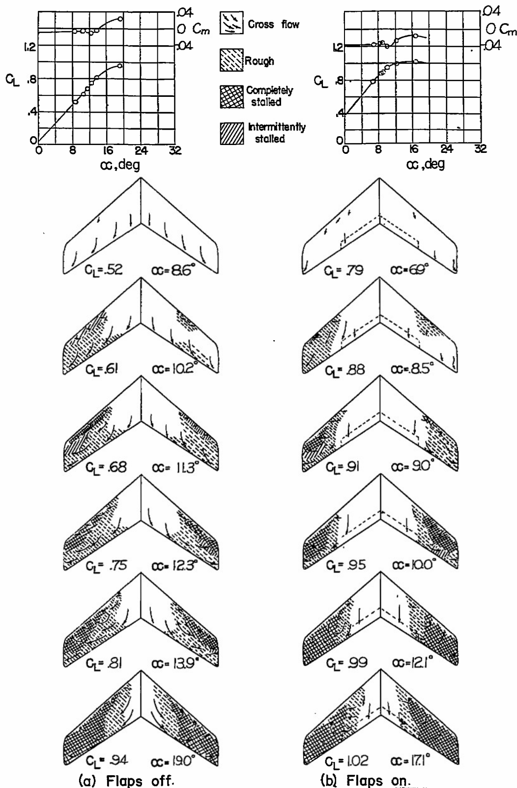
Figure 9.— Stalling characteristics of 42^\circ swept-back wing with leading edge roughness. R=6,800,000 .
