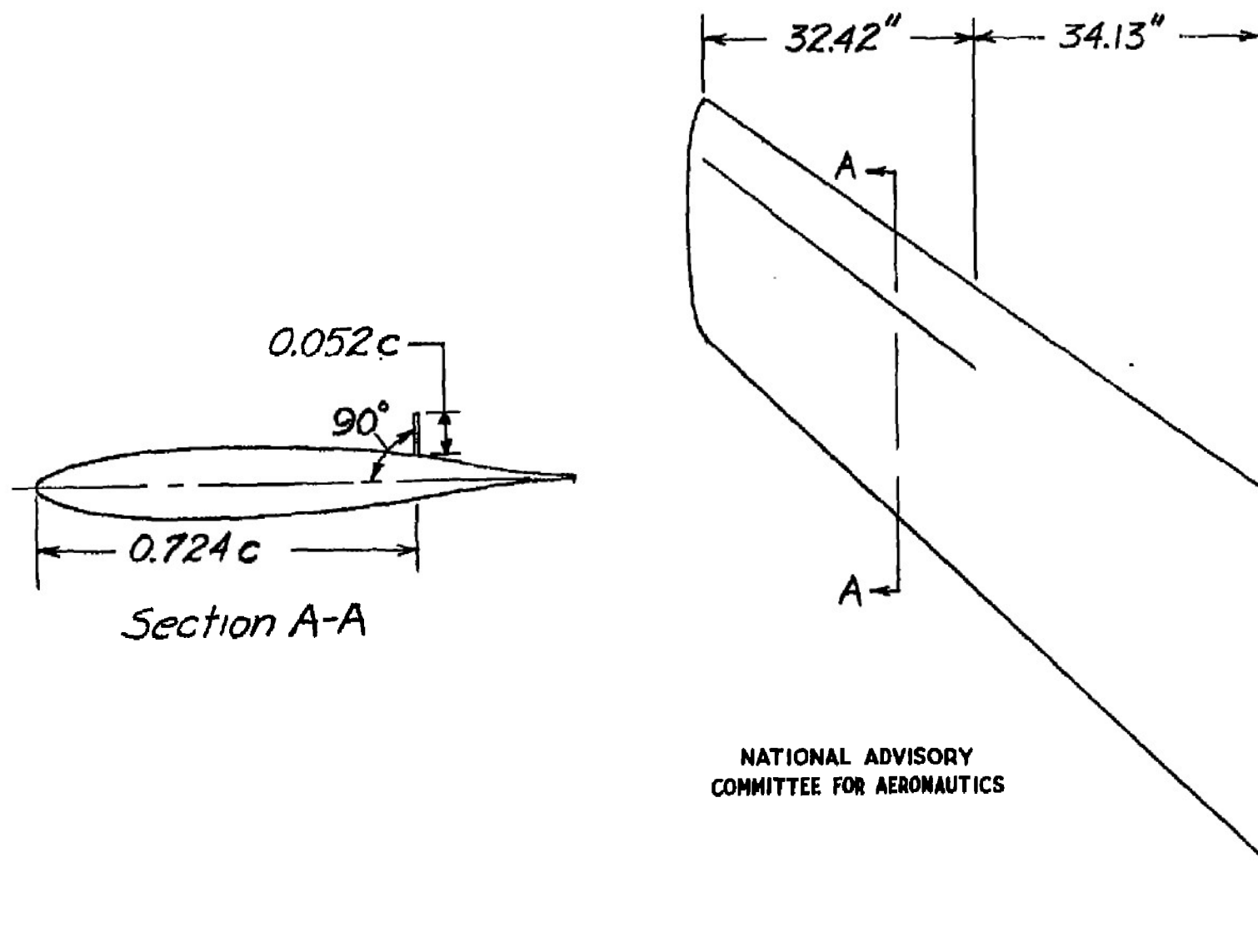
Figure 3.- Spoiler installation.
