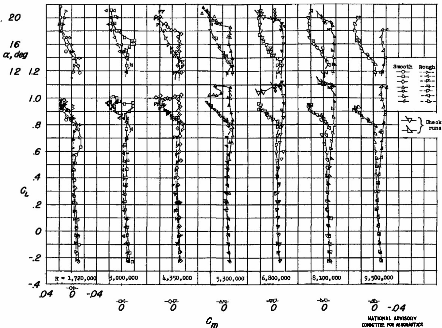
Figure 10.- Pitching-moment characteristics for various values of Reynolds number, 42^\circ swept-back wing with and without leading-edge roughness; \gamma = 0^\circ
