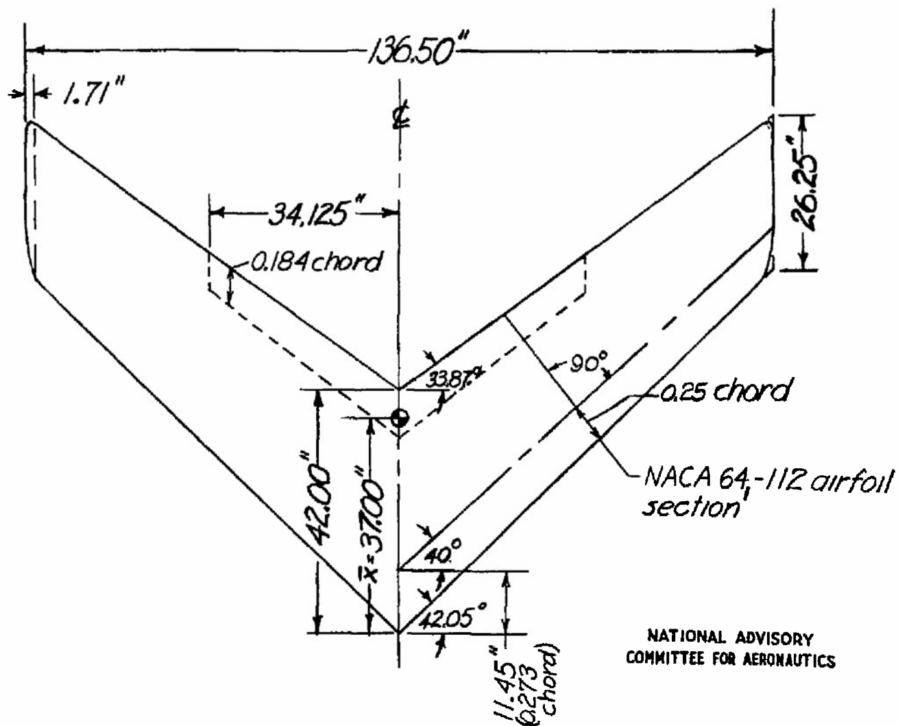
Figure 2.- Plan form of wing. Aspect ratio, 4.01; area, 4543 square inches; mean aerodynamic chord, 34.71 inches.
