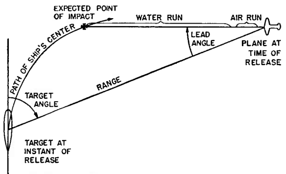
FIGURE 5. Position of target ship at instant torpedo is released, and expected point of impact.
