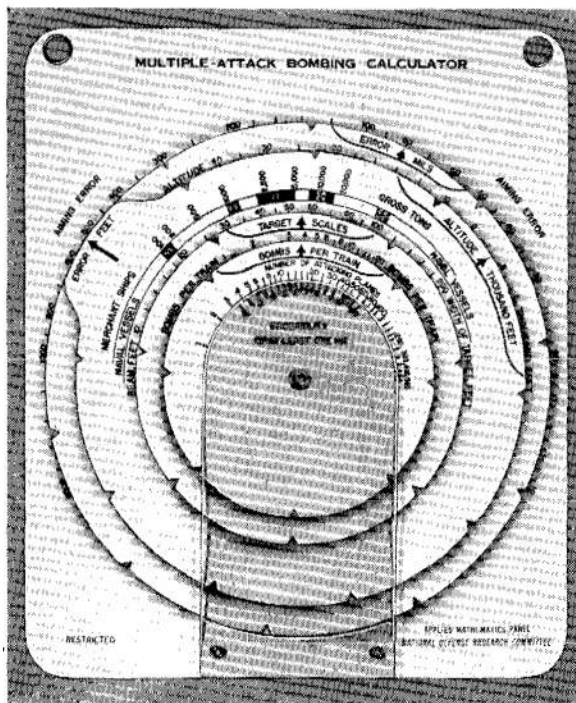
FIGURE 12. Photograph of AMP Multiple-Attack Bombing Calculator.
