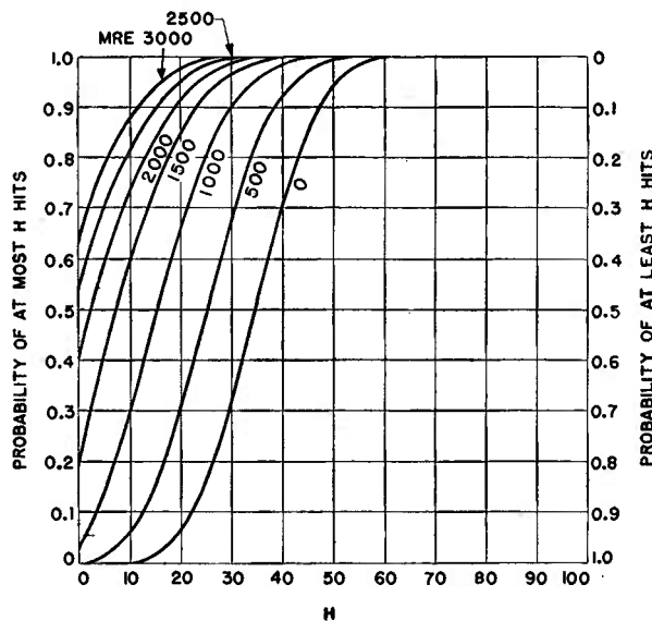
FIGURE 8. Graph showing the probability that the proportion of hits will be at most (or at least) H plotted against H . For double attacks ( s = 2 ); for operational patterns of area 3 \times 10^6 sq ft and circular target of radius 500 ft.
