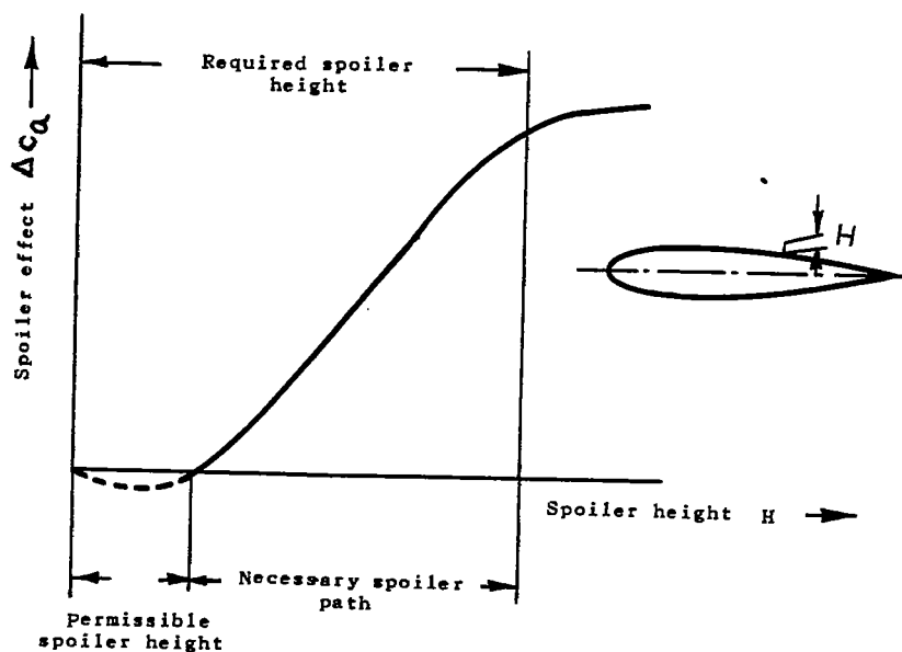
Figure 2.- Fundamental variation of the spoiler effect with the height of the spoiler.
