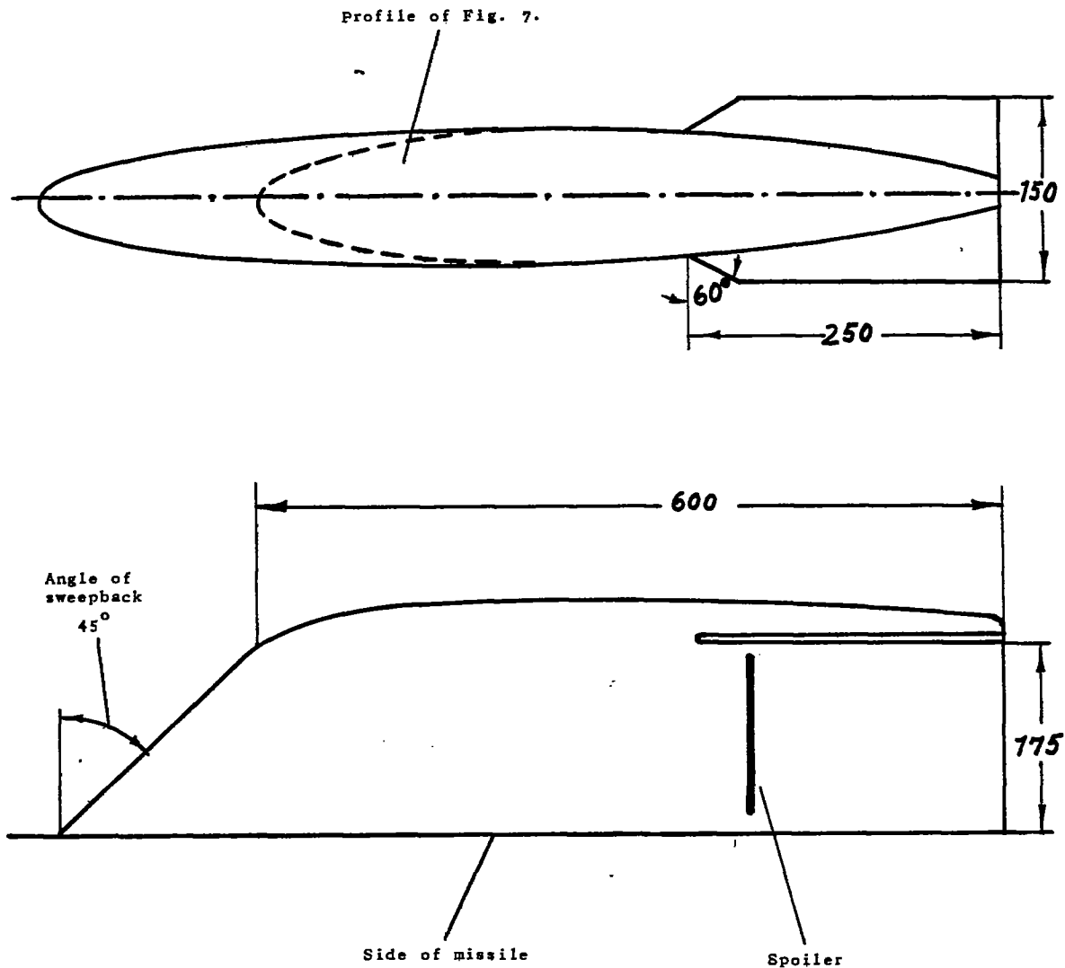
Figure 9.- Control element - leading edge 45^\circ sweepback, trailing edge straight.
