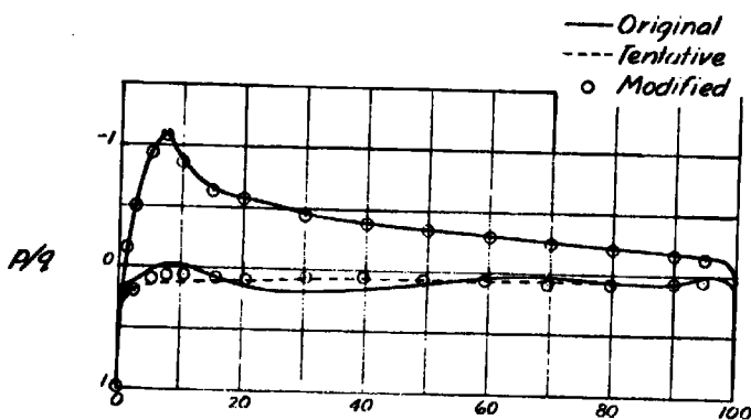
Figure 1.- Shape and pressure distribution, case I. (R.A.F. 15 airfoil)
