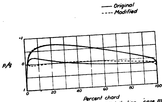
Figure 7. - Shape and pressure distribution, case III.
