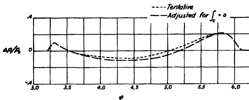
(b) Tentative and adjusted pressure changes.
