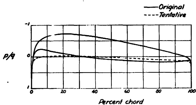
(a) Original and tentative pressure distributions.
