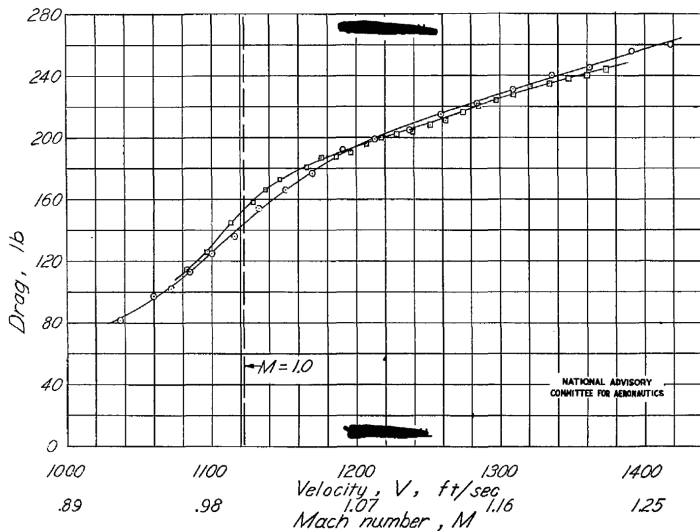
Figure 6.-Comparative drag measurements of two identical test vehicles with wings of arrowhead plan form
