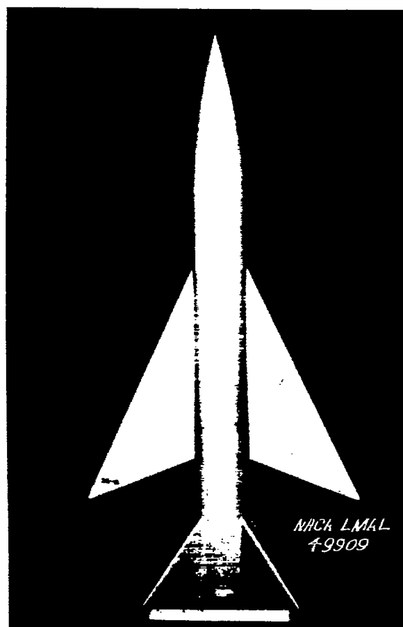
Figure 3.- The test vehicle with wing of arrowhead plan form.
