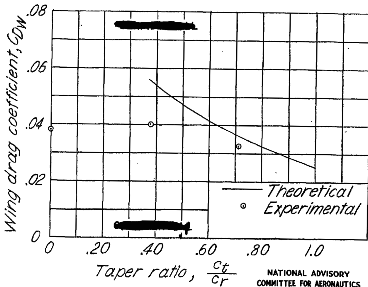
Figure 9.- Comparison of experimental and theoretical variation of wing drag coefficient with taper ratio. A_{exp} = 2.15 ; \Lambda_{L.E.} = 45^\circ ; M = 1.15 .
