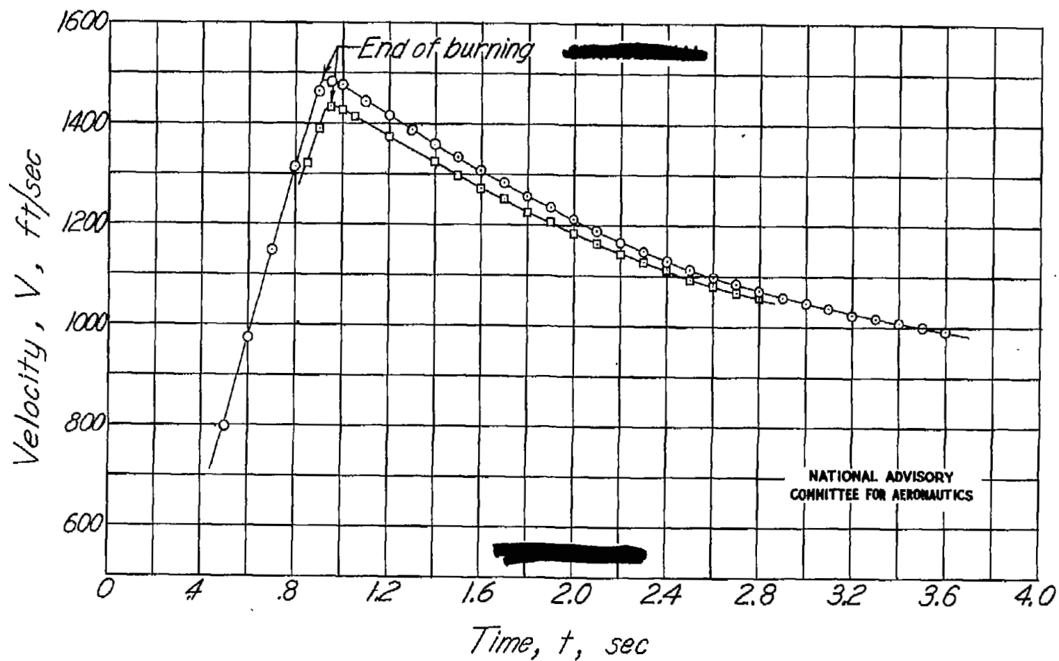
Figure 5. - Velocity-time curves for two identical test vehicles with wings of arrowhead plan form.
