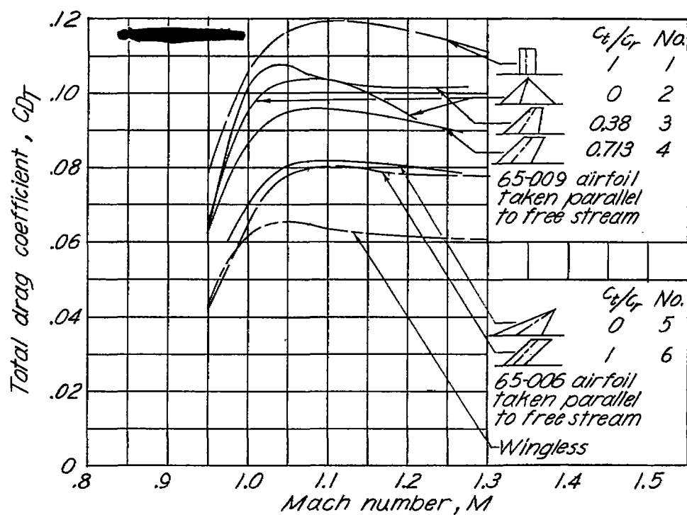
(a) Total drag coefficient.
