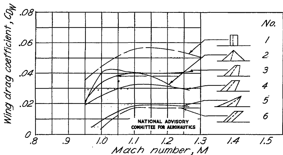
(b) Wing drag coefficient.
