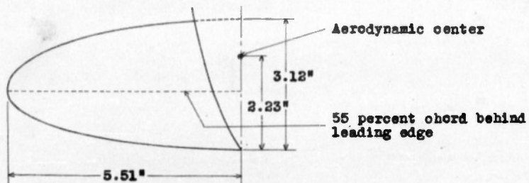
(c) Plan form of tail panel used in tail surfaces (NACA 0009 section; panel area, 13.5 sq in., including 3.04 sq in. in fuselage).
