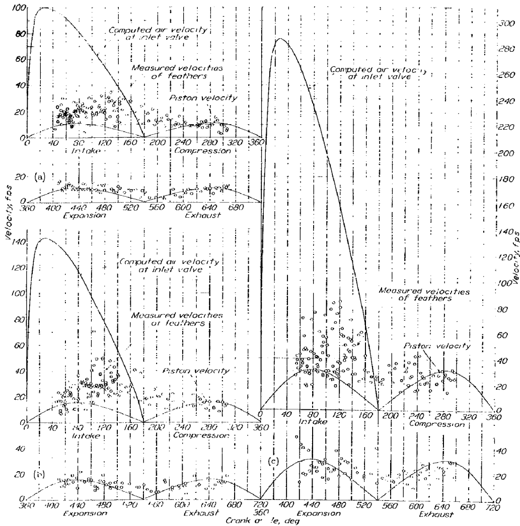
(a) Engine speed, 750 r.p.m. (b) Engine speed, 500 r.p.m. (c) Engine speed, 1,000 r.p.m.
