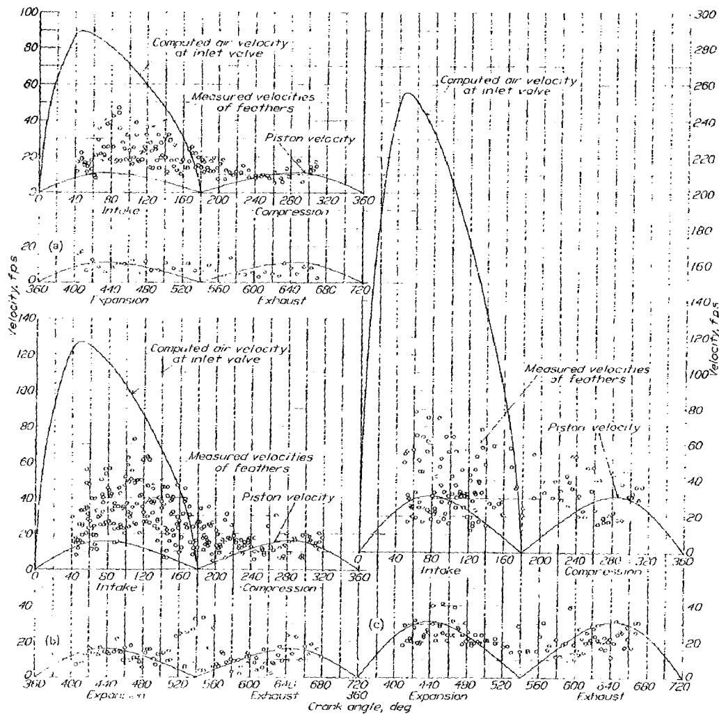
(a) Engine speed, 360 r.p.m. (b) Engine speed, 500 r.p.m. (c) Engine speed, 1,600 r.p.m.
