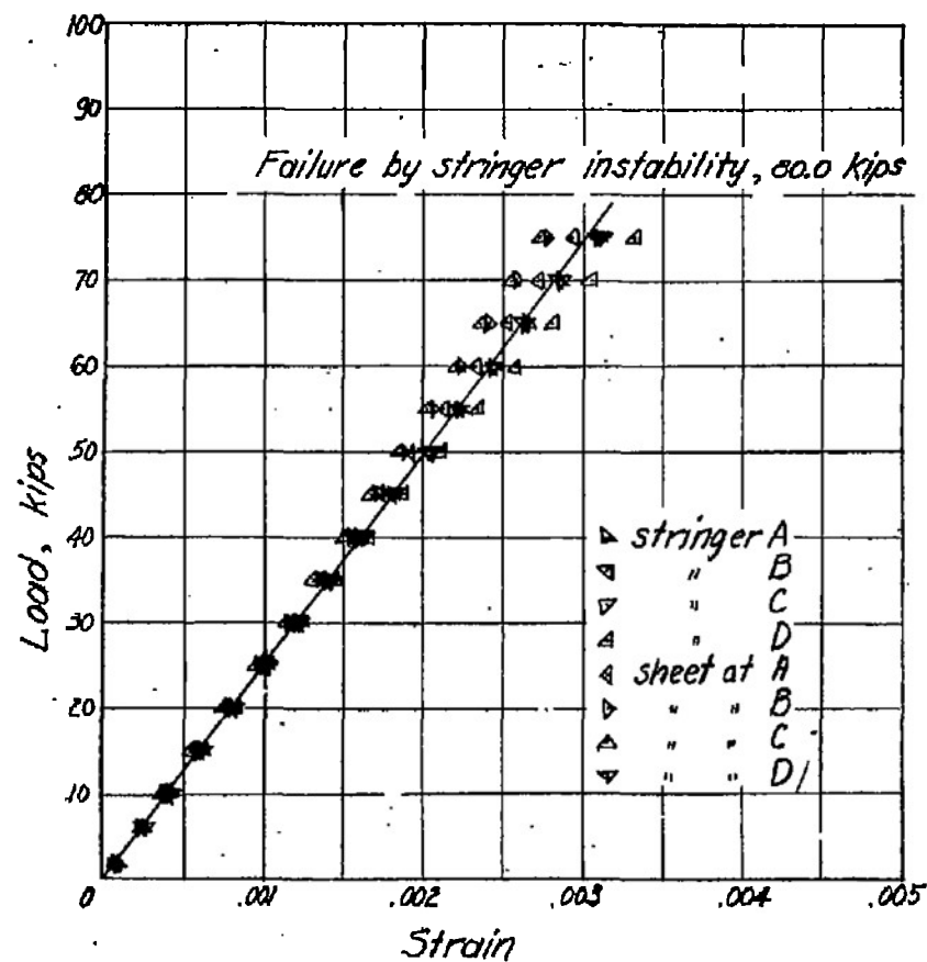
Figure 20.- Test of panel 15; radius, 35.5 inches.
