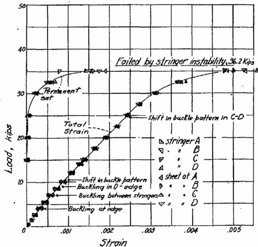
Figure 6.- Test of panel 1; radius, 78.5 inches.
