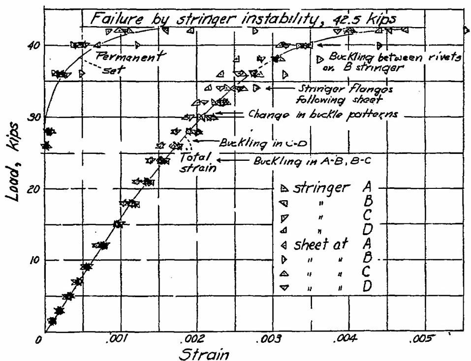
Figure 15.- Test of panel 10; radius, 25.5 inches.
