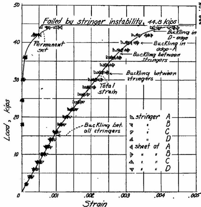
Figure 13.- Test of panel 8; radius, 76.5 inches.
