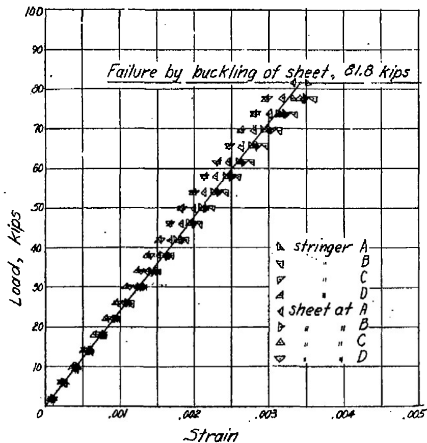
Figure 21.- Test of panel 16; radius, 19.1 inches, (BR-4 gages used after 73.8 kips).
