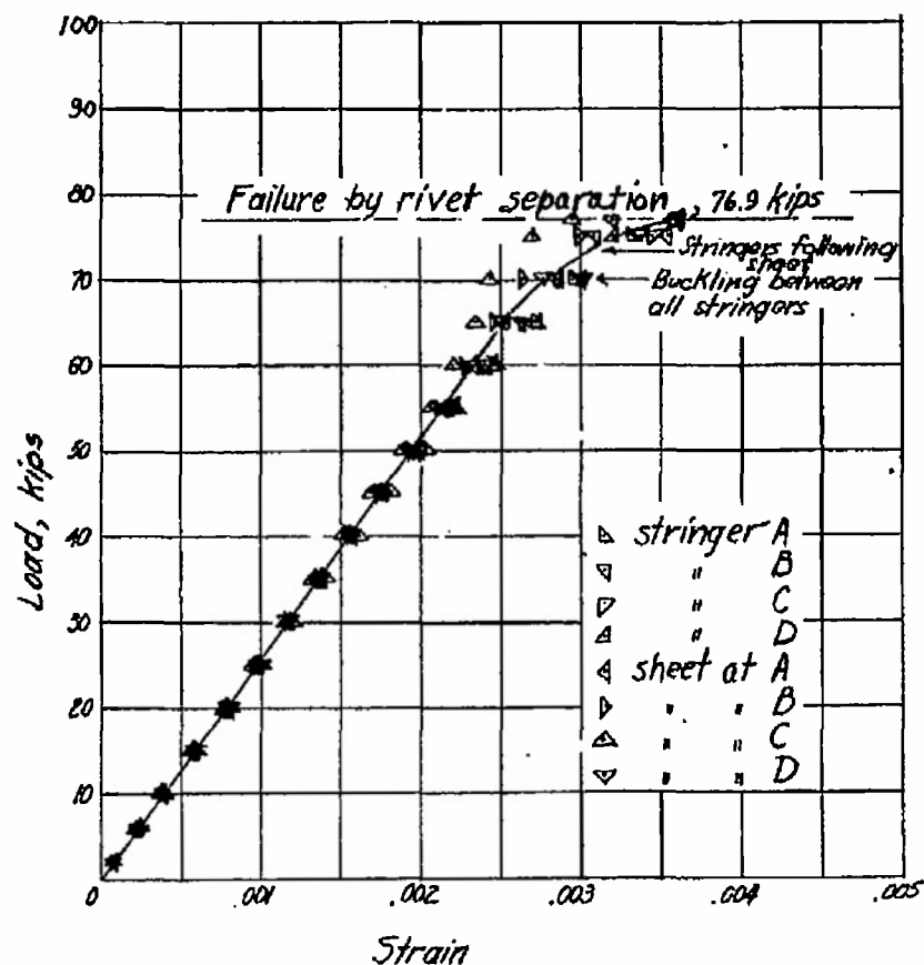
Figure 18.- Test of panel 13; radius, 78.5 inches.
