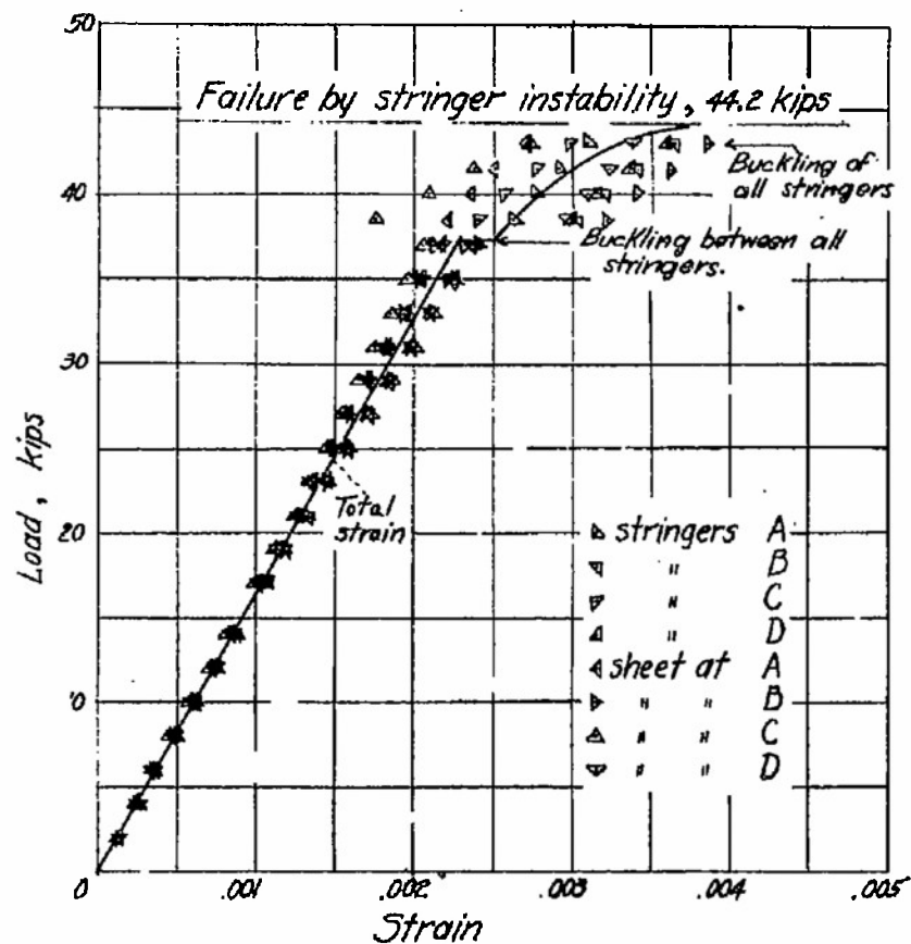
Figure 16.- Test of panel 11; radius, 19.1 inches, (BR-4 gages used to reset Tuckerman gages after buckling at 37.1 kips).
