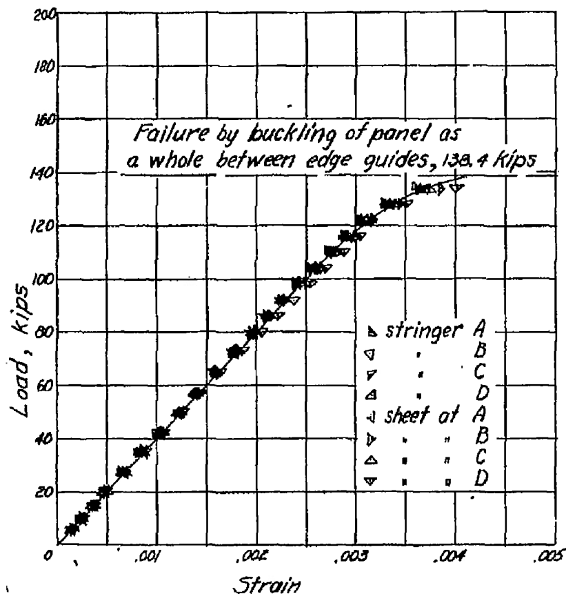
Figure 22.- Test of panel 17; flat sheet, (SR-4 gages used after 116 kips).
