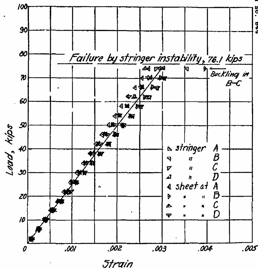
Figure 19.- Test of panel 14; radius, 38.5 inches. (8R-4 gages used after 70.0 kips).
