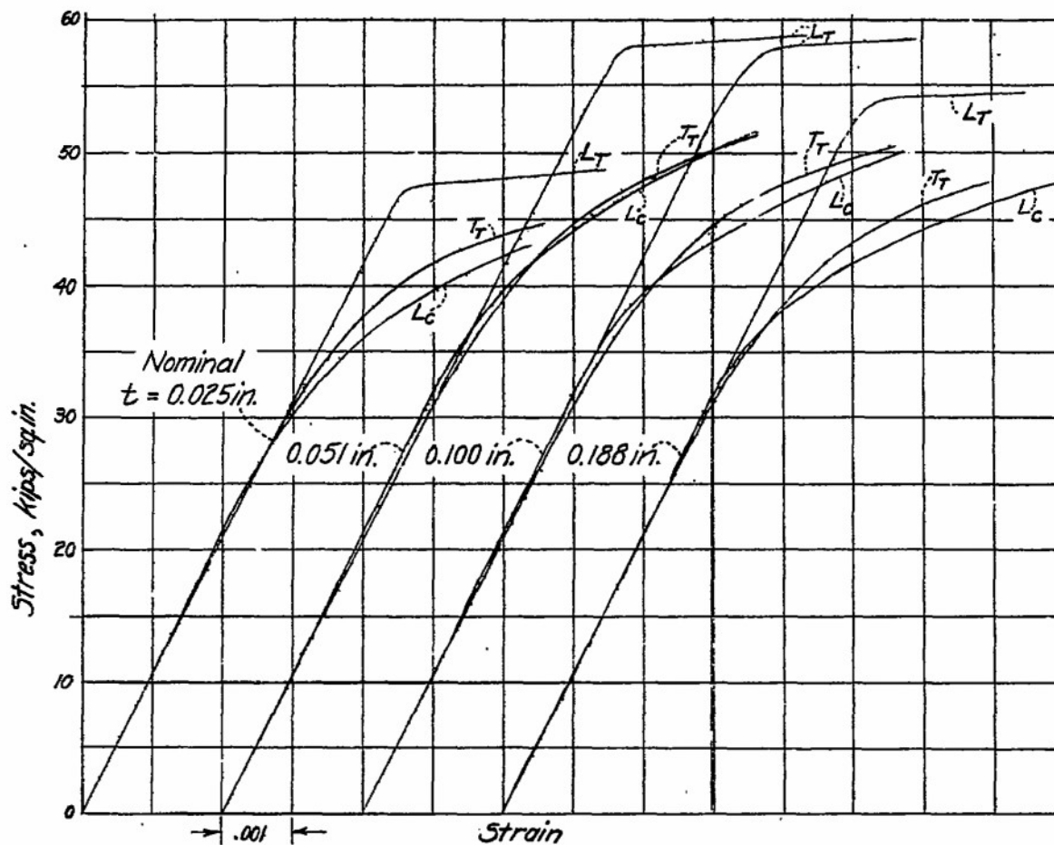
Figure 2.- Stress-strain curves of 24S-T aluminum alloy sheet used in panels. L_T , tension in direction of rolling; L_C , compression in direction of rolling; T_T , tension transverse to direction of rolling.
