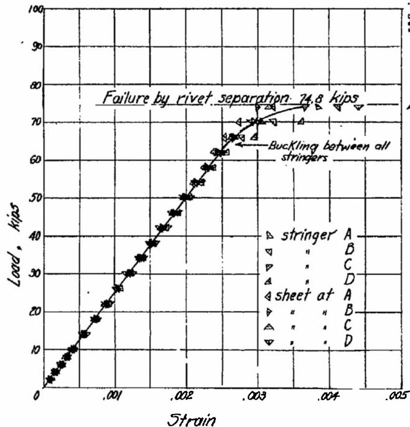
Figure 17.- Test of panel 12; flat sheet, (BR-4 gages used after 70.0 kips).
