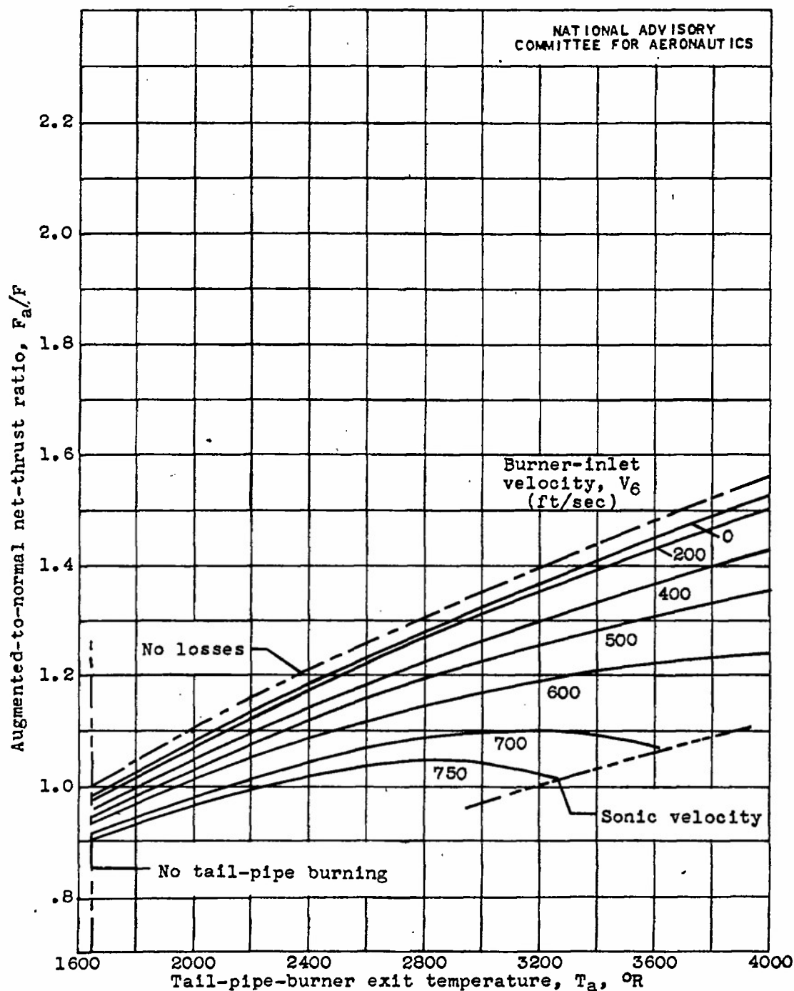
Figure 6. - Variation of augmented-to-normal net-thrust ratio with tail-pipe-burner exit temperature for various burner-inlet velocities. V_5 , 750 feet per second; T_5 , 1650 ^{\circ} R; C_D , 1.0; \eta_d , 0.8; C_V , 0.975.
