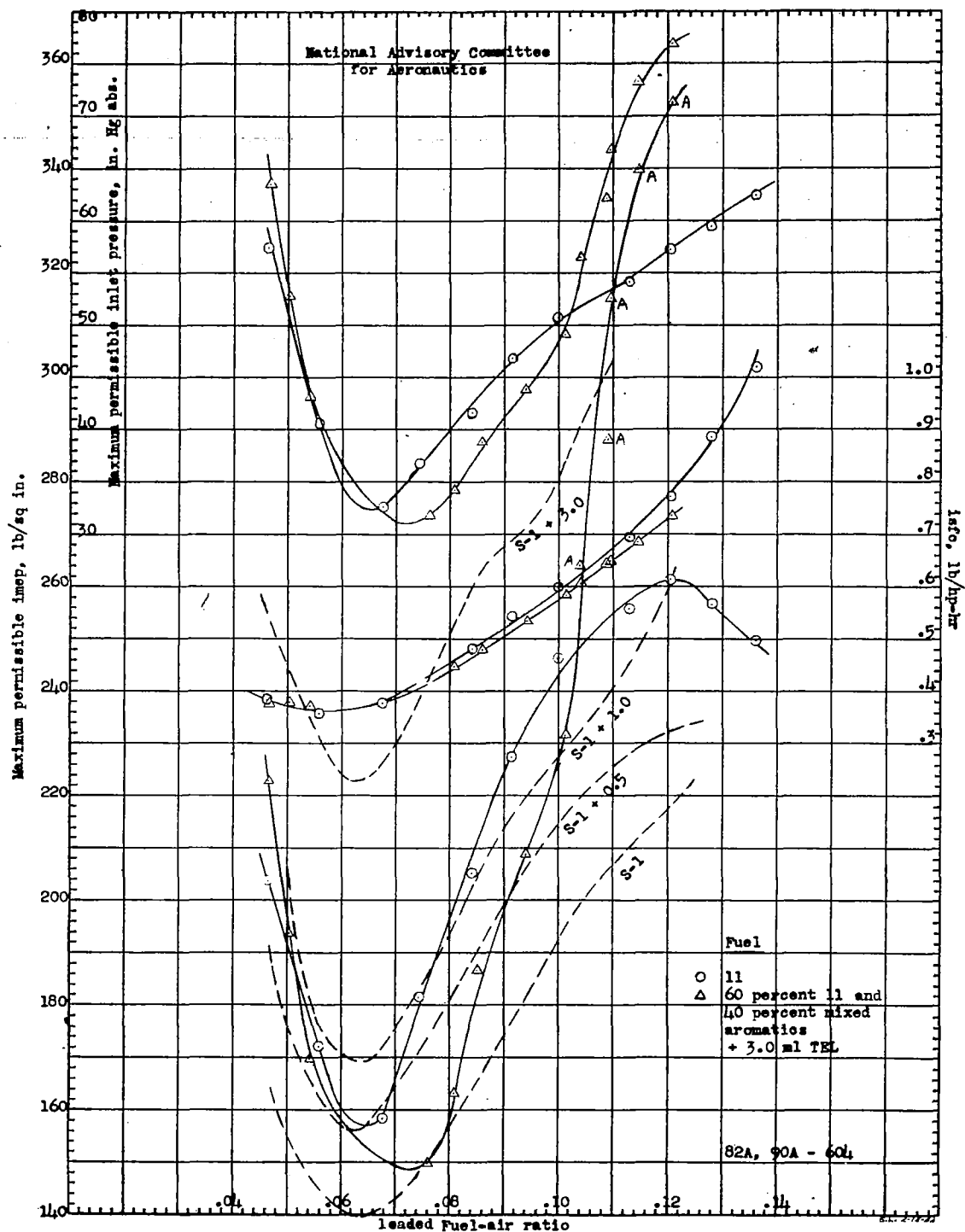
Figure 25. - Effect of addition of mixed aromatics on NACA fuel 11 at 3100 rpm and 250°F inlet-air temperature. Lycoming O-1230 cylinder; spark advance, 29°; coolant inlet temperature, 250°F; compression ratio, 7.0.
