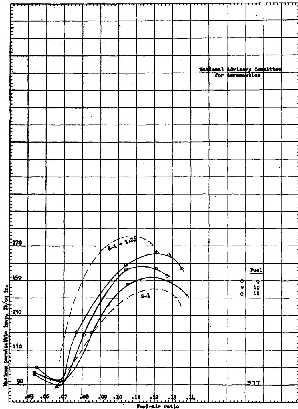
Figure 5 . - Comparative performance of NACA fuels 9, 10, and 11 by 3-C Method. 2-5/8-inch C.F.R. engine; engine speed, 1800 rpm; spark advance, 45^\circ ; coolant temperature, 375^\circ\text{F} ; compression ratio, 7.0; intake-air temperature, 225^\circ\text{F} . Data from Esso Laboratories.
