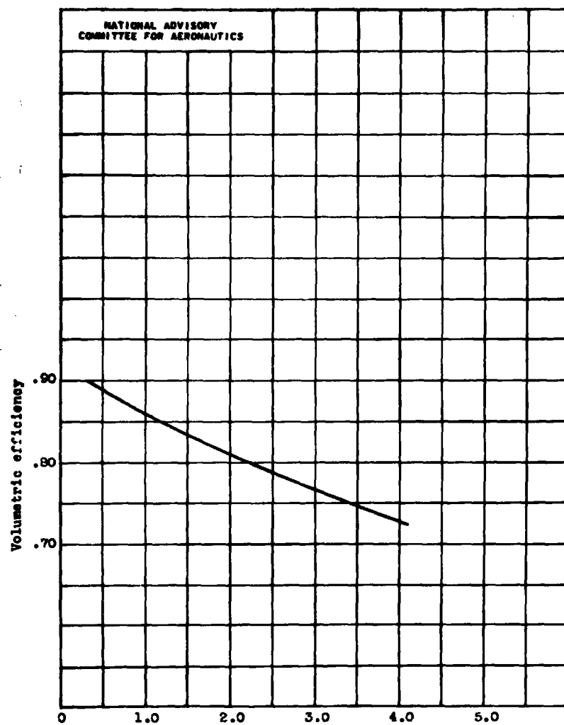
Figure 9. - Effect of ratio of exhaust back pressure to inlet-air pressure on volumetric efficiency of compression-ignition engine with no valve overlap. Engine speed, 2200 rpm; compression ratio, 13.0.
