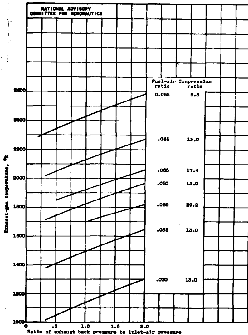
Figure 10. - Variation of exhaust-gas temperature with ratio of exhaust back pressure to inlet-air pressure for various fuel-air ratios and compression ratios.
