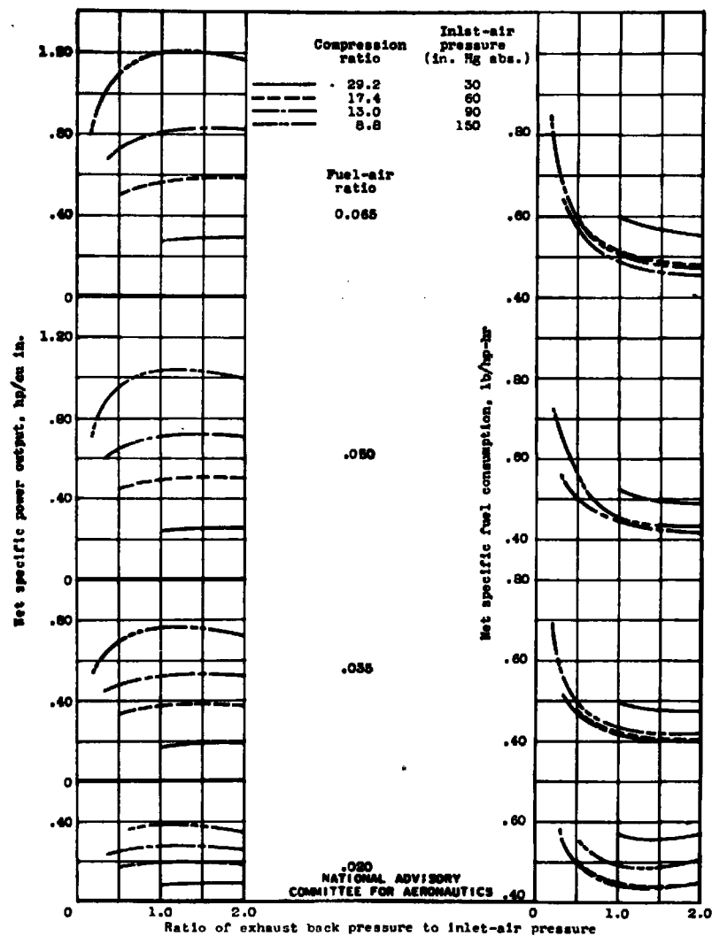
Figure 2. - Variation of net specific power output and corresponding net specific fuel consumption with ratio of exhaust back pressure to inlet-air pressure for various fuel-air ratios and compression ratios. Maximum cylinder pressure maintained constant at 1400 pounds per square inch; engine speed, 2200 rpm; compressor efficiency, 0.70; turbine efficiency, 0.65.
