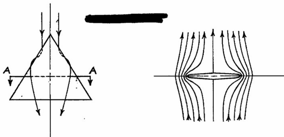
(a) Elements of flow over a triangular wing having a rounded leading edge at high Reynolds numbers.
