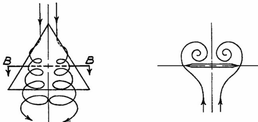
(c) Elements of flow over a triangular wing at low Reynolds numbers or over a triangular wing having a sharp leading edge.
