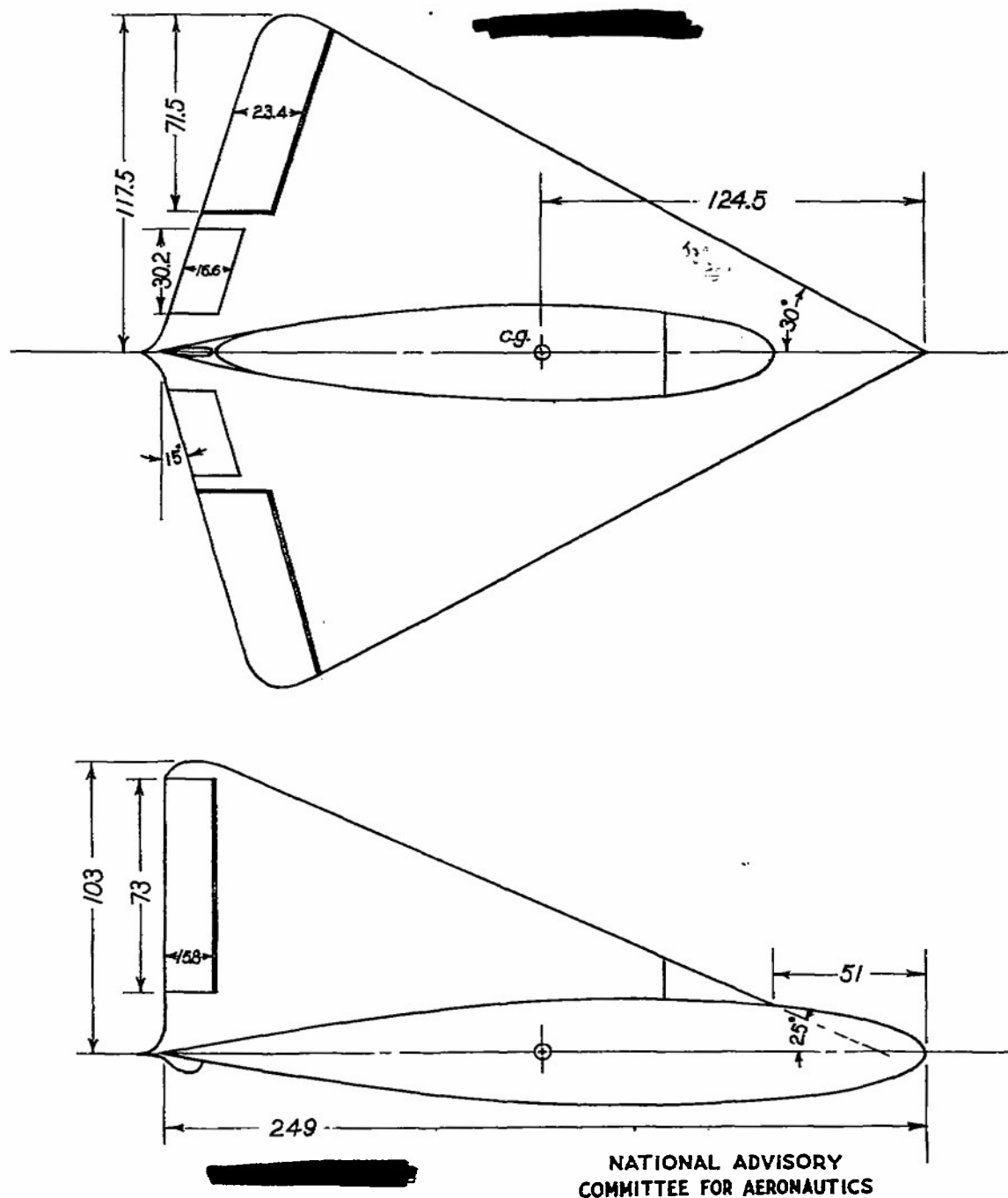
(A) Principal dimensions of original glider.
