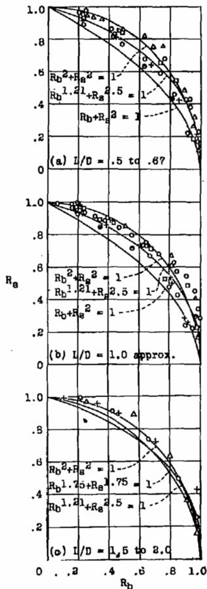
Figure 15.- Plot of test results for cylinders under combined pure bending and pure torsion loads.
