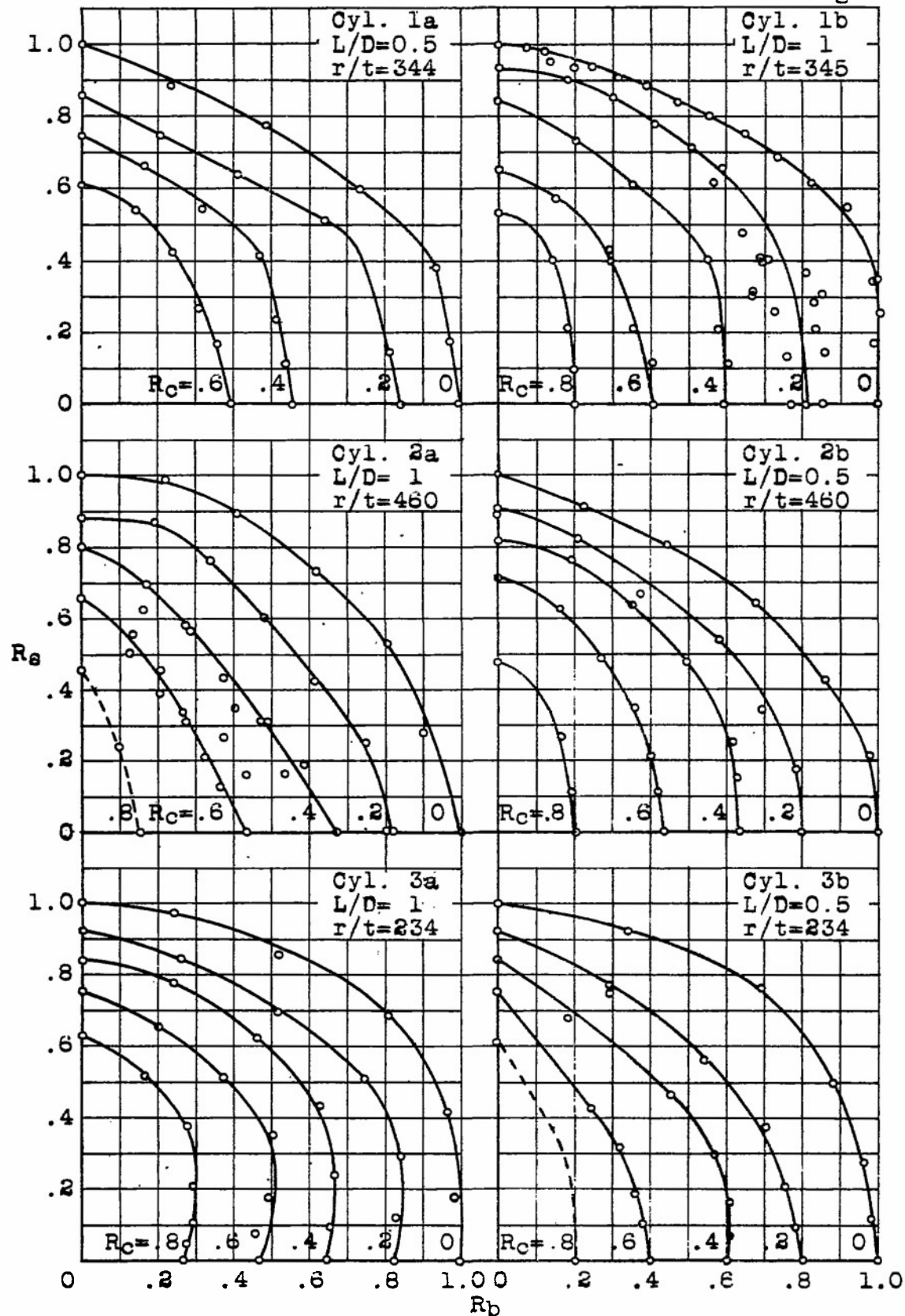
Figure 16.- Plot of test results for various test cylinders loaded in combined compression, pure bending and pure torsion.
