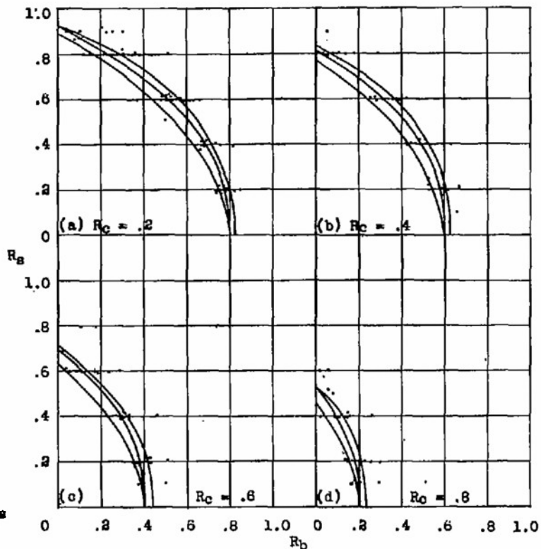
Figure 15.- Plot of test results for cylinders under combined pure bending and pure torsion loads.
