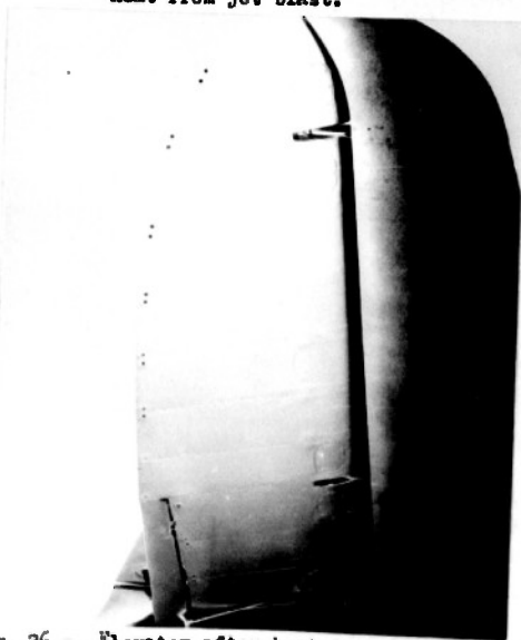
Fig. 26 -- Elevator after heat resistant treatment applied.
