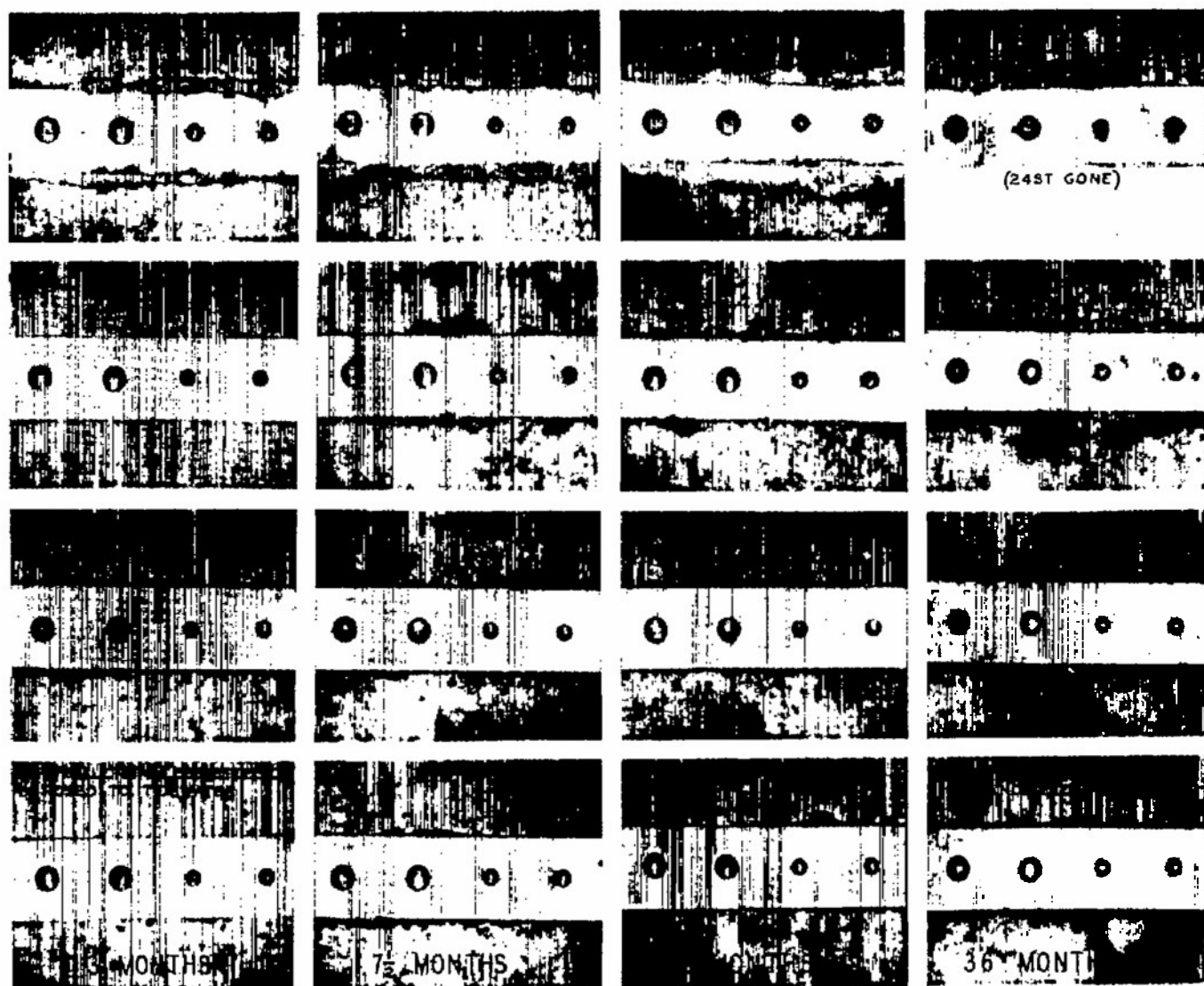
Figure 29.- Strips of stainless steel, coupled in a 1:7 area ratio with panels of aluminum alloys, and exposed to the tidewater at Hampton Roads, Va. for the periods indicated. Note that the aluminum alloys are less severely attacked, and the quantities of corrosion products at the edges of juncture are less than in figure 28. x 1/3.
