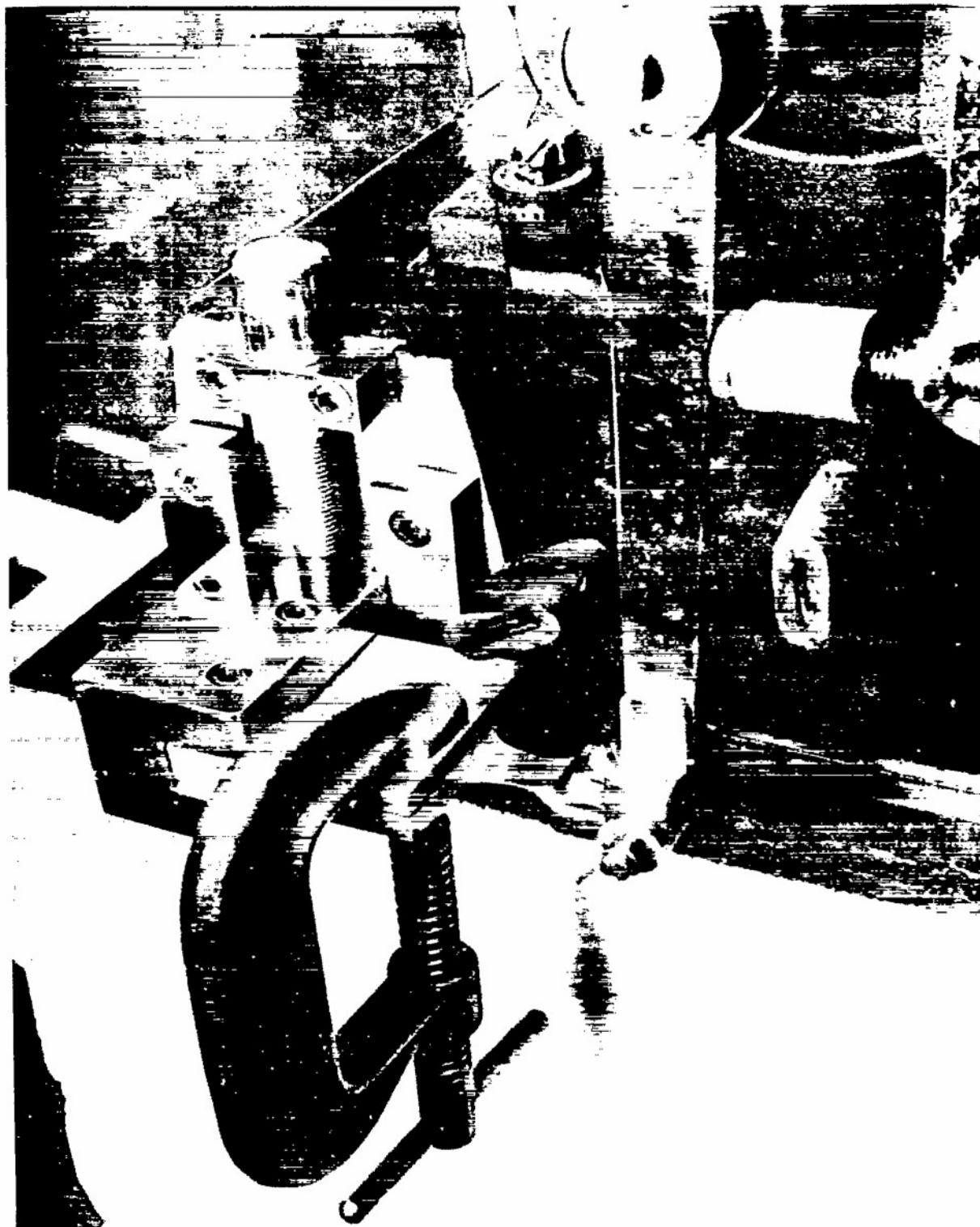
Figure 7.- A specimen in the Krouse flexural fatigue testing machine, showing the method of attaching it at the fixed and loading ends.
