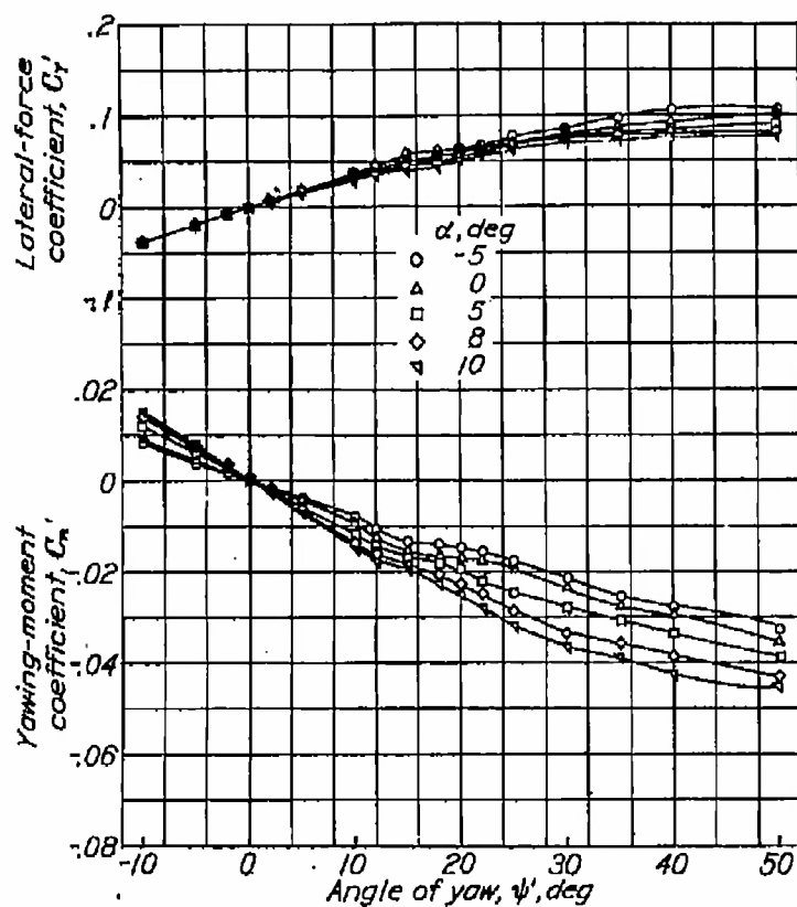
Figure 20.- Yawing-moment and lateral-force coefficients for high-wing combination. \delta_F = 60^\circ .
