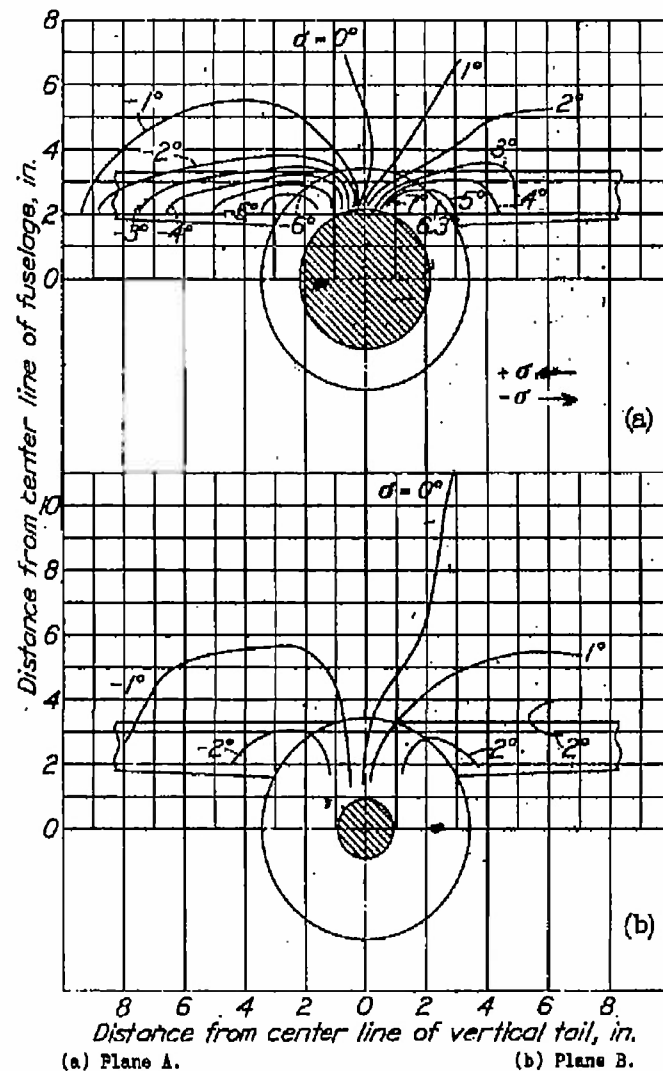
Figure 5.- Contours of sidewash angle, \sigma , in region of tail. \alpha = 0^\circ ; \psi = 0^\circ ; high wing; \delta_T = 0^\circ .
