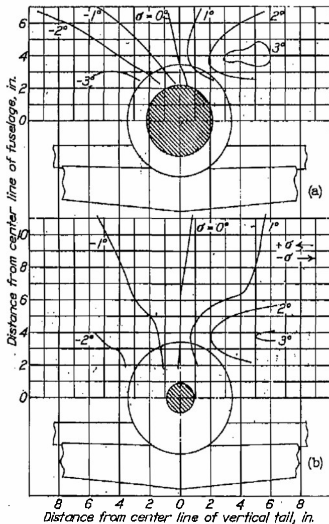
Figure 8.- \alpha = 0^\circ , \psi' = 0^\circ , low wing; \delta_F = 60^\circ .
