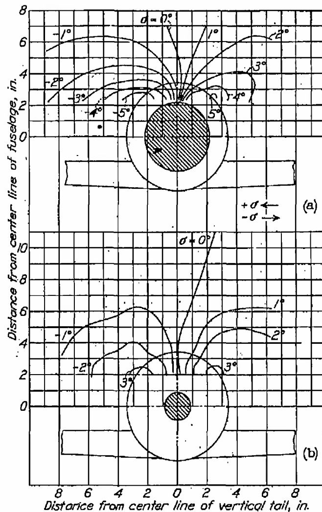
(a) Plane A. (b) Plane B. Figure 7.- \alpha = 0^\circ ; \psi' = 0^\circ ; low wing; \delta_F = 0^\circ .
