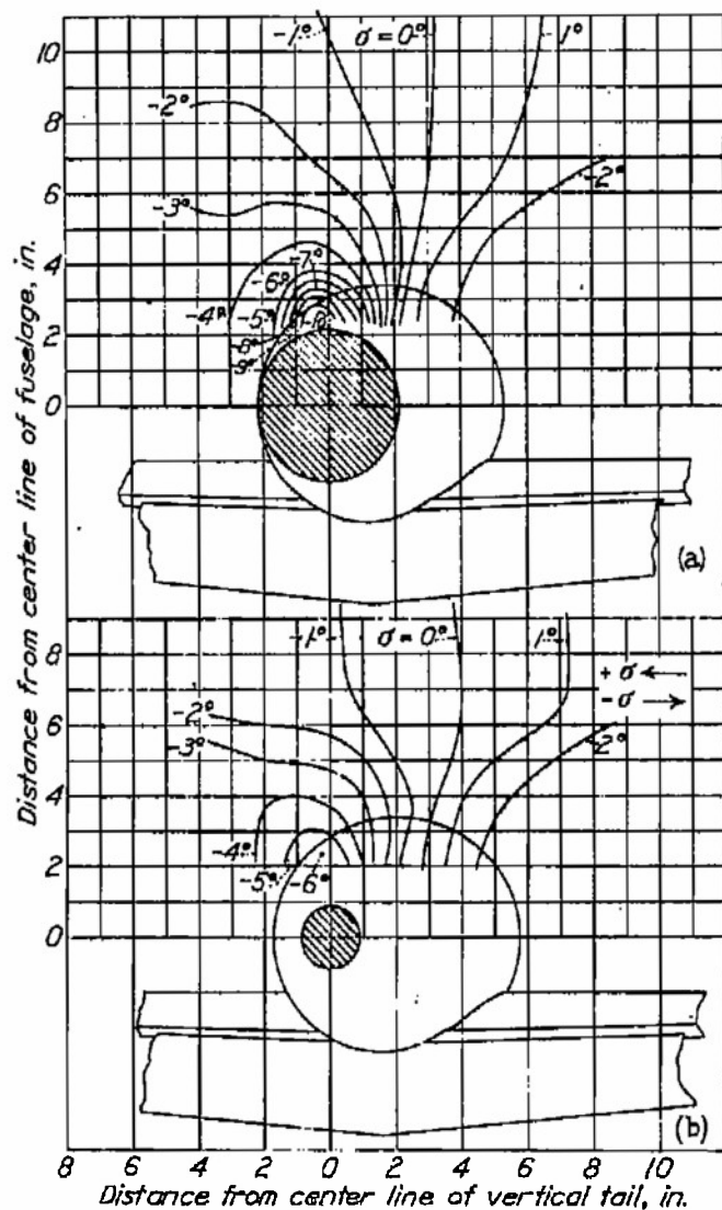
Figure 12.- \alpha = 0^\circ ; \psi' = 0^\circ ; low wing; \delta_f = 60^\circ .
