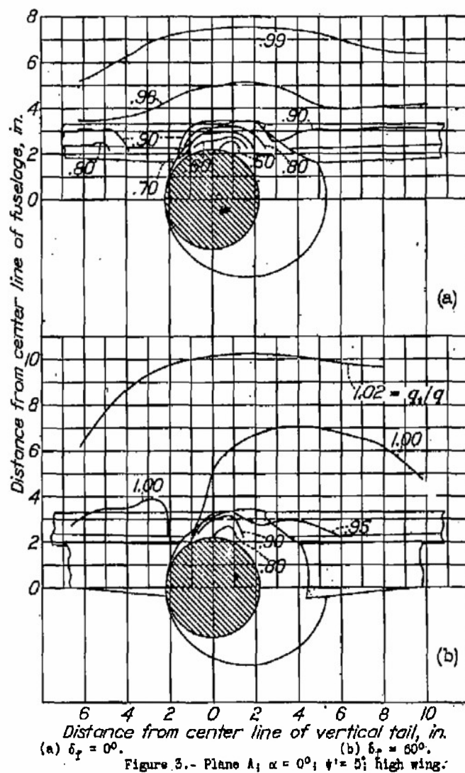
Figures 2,3.- Contours of dynamic-pressure ratio, q_t/q , in region of tail.
