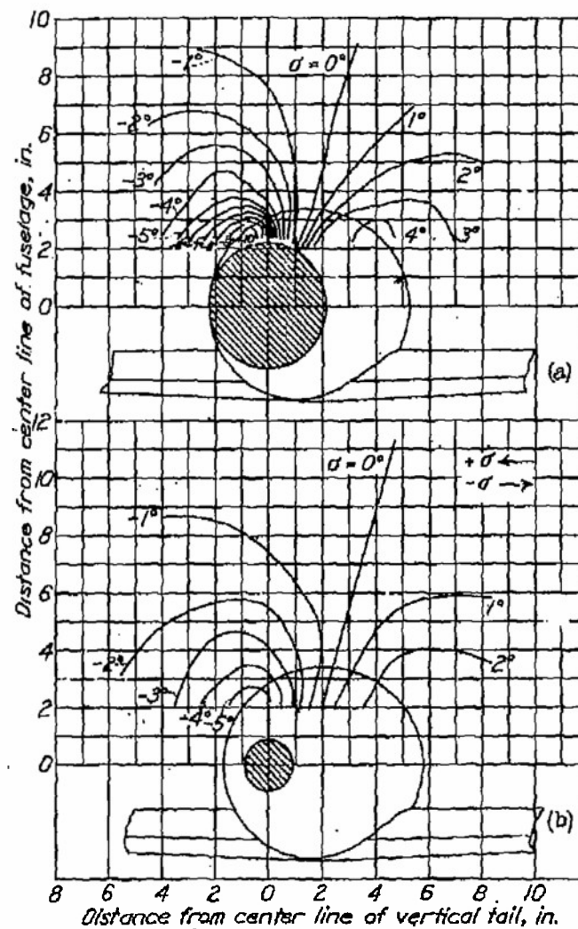
(a) Plane A. (b) Plane B. Figure 11.- \alpha = 0^\circ ; \psi' = 5^\circ ; low wing; \delta_F = 0^\circ .
