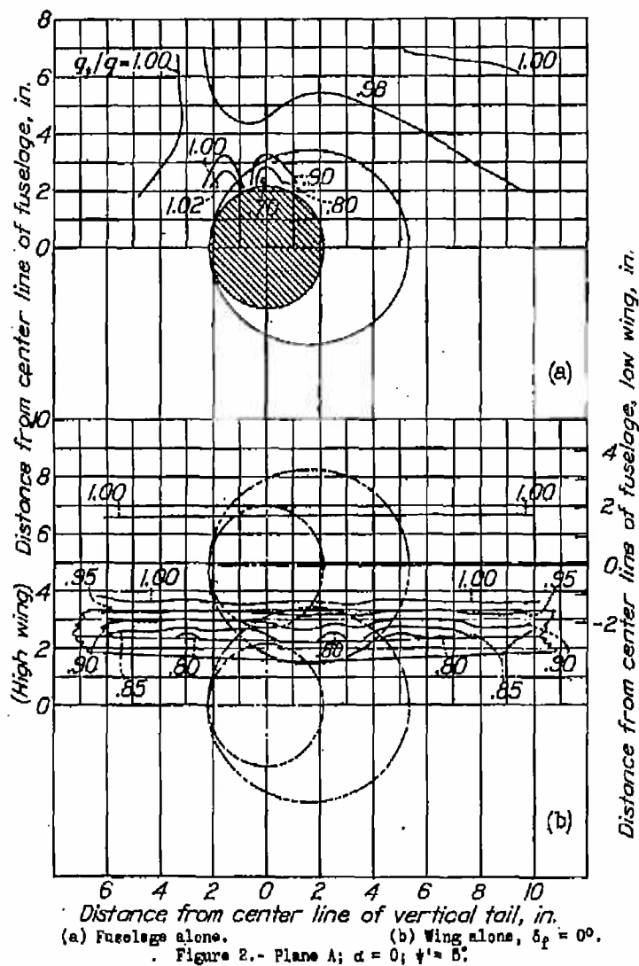
Figures 2,3.- Contours of dynamic-pressure ratio, q_t/q , in region of tail.
