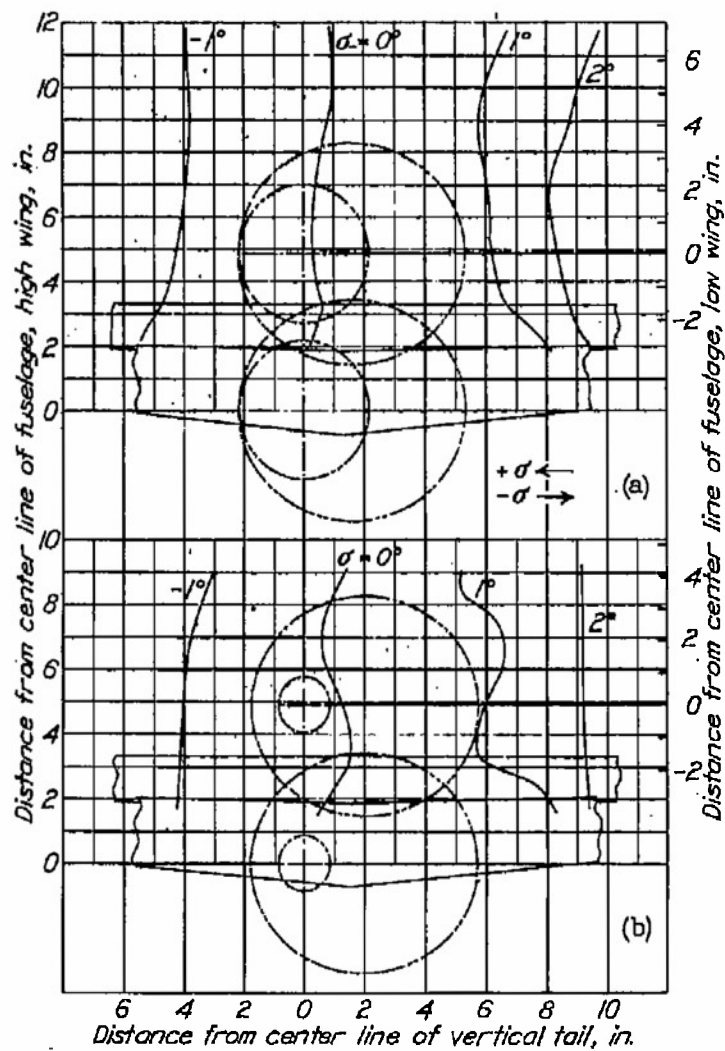
(a) Plane A. (b) Plane B. Figure 14.- \alpha = 0^\circ , \psi' = 5^\circ ; wing alone; \delta_F = 60^\circ .
