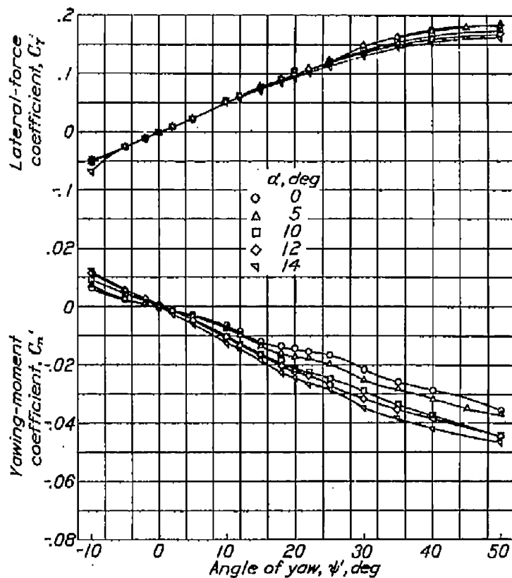
Figure 19.- Yawing-moment and lateral-force coefficients for high-wing combination with tail. \delta_f = 0^\circ .
