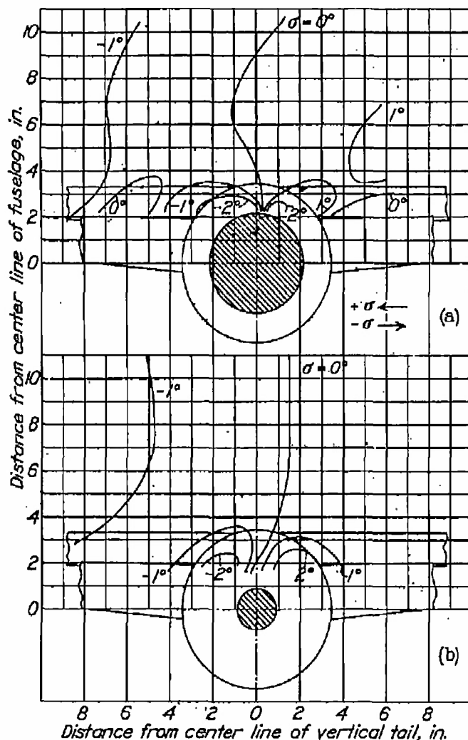
(a) Plane A. (b) Plane B. Figure 6.- \alpha = 0^\circ ; \psi' = 0^\circ ; high wing; \delta_F = 60^\circ .
