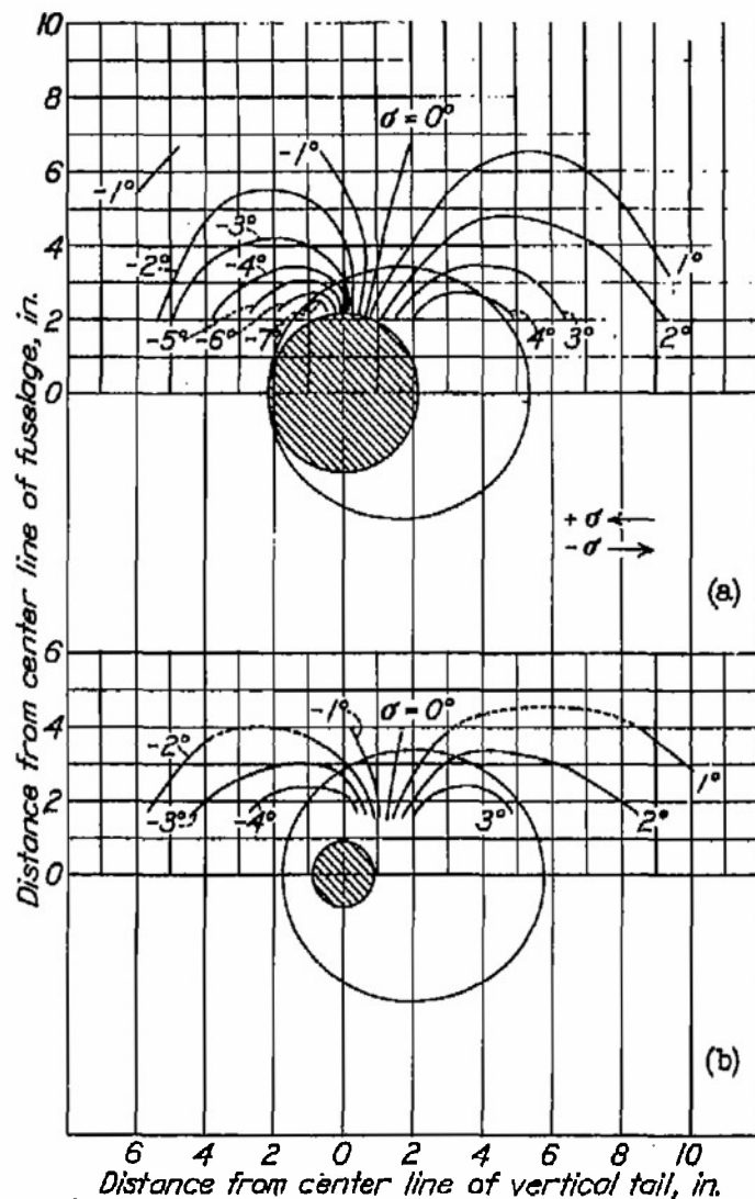
Figure 16.- Contours of sidewash, \sigma , in region of tail. \alpha = 0^\circ ; \psi' = 5^\circ ; fuselage alone.
