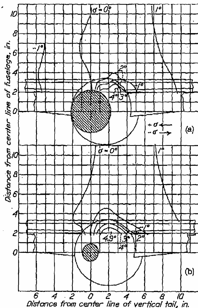
(a) Plane A. (b) Plane B. Figure 10.- \alpha = 0^\circ ; \psi' = 5^\circ ; high wing; \delta_F = 60^\circ .
