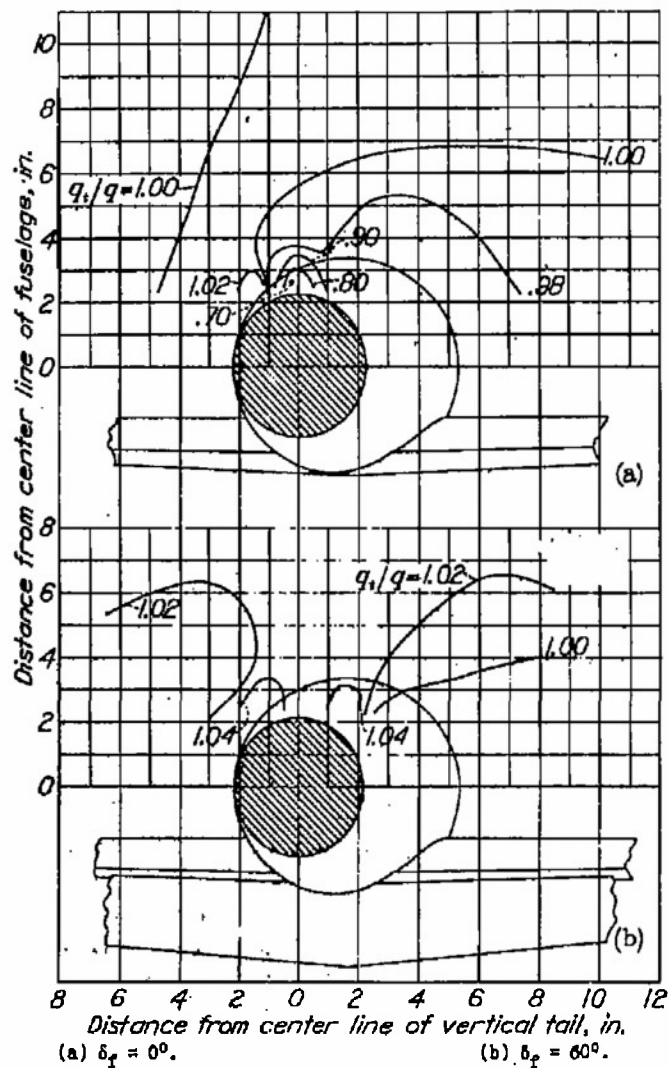
Figure 4.- Contours of dynamic pressure ratio, q_t/q , in region of tail. Plane A; \alpha = 0^\circ ; \psi = 60^\circ ; low wing.
