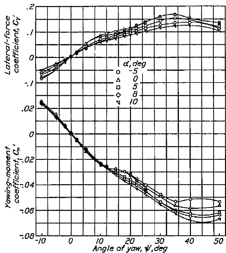
Figure 18.- Yawing-moment and lateral-force coefficients for low-wing combination with tail. \delta_f = 60^\circ .
