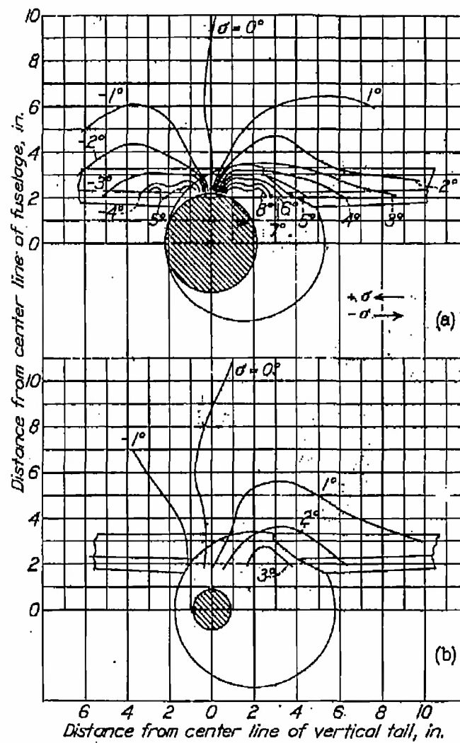
Figure 9.- \alpha = 0^\circ , \psi' = 5^\circ , high wing; \delta_F = 0^\circ .
