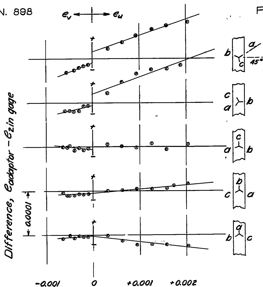
Figure 12.-Strain, from 2 in gages
