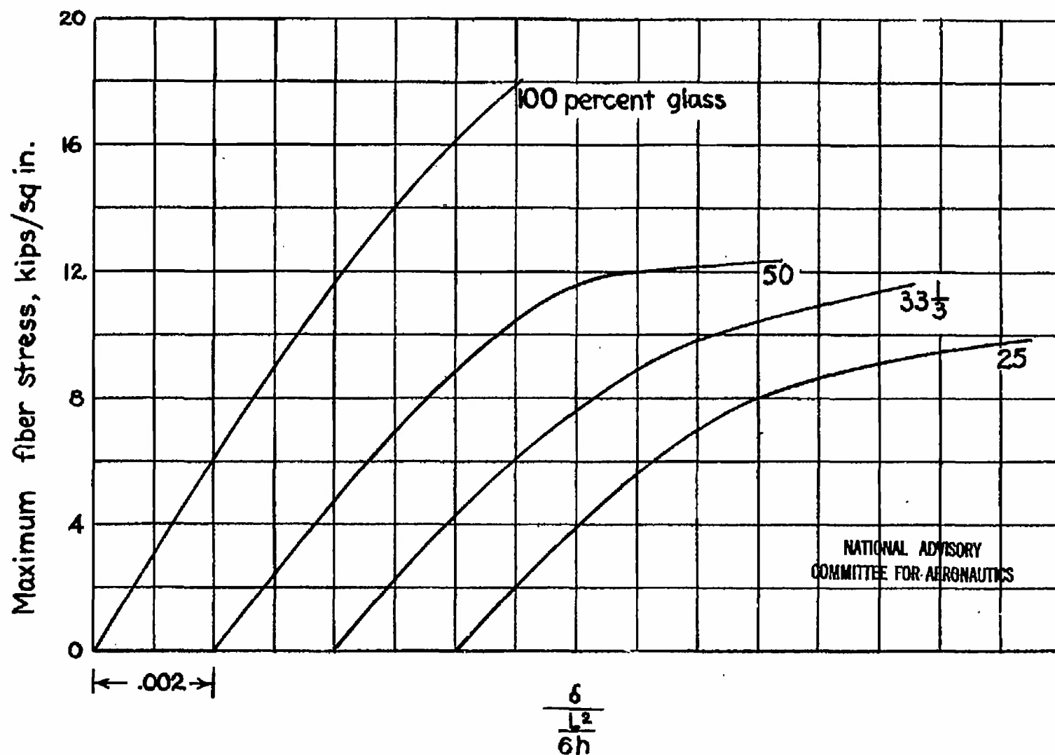
Figure 15.- Longitudinal bending stress-strain curves.
