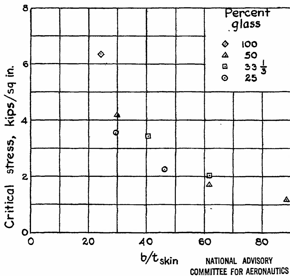
Figure 18.-Variation of critical compressive stress for sheet between stiffeners with b/t_{skin} .
