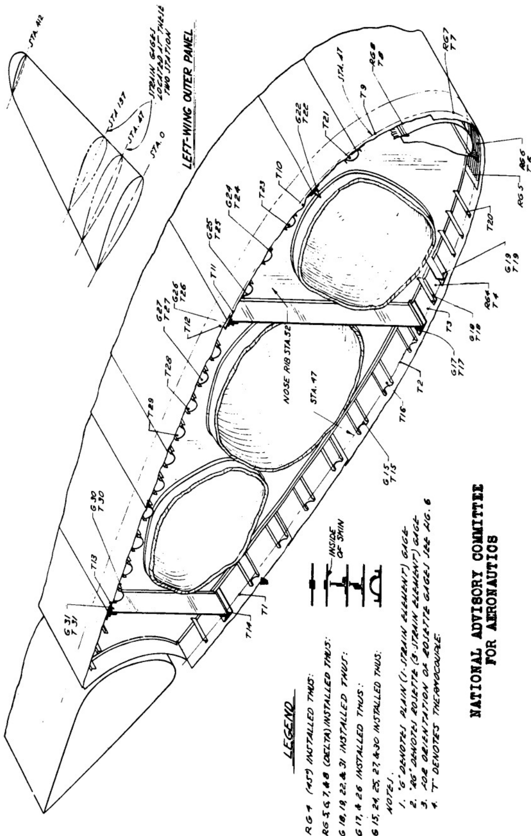
Figure 4.- Location of strain gages and thermocouples at wing outer-panel station 47, C-46 airplane.
