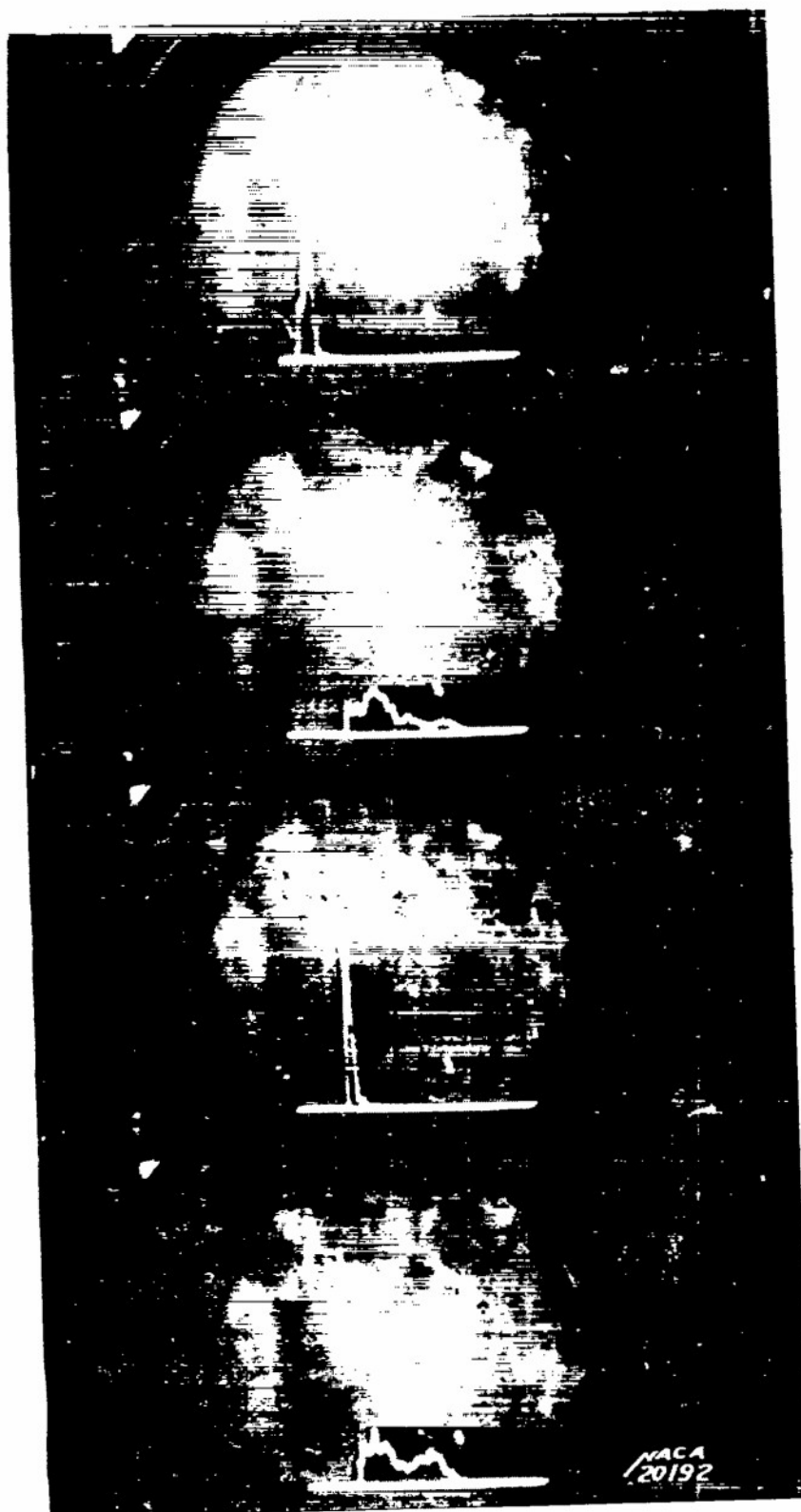
Figure 4.-- Ioniza- tion- current records of four successive engine cycles. In the first and the third cycles, knock was present.
