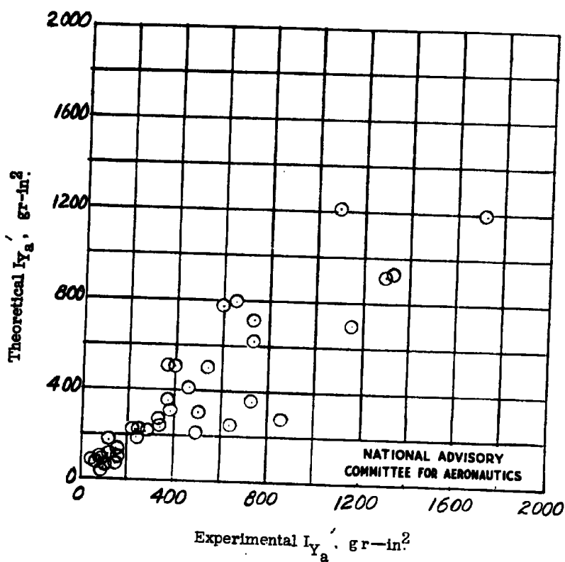
Figure 10.- Comparison of the experimental and calculated model values of the additional moments of inertia about the Y-swinging axis for 40 free-spinning models.
