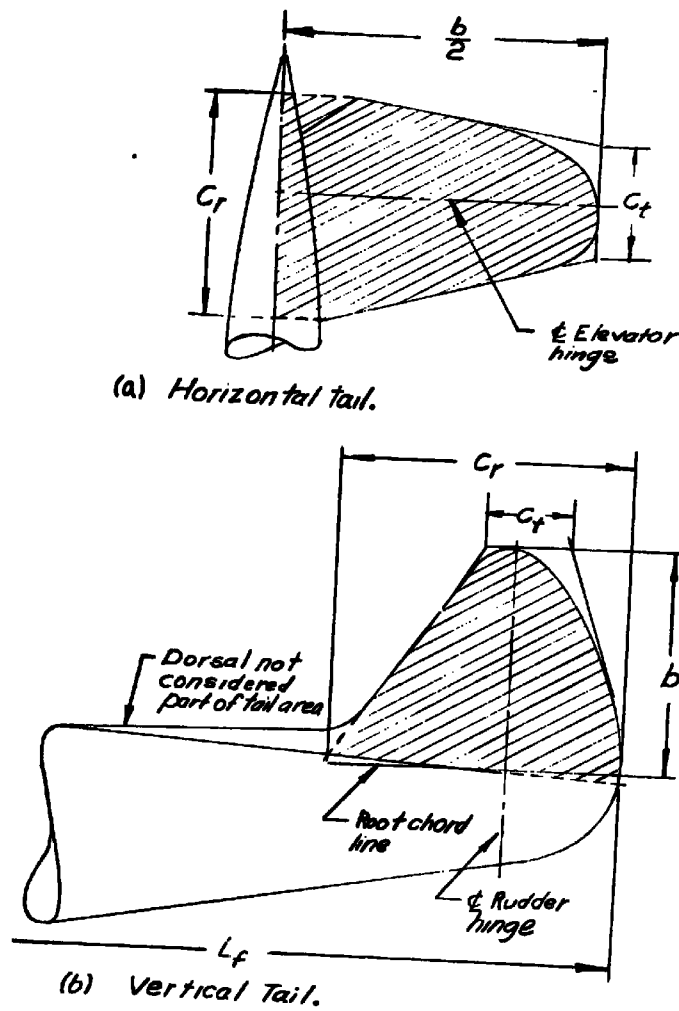
Figure 2.- Sketch illustrating method of measuring the chords, span, and area of the horizontal and vertical tail surfaces;
