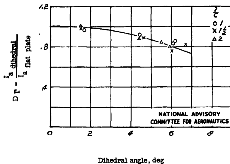
Figure 5.- Variation of the additional moments of inertia of a single plate with dihedral angle; A = 4 (reference 5).
