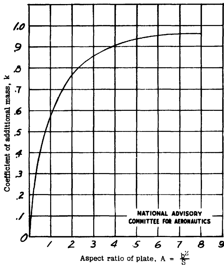
Figure 3.- Coefficients of additional mass for rectangular plates. Curve is average of NACA 1933 and 1940 tests. (Reference 5)
