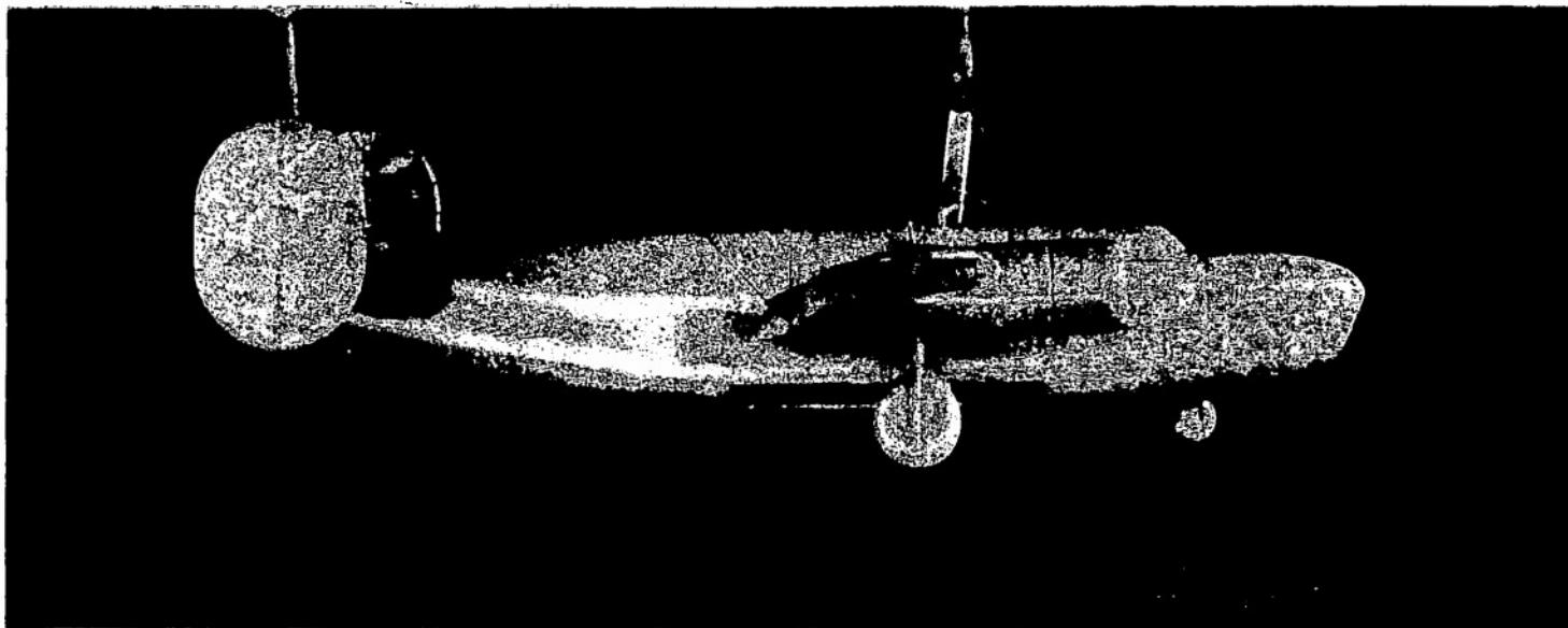
(b) Side view. The nose wheel is notched so that it can fall back partially into the open wheel compartment.
