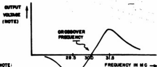
FIG. 4-2 THE COMPLETE DISCRIMINATOR CHARACTERISTIC.
