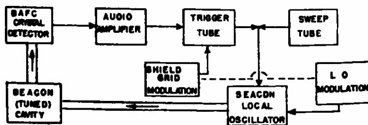
FIG. 4-3 BLOCK DIAGRAM OF BEACON AFC.
