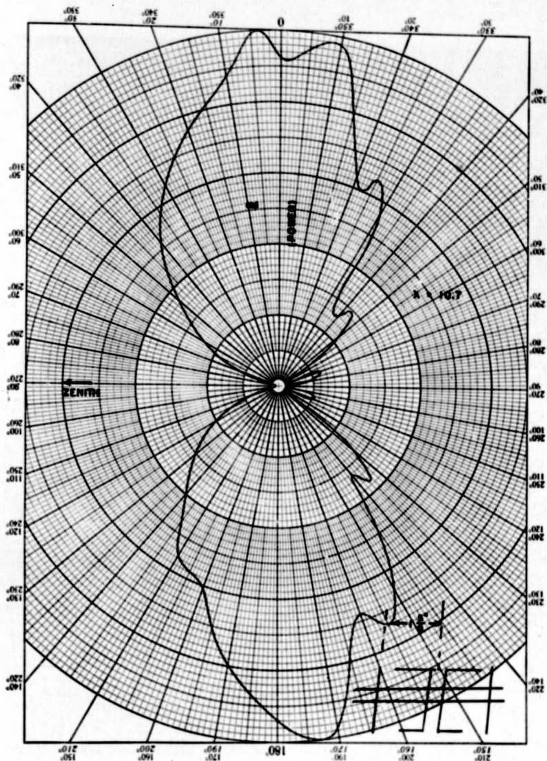
FIG. 10 - ELEVATION PATTERN OF SINGLE DOUBLE H ELEMENT ANTENNA
