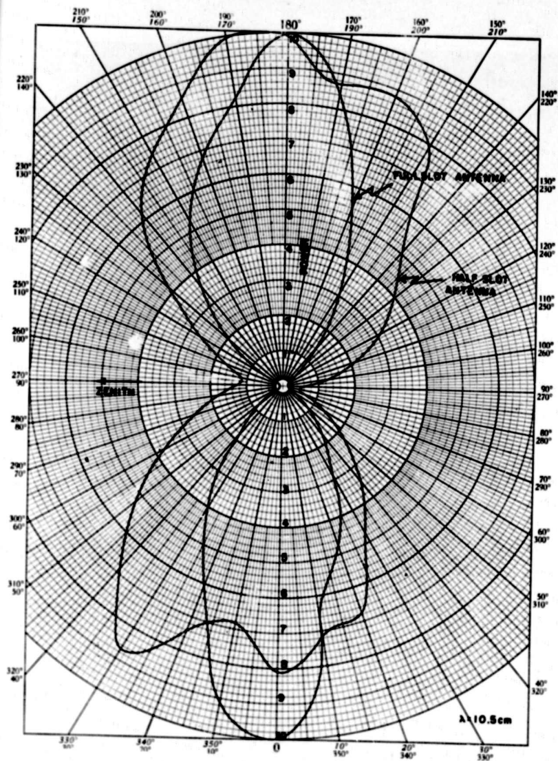
FIG. 4 - ELEVATION PATTERNS OF SLOTTED ANTENNAS
