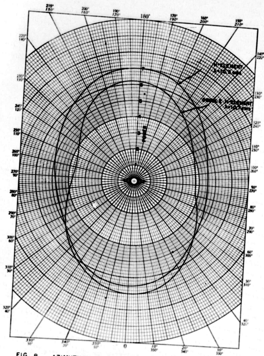
FIG. 8 AZIMUTHAL PATTERNS OF H-ELEMENT ANTENNAS
