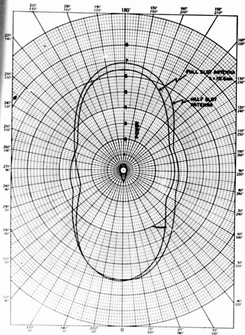
FIG. 3 — AZIMUTH PATTERNS OF SLOTTED BEACON ANTENNAS
