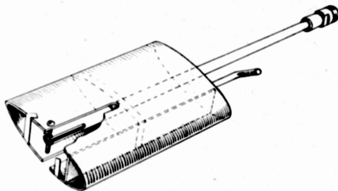
FIG. 2 HALF-SLOT ANTENNA S-BAND
