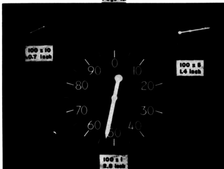
Figure 2. Dial designs and sizes used in the experiment. Each of the three designs shown were used in all three sizes indicated. The dimensions, in inches, given below are for the 2.8 inch dial. For the 1.4 inch and 0.7 inch dials all dimensions are respectively one half and one fourth as large.
