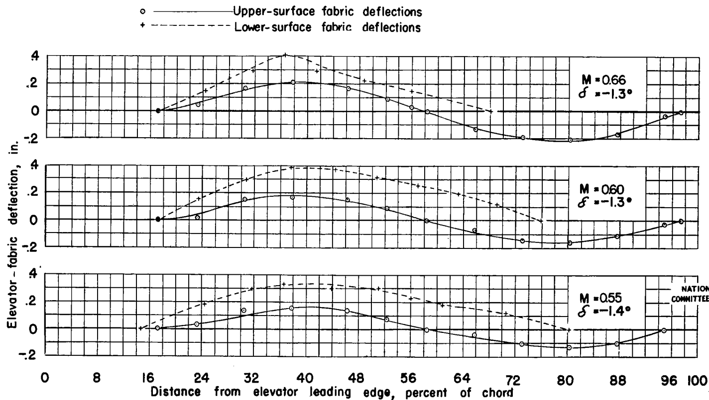
Figure 11 — Concluded.
