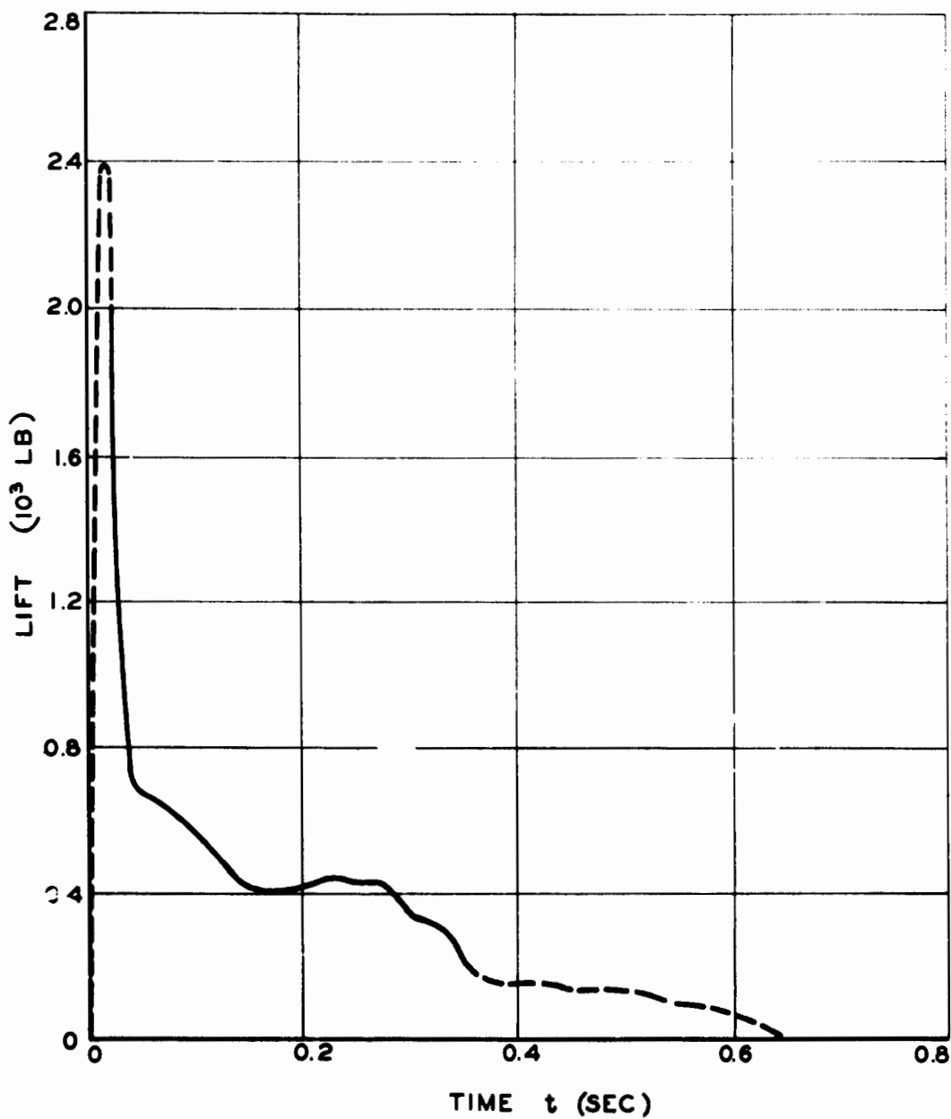
Fig. 5.25 Average Variation of Lift with Time Obtained from Differential-pressure Measurements for Rigid Wing 102. The angle of incidence was 9°, and the range was 4,020 ft, Engel.
