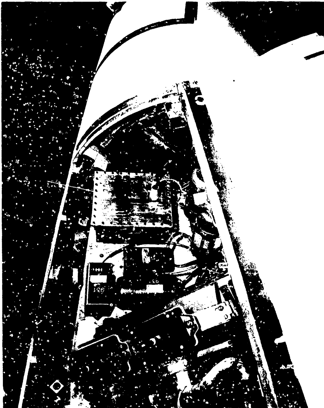
Fig. 14 - Emergency Cutoff Receiver Installed in the V-2 Control Chamber
