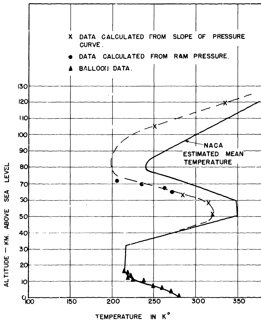
Fig. 5 - Temperature vs. Altitude, 7 March 1947
