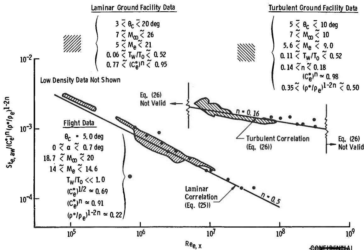
Figure 18. Local heating rate comparison between ground test facility and full-scale flight for laminar and fully turbulent boundary-layer conditions.
