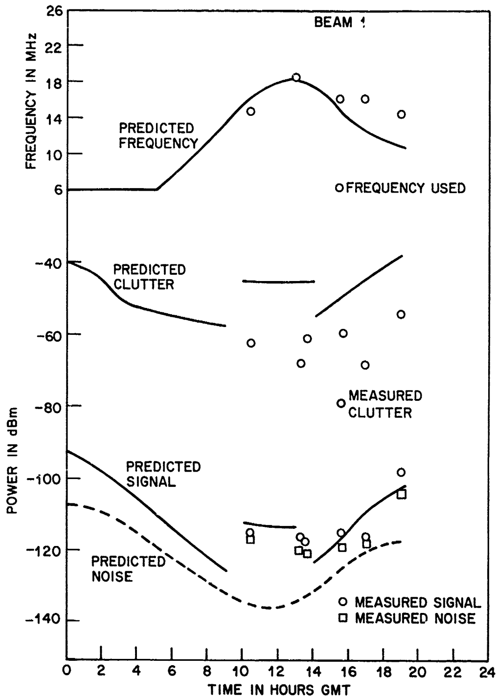
(S) Fig. 18 - Comparison between predictions and measurements
