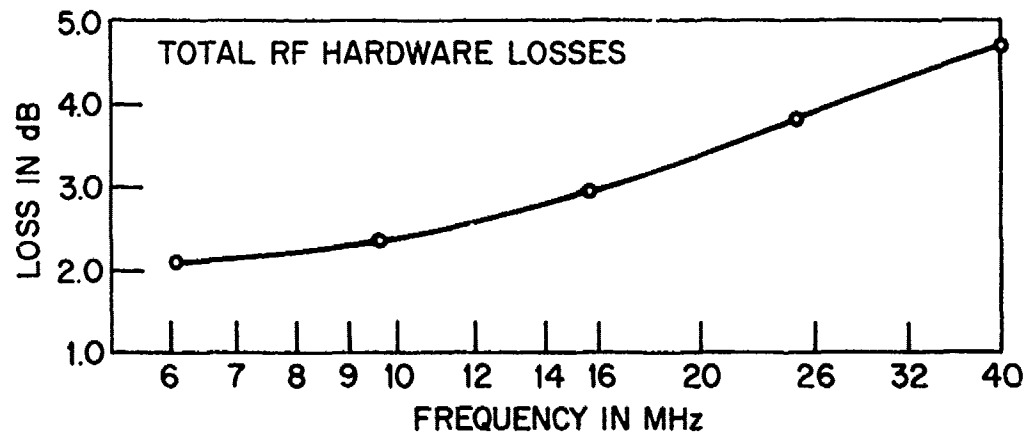
(S) Fig. 6 - RF Hardware losses
