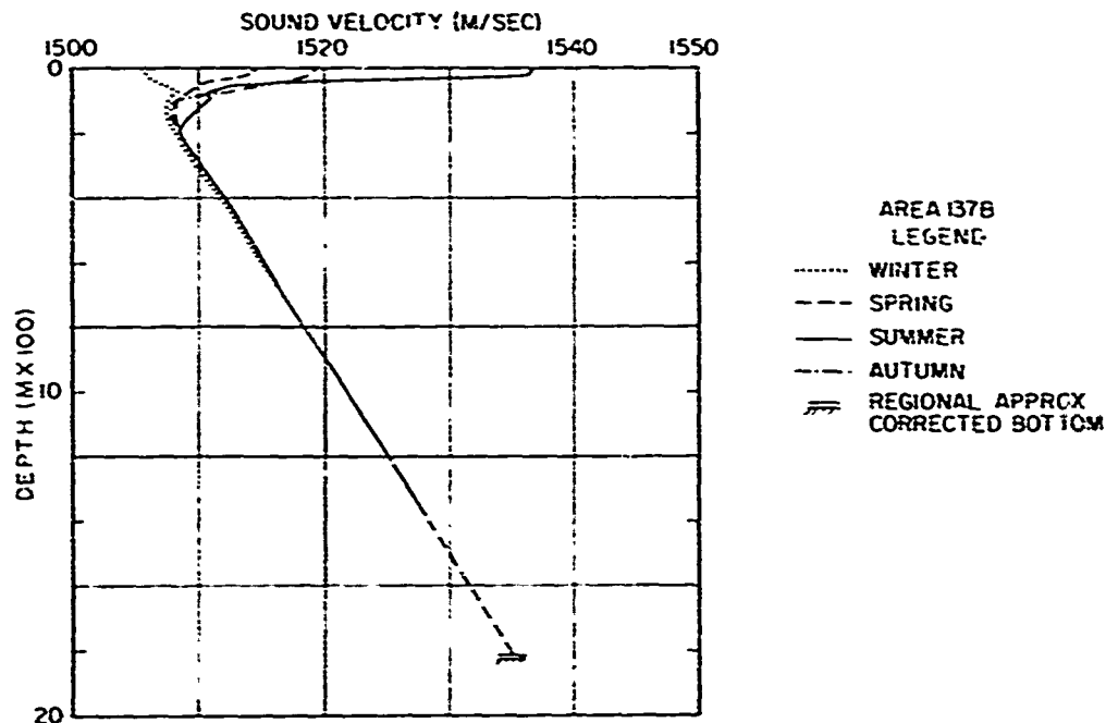
Figure A-2. Representative Seasonal Sound Velocity Profiles for Region 137B
