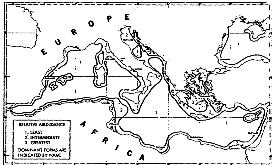
Figure 2.4.2-4. Distribution of Sound Producing Fish, Autumn
