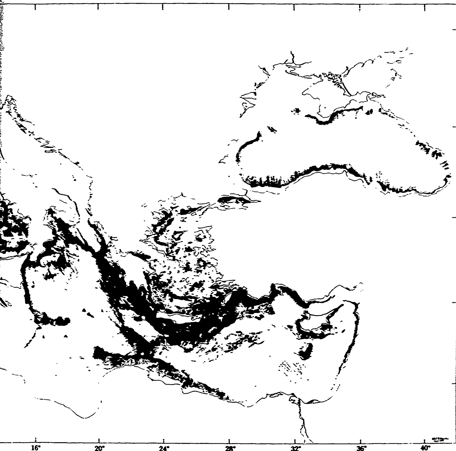
Physiographic Diagram of the Mediterranean Sea
