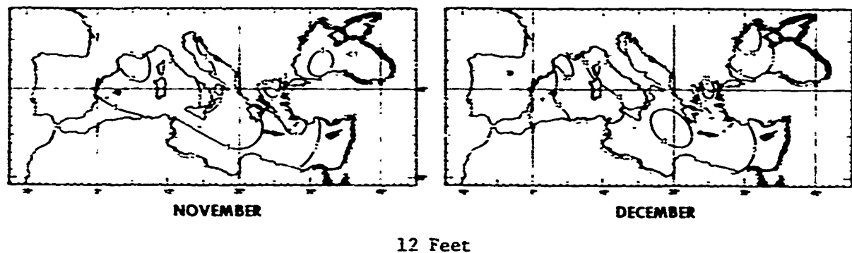
Figure 2.1.6-6. Cumulative Percentage Frequency of Occurrence of Sea Heights Exceeding 5, 8 and 12 feet for the Months of November and December
