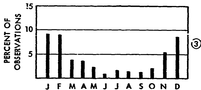
Figure 2.1.4-5. Percentage of Climatological Observations by the Month Which Include Precipitation for the Indicated Basins (Narrow Bars Correspond to Liquid, Wide Bars to Frozen Precipitation)
