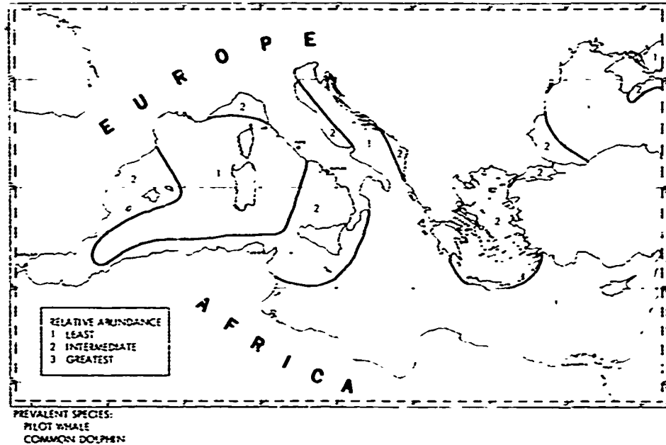
Figure 2.4.1-1. Distribution of Marine Mammals, Winter
