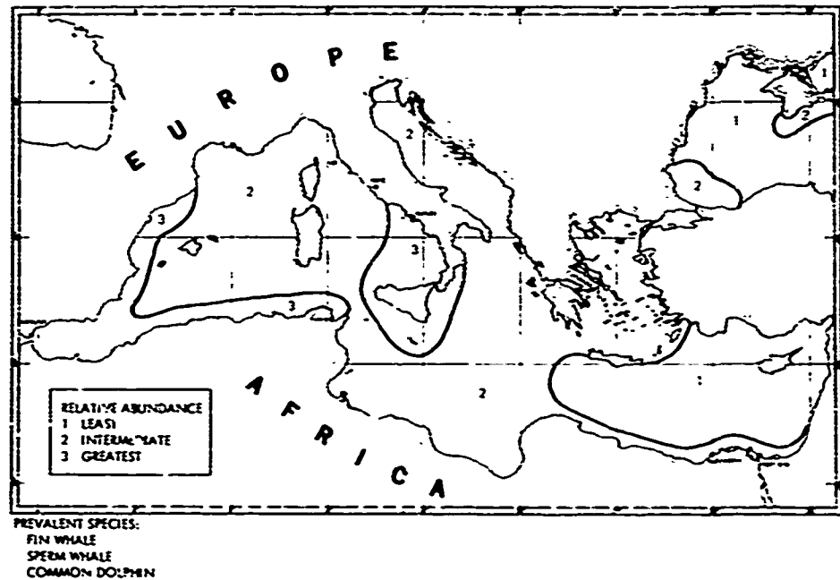
Figure 2.4.1-2. Distribution of Marine Mammals, Spring
