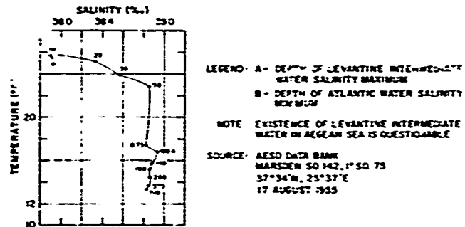
Figure 2.2.i-11. Winter and Summer Temperature, Salinity, Sound Velocity Profiles and Temperature-Salinity Diagrams for Aegean Sea
