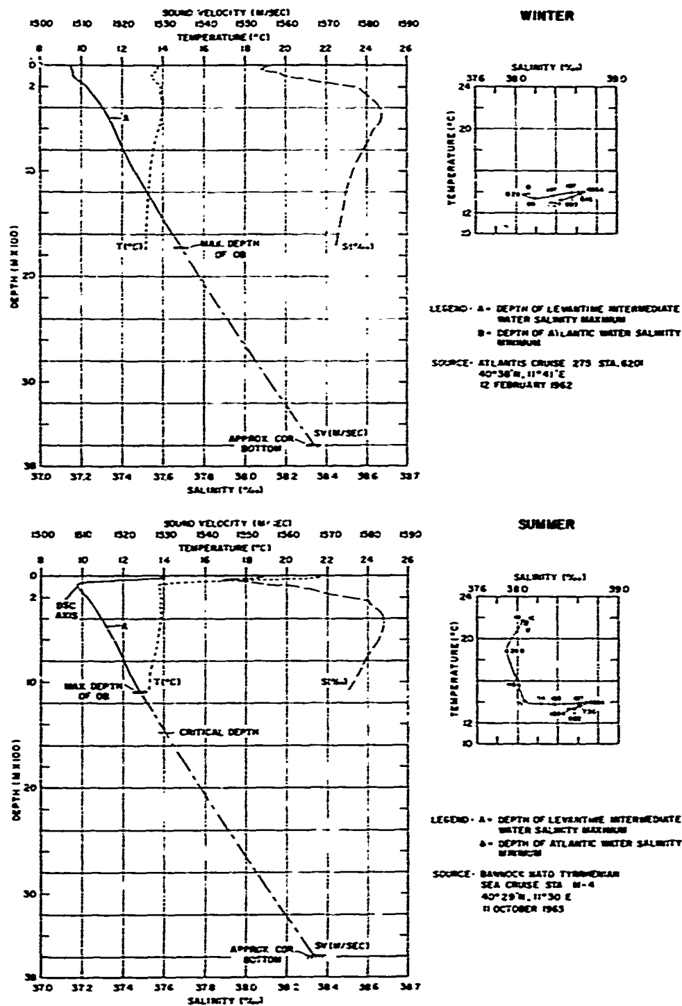
Figure 2.2.1-6. Winter and Summer Temperature, Salinity, Sound Velocity Profiles and Temperature-Salinity Diagrams for Tyrrhenian Sea
