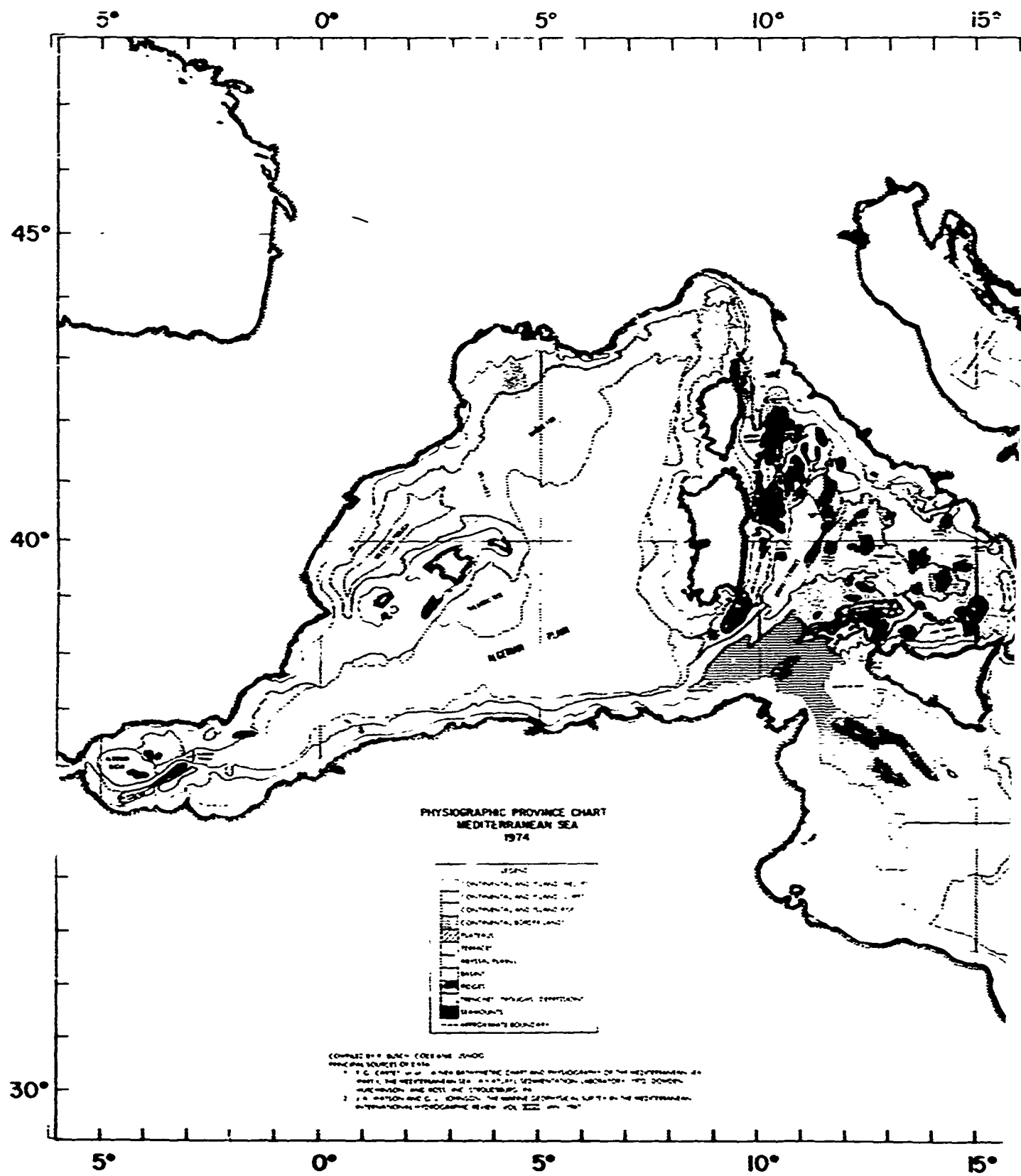
Figure 2.3.2-1. Physiographic Provi
