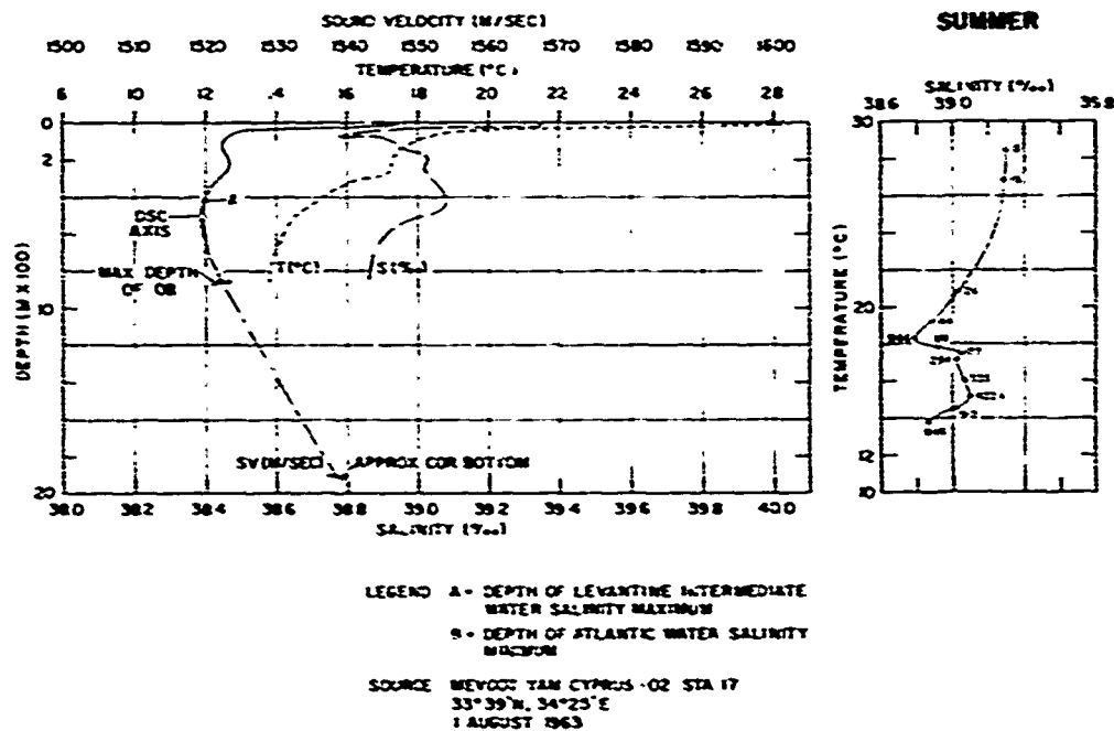
Figure 2.2.1-14. Winter and Summer Temperature, Salinity, Sound Velocity Profiles and Temperature-Salinity Diagrams for Eastern Levantine Basin
