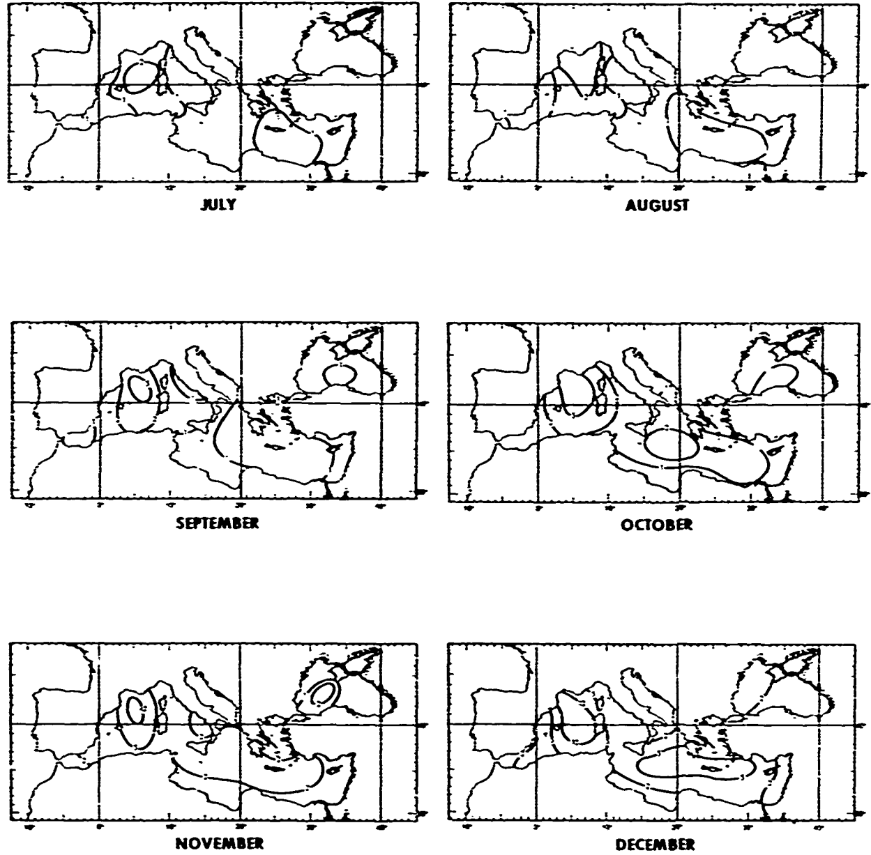
Figure 2.1.-3. Cumulative Percentage Frequency of Occurrence Swell Exceeding 12 feet for the Months July through December
