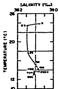
Figure 2.2.1-8. Winter and Summer Temperature, Salinity, Sound Velocity Profiles and Temperature-Salinity Diagrams for Adriatic Basin
