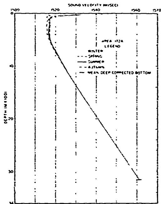
Figure A-48. Representative Seasonal Sound Velocity Profiles for Region 172A
