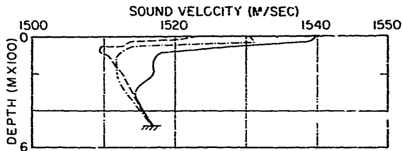
Figure A-23. Representative Seasonal Sound Velocity Profiles for Region 157A
