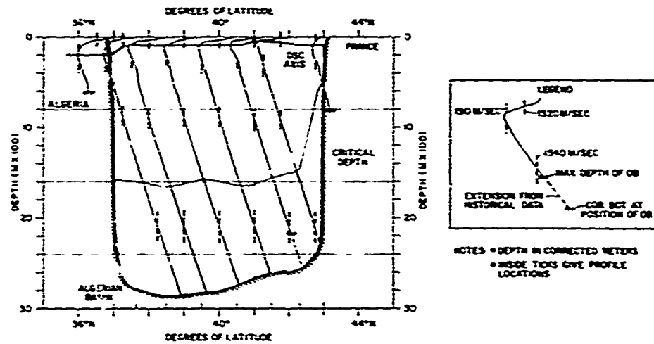
Figure 3.1.2-5. South-North Sound Velocity Cross-section in Algerian Basin (6°E) for Summer, July-Sept. or
