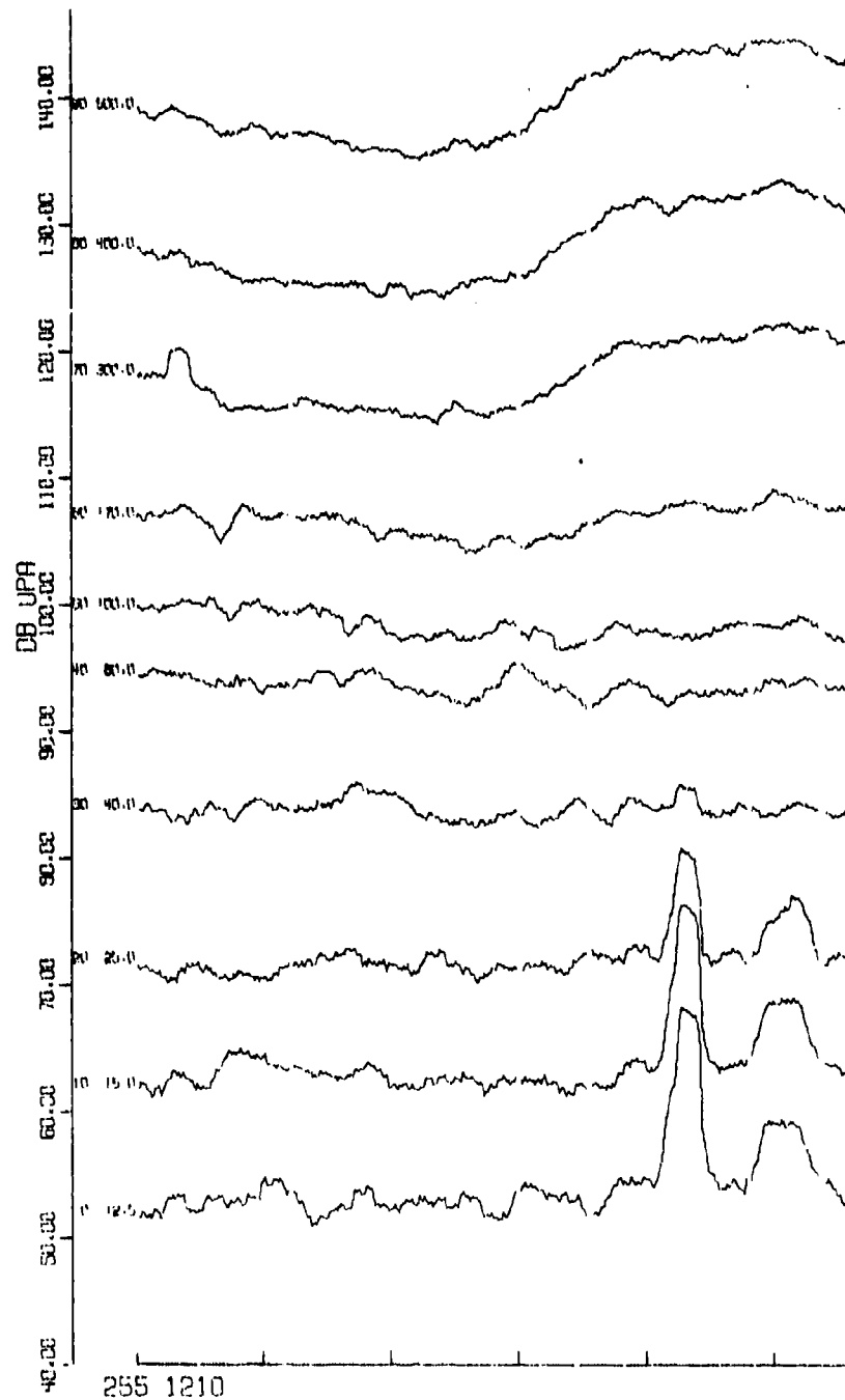
Figure 4(C). Ambient noise levels as a function of time for the indicated frequencies, using a 10 minute integration time, for Julian Day 255 from 1210 to 1755 hours. (The number to the far left of each curve indicates the number of dB the curve is displaced relative to the ordinate scale.) (U)
