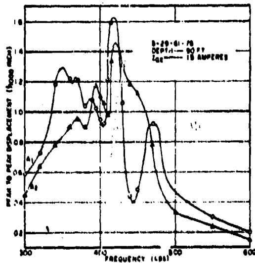
Figure 18 - Transducer displacement
