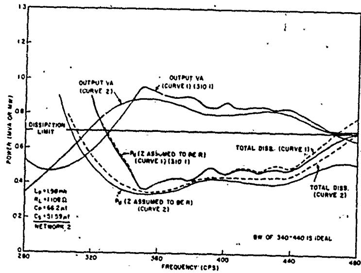
Fig. 21 - Amplifier Operating Characteristics Curves 1 and 2 at 310:1.
