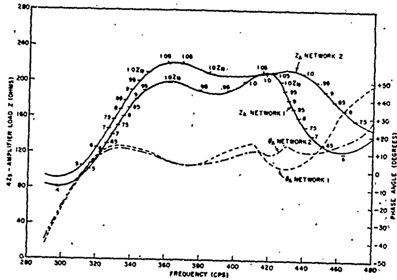
Fig. 22 - Impedance Diagram for Transducer Curve 1, Line Match of 279:1, Networks 1 and 2
