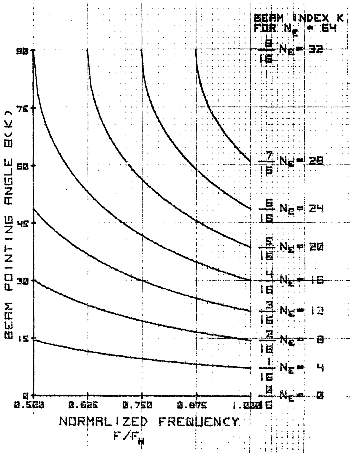
Figure 4-2. Beam Steering
