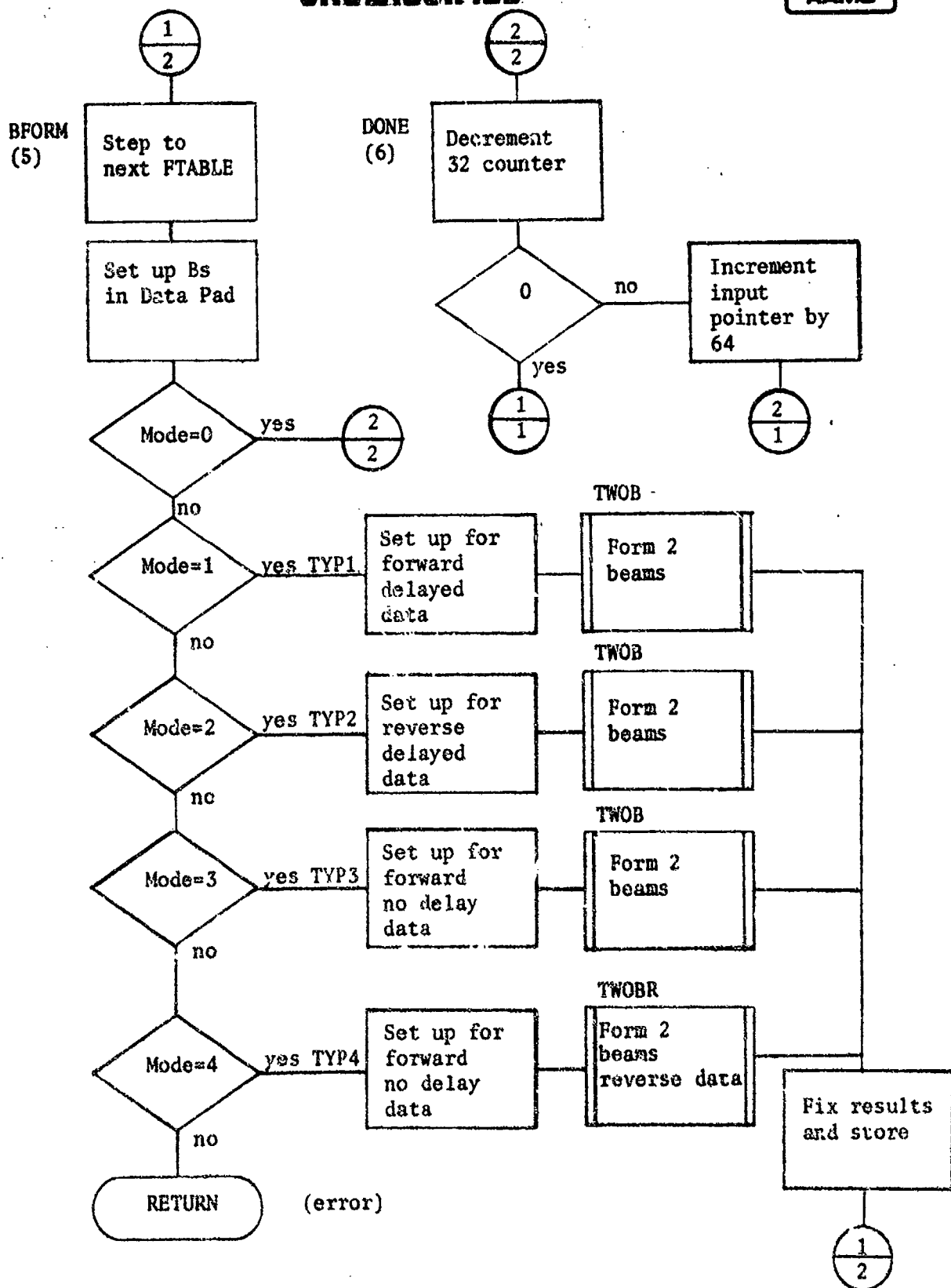
Figure A-2. TBDF (Sheet 2 of 2)
