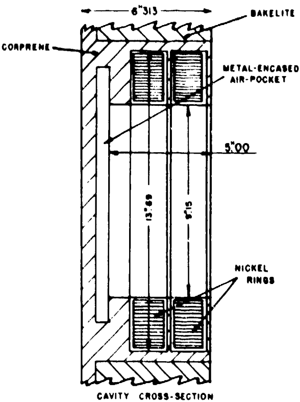
Fig. 3 - Cross section of typical cavity element of magnetostrictive transducer XM-1A
