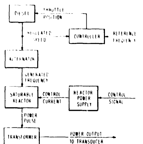
Fig. 18 - Block diagram control circuit of diesel-alternator
