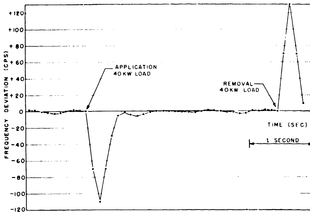
Fig. 20 - Frequency-control characteristics of diesel-alternator
