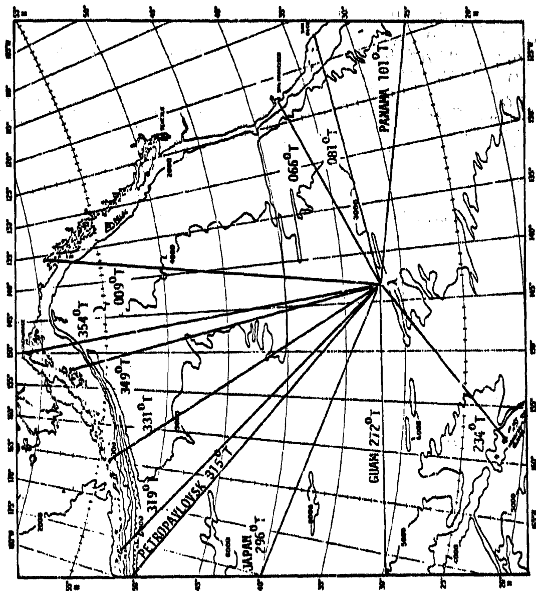
Figure 13. (C) Bearings from CHURCH OPAL Site 2g to various locations in the North Pacific Ocean Basin. (U)
