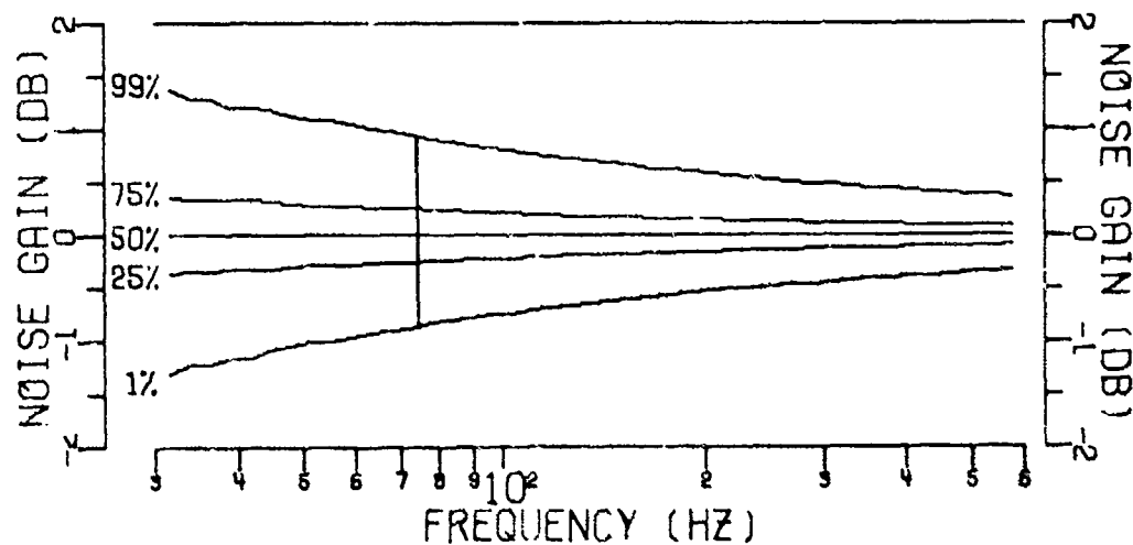
FIGURE I-19 EXPECTED DISTRIBUTION OF AMBIENT SOUND FIELD MEASUREMENTS THROUGH 1/10-OCTAVE BANDS
