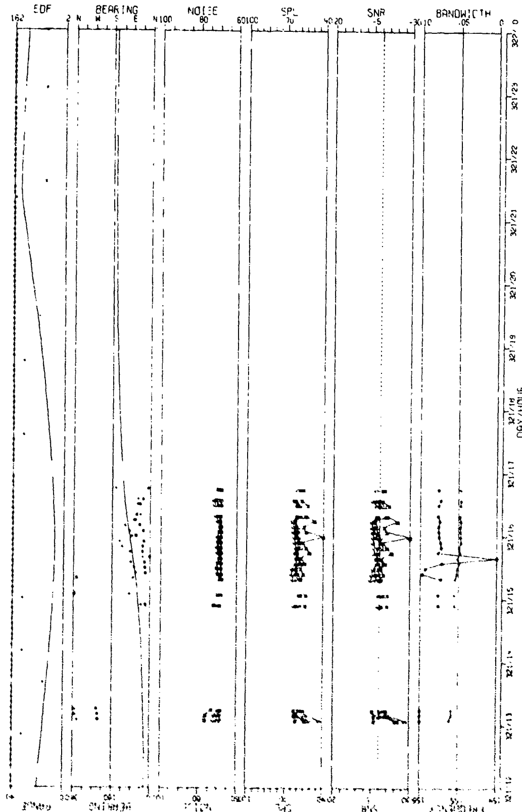
FIGURE 11-21 155HZ LINE HISTORY AS OBSERVED VIA THE MAX GAIN LIMACONS SENSOR DURING THE 17 NOV FIELD EVENT WITH STANDARD RESOLUTION 101
