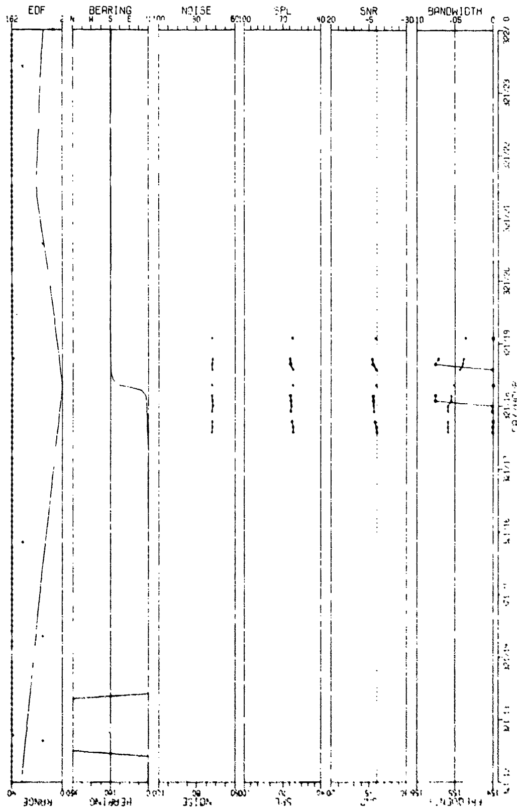
FIGURE 11-103 M-100 155mm LINE HISTORY AS OBSERVED VIA THE OMNIDIRECTIONAL SENSOR AT SITE A3 DURING THE 17 NOV FIELD EVENT WITH STANDARD RESOLUTION (U)
