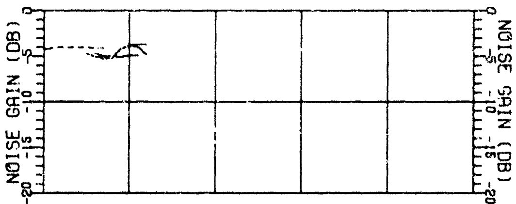
FIGURE II-175 MSS-FVT NEAR BOTTOM SINGLE CARDIOIDS SENSOR ARRAY GAIN RESULTS FOR 305HZ AT 136DB (U)
