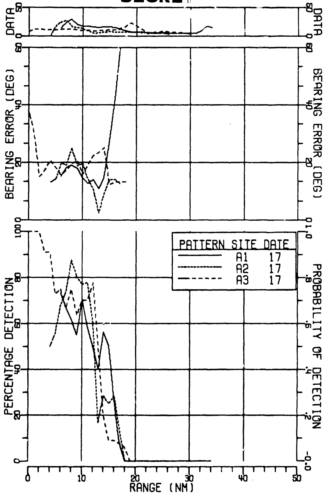
FIGURE II-193 MSS-FVT NEAR BOTTOM MAX GAIN LIMAcons SENSOR DETECTION RESULTS FOR 305HZ AT 136DB (U)
