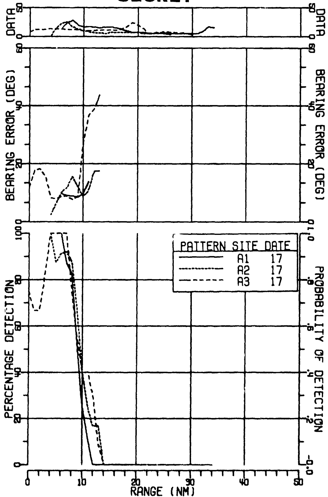
FIGURE II-195 MSS-FVT NEAR BOTTOM DIFFERENCED CAROIDIDS SENSOR DETECTION RESULTS FOR 305HZ AT 136DB (U)
