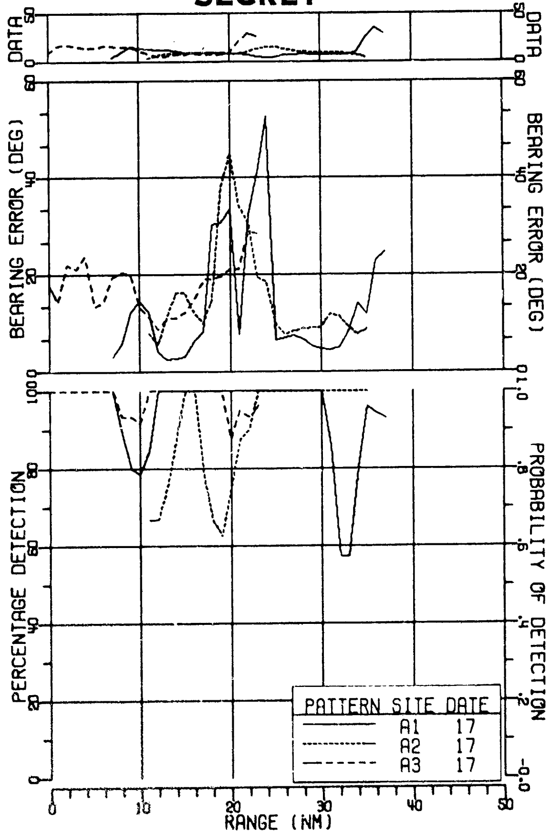
FIGURE II-217 MSS-FVT NEAR BOTTOM SINGLE CARDIOIDS SENSOR DETECTION RESULTS FOR 170HZ AT 156DB (U)
