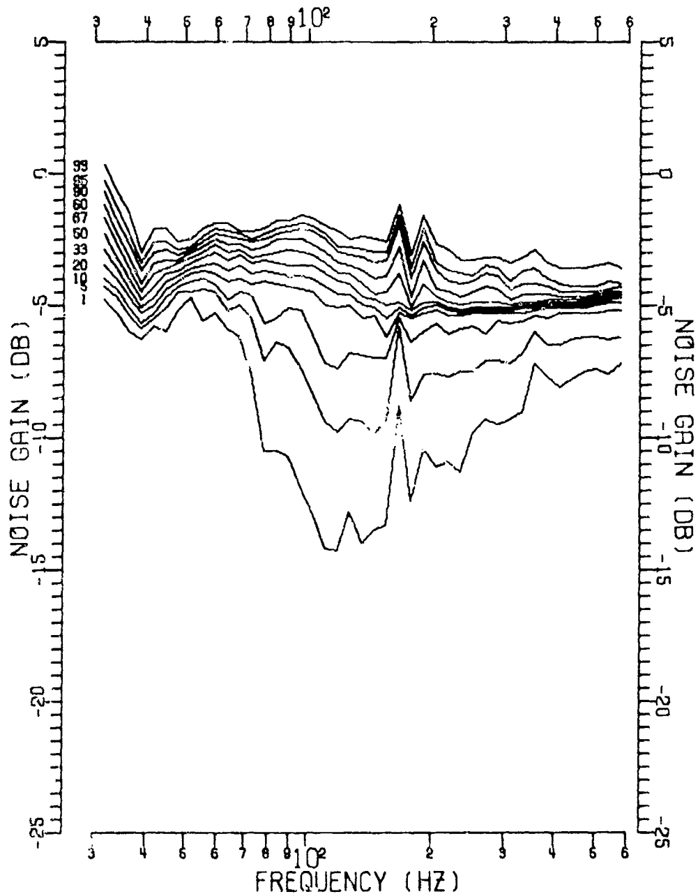
FIGURE II-334 MSS-FVT PHASE II SITE A1 EAST CARDIOID PERCENTILE LEVELS OF 1 MIN AVERAGED NOISE GAINS THROUGH 1/10-OCTAVE BANDS DURING THE 17 NOV FIELD EVENT (U)
