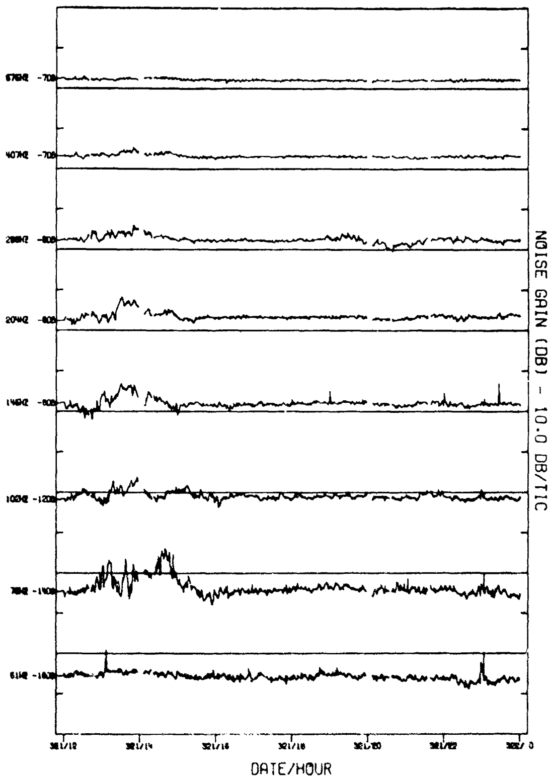
FIGURE 11-318 MSS-FVT PHASE II SITE A3 DIFFERENCED NORTH CARDIOID TIME SERIES OF 1 MIN INTENSITY-AVERAGED NOISE GAINS THROUGH 1/10-OCTAVE BANDS DURING THE 17 NOV FIELD EVENT (U)
