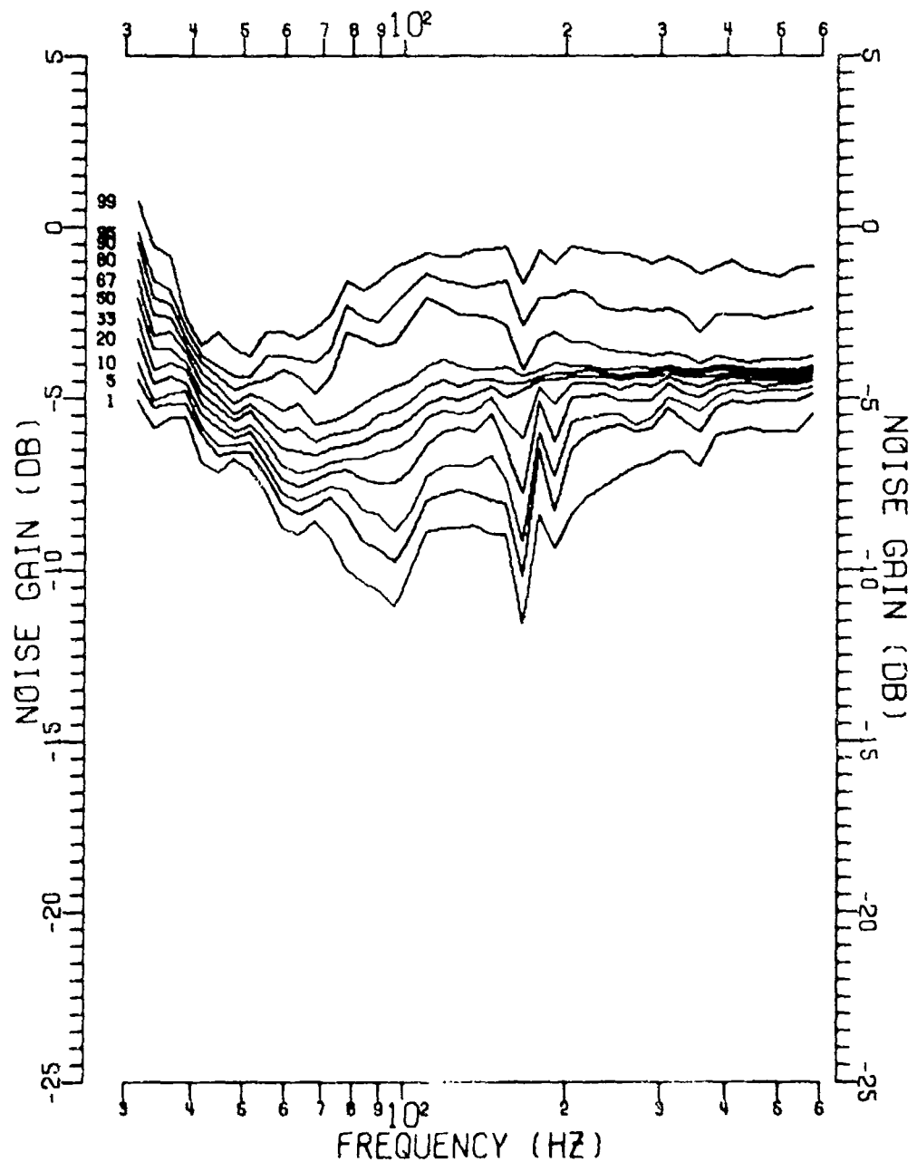
FIGURE II-340 MSS-FVT PHASE II SITE A1 WEST CARDIOID PERCENTILE LEVELS OF 1 MIN AVERAGED NOISE GAINS THROUGH 1/10-OCTAVE BANDS DURING THE 17 NOV FIELD EVENT (U)
