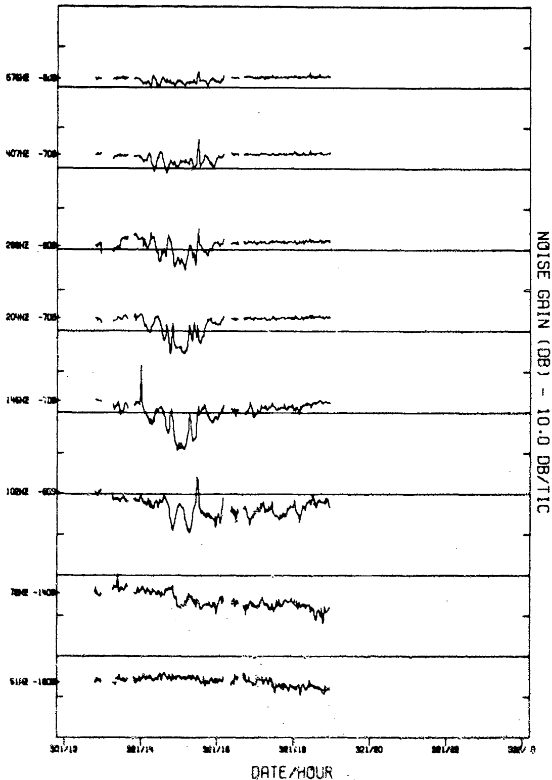
FIGURE 11-323 MSS-FVT PHASE II SITE A2 DIFFERENCED SOUTH CARDIOID TIME SERIES OF 1 MIN INTENSITY-AVERAGED NOISE GAINS THROUGH 1/10-OCTAVE BANDS DURING THE 17 NOV FIELD EVENT (U)
