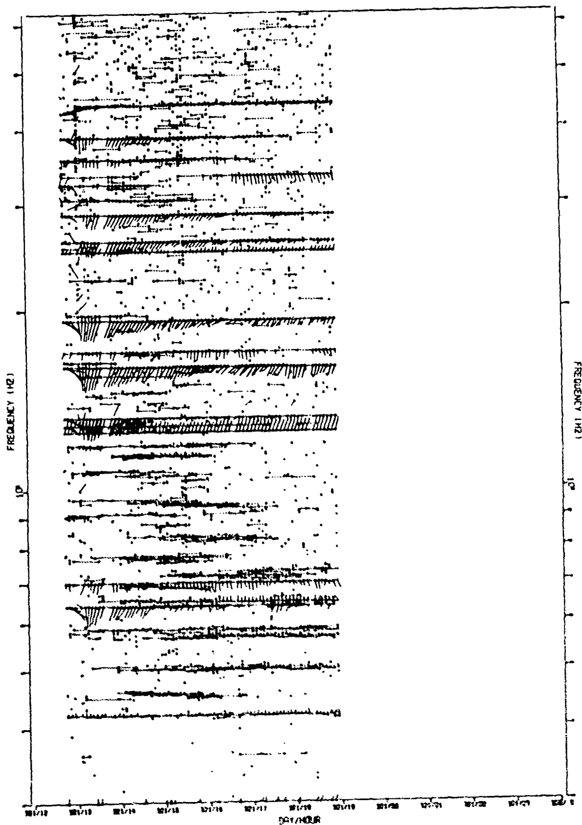
FIGURE 11-10 MKS-FVT DETECTION OVERVIEW DURING THE 17 NOV FIELD EVENT AT SITE R2 OBTAINED VIA THE DIFFERENTIAL CAPACITIVE SENSOR WITH STANDARD SIGNALING
