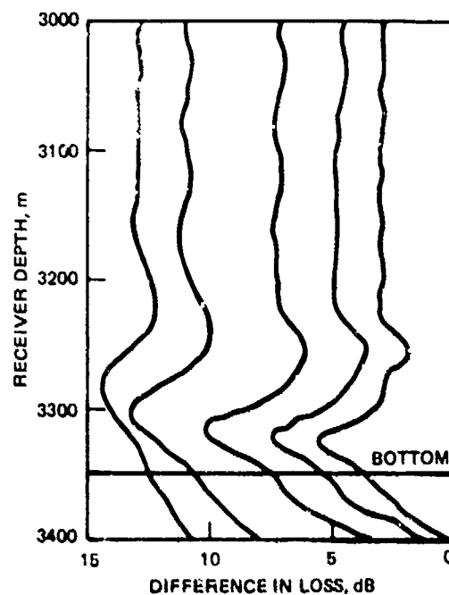
(U) Figure 31. Differences in propagation loss between the 18- and 100-m source depths of the two previous figures.
