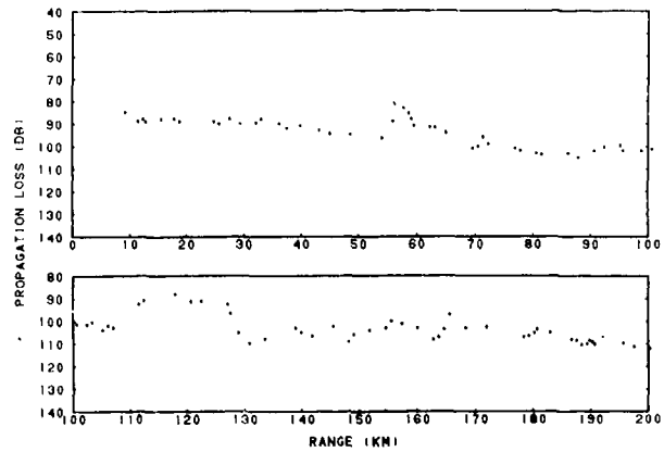
UNCLASSIFIED (U) Figure 1. PARKA Data: Source Depth-50 ft, Receiver-Depth 300 ft, Frequency-400 Hz
