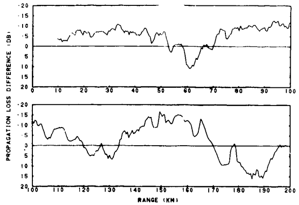
UNCLASSIFIED (U) Figure 4. Smoothed RAYMODE X (Coherent): Source Depth-50 ft, Receiver Depth-300 ft, Frequency-400 Hz Subtracted from Experimental Data, Source Depth-50 ft, Receiver Depth-300 ft, Frequency-400 Hz
