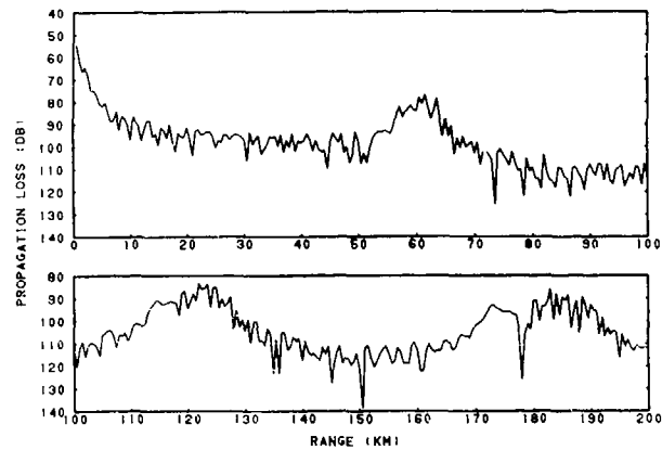
UNCLASSIFIED (U) Figure 2. RAYMODE X (Coherent): Source Depth-50 ft, Receiver Depth-300 ft, Frequency-400 Hz
