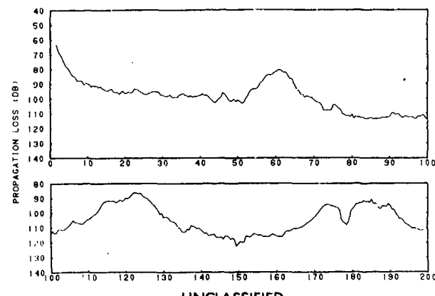
UNCLASSIFIED (U) Figure 3. RAYMODE X (Coherent): Source Depth-50 ft, Receiver Depth 300 ft, Frequency-400 Hz Sliding Averages of 5 Points (2.0 km)
