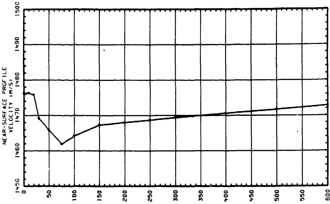
(U) Figure III-1. Gulf of Alaska Run 140 Sound Speed Profile
